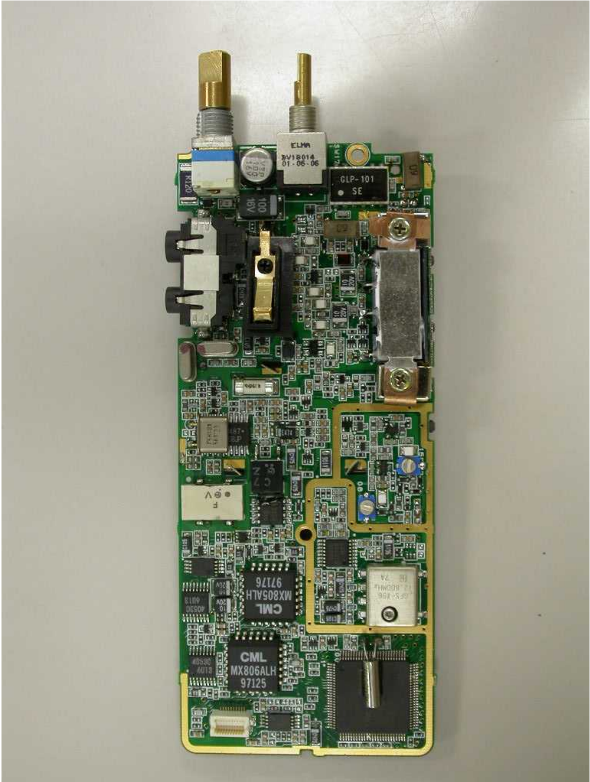
10) MAIN PCB of SC-281 A (Solder Side View)
