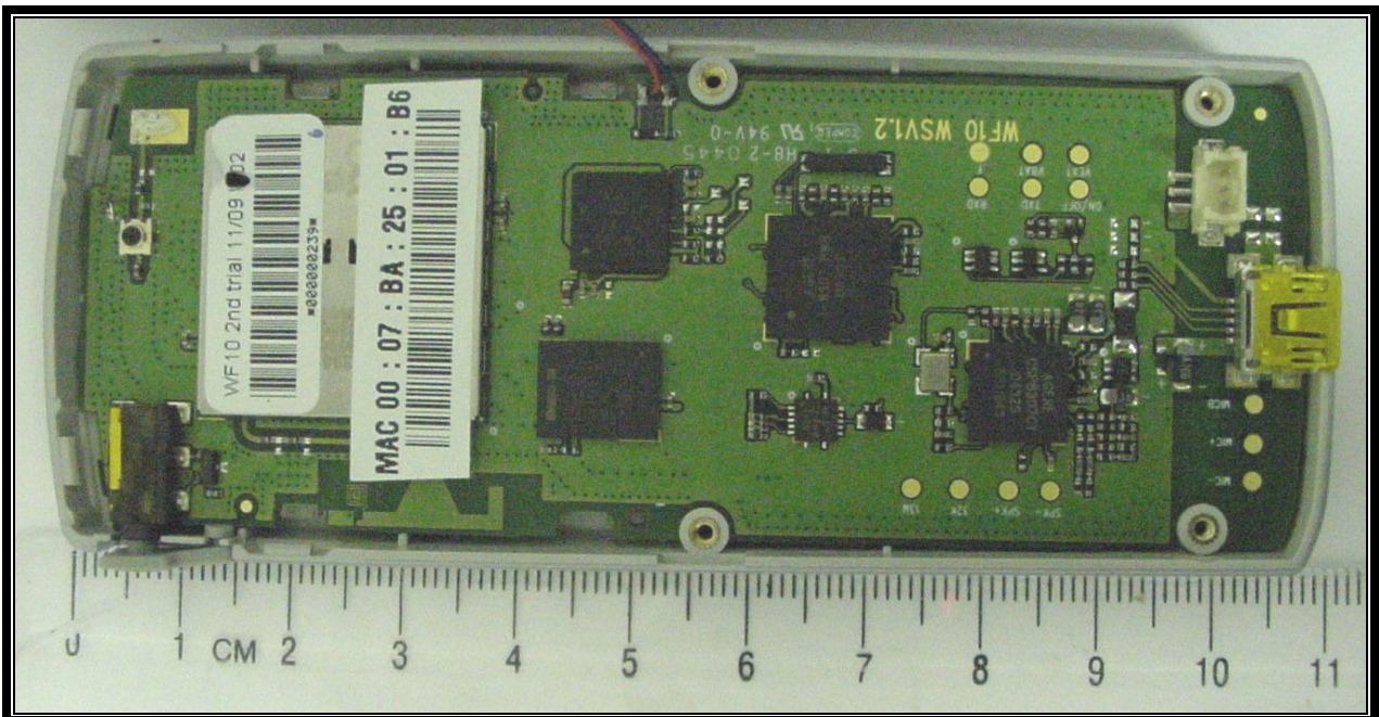
PHOTOGRAPH 12: PCB IN FRONT CASE
