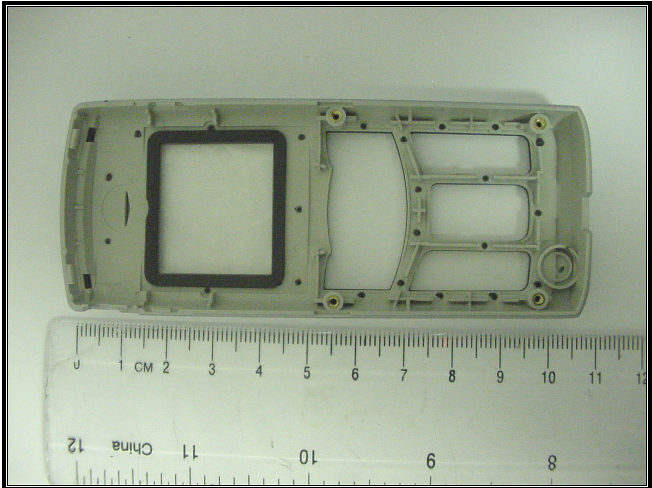
PHOTOGRAPH 10: INSIDE OF FRONT CASE
