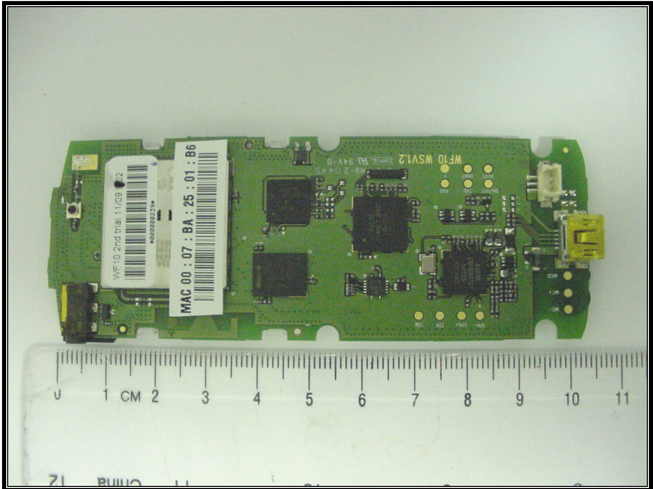
PHOTOGRAPH 14: PCB BACK
