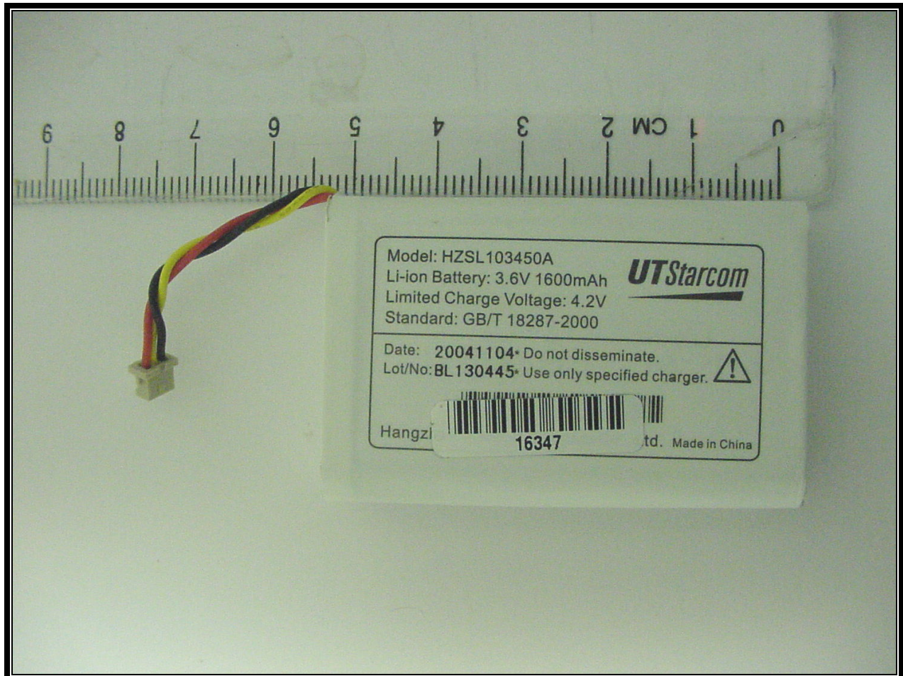
PHOTOGRAPH 9: BATTERY
