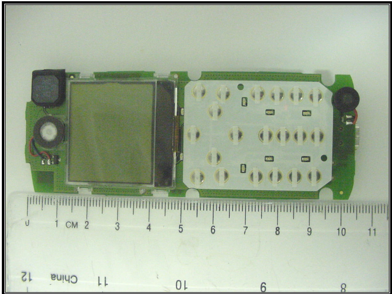
PHOTOGRAPH 13: PCB FRONT
