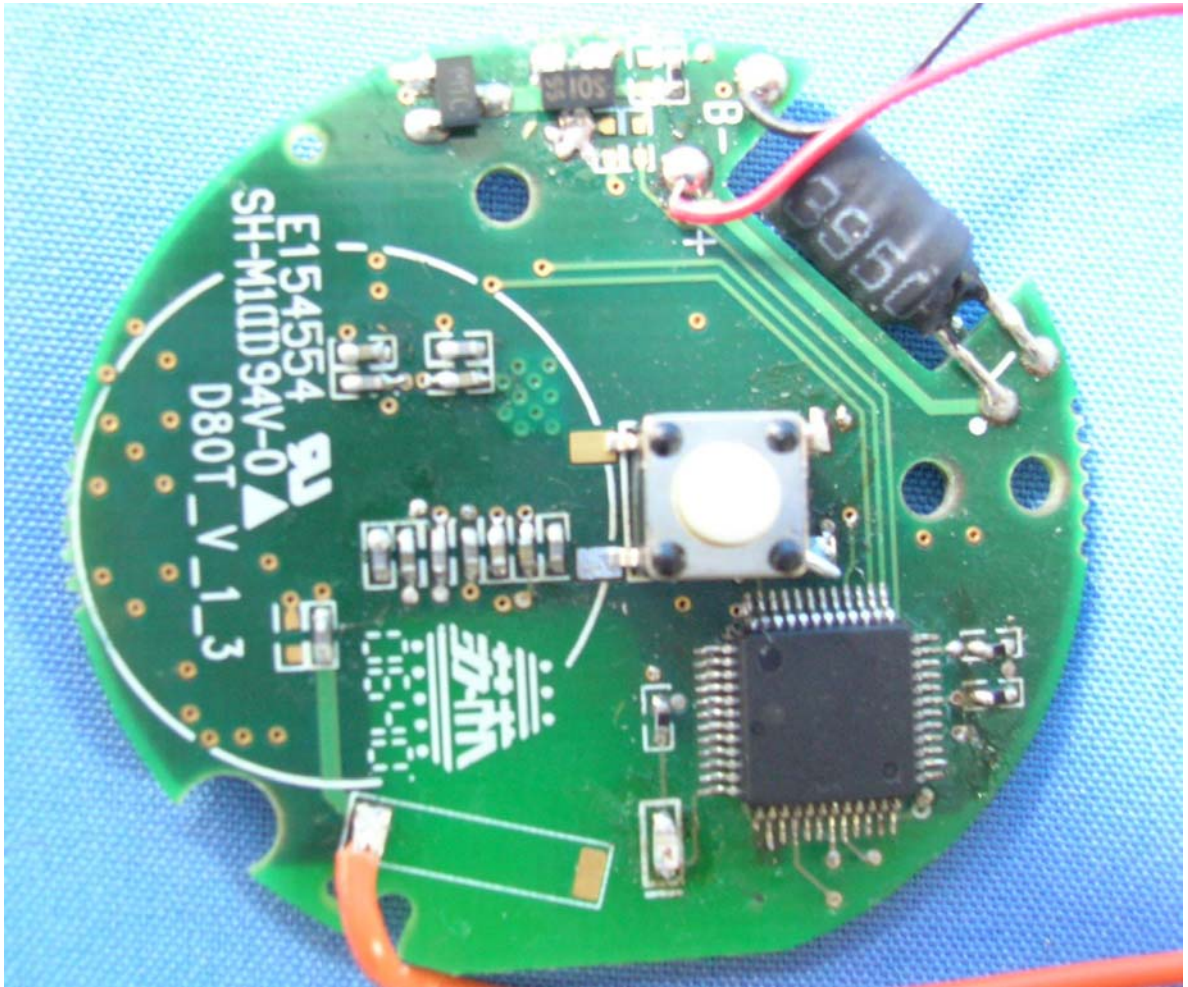
(11) EUT Photo
