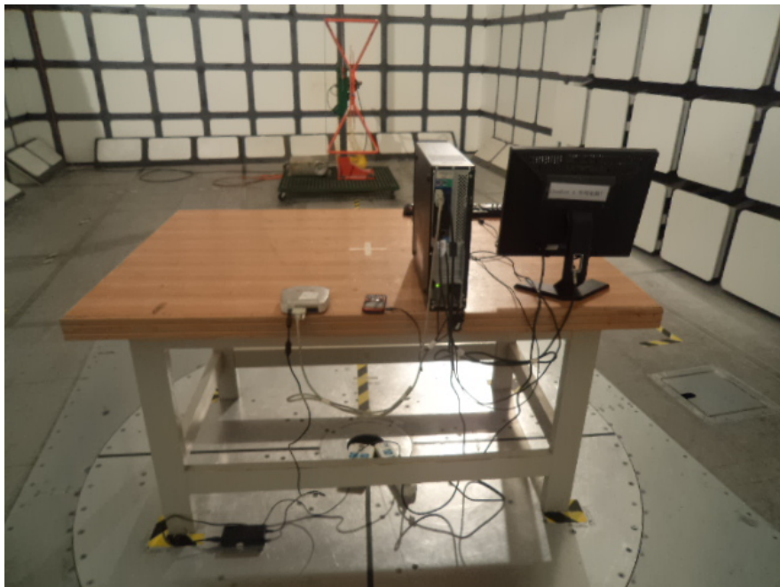
Radiated Emissions – Rear View (downloading mode, 30-1000 MHz)
