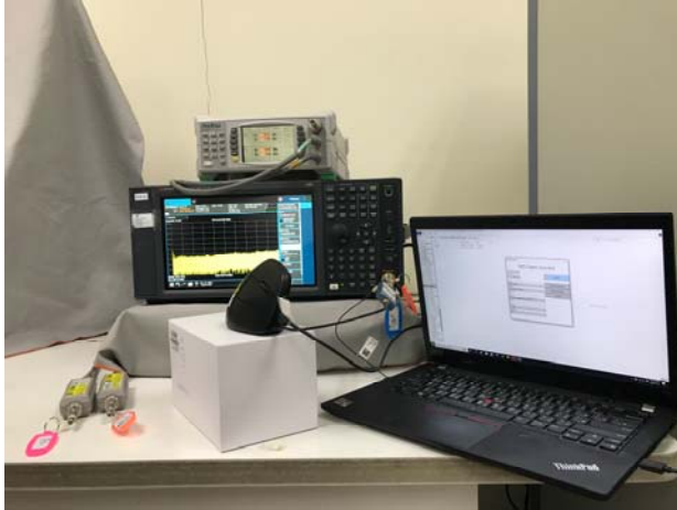
Part 15_249_SRD_Radiated_Setup
