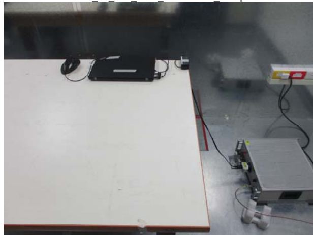
Part 15 249 SRD Conduction Setup
