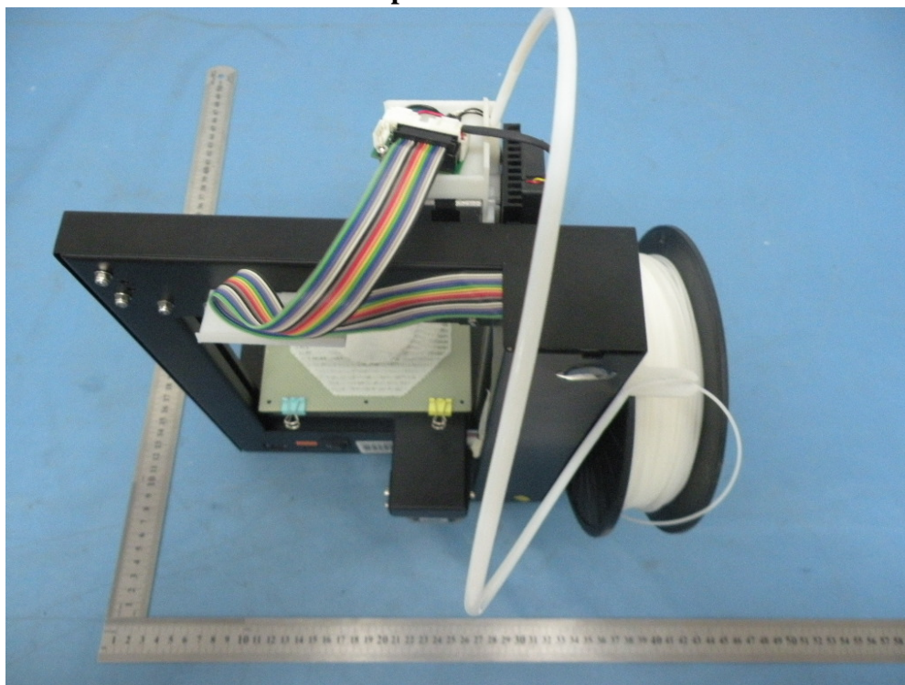
Top View
