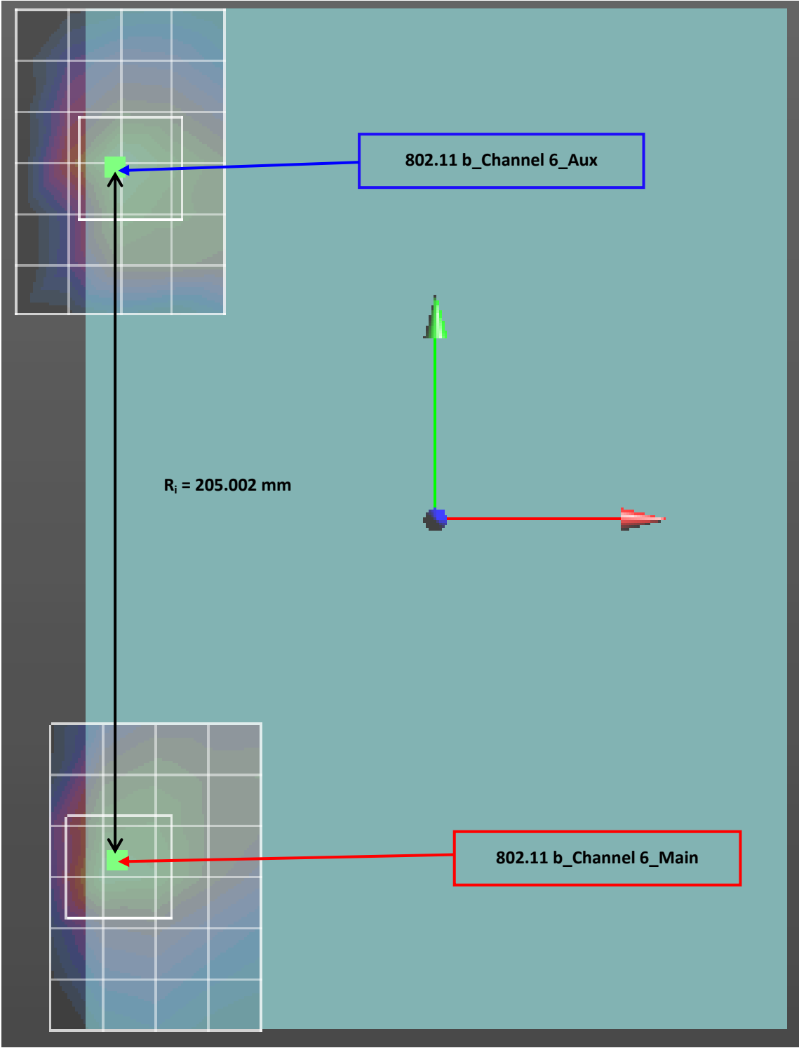
SAR Peak Location Separation Distance_2.4G_P-Sensor On
