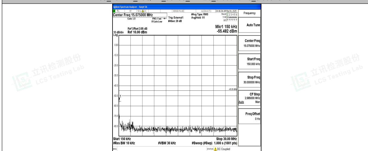
Band38_10MHz_16QAM_38200_1RB#0_0.15~30_0.15~30
