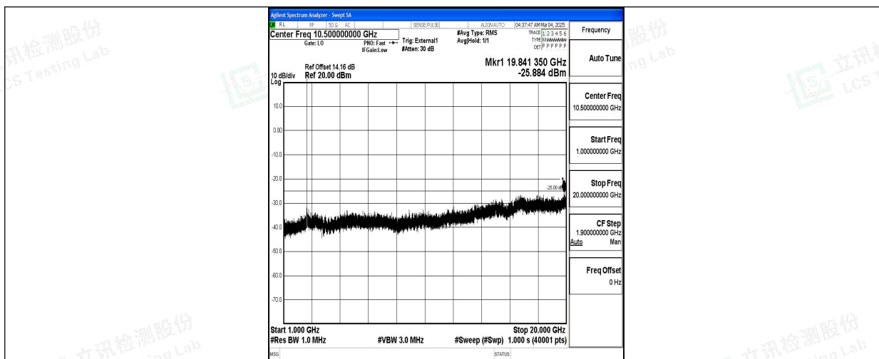
Band38_10MHz_QPSK_37800_1RB#0_1000~20000_1000~20000
