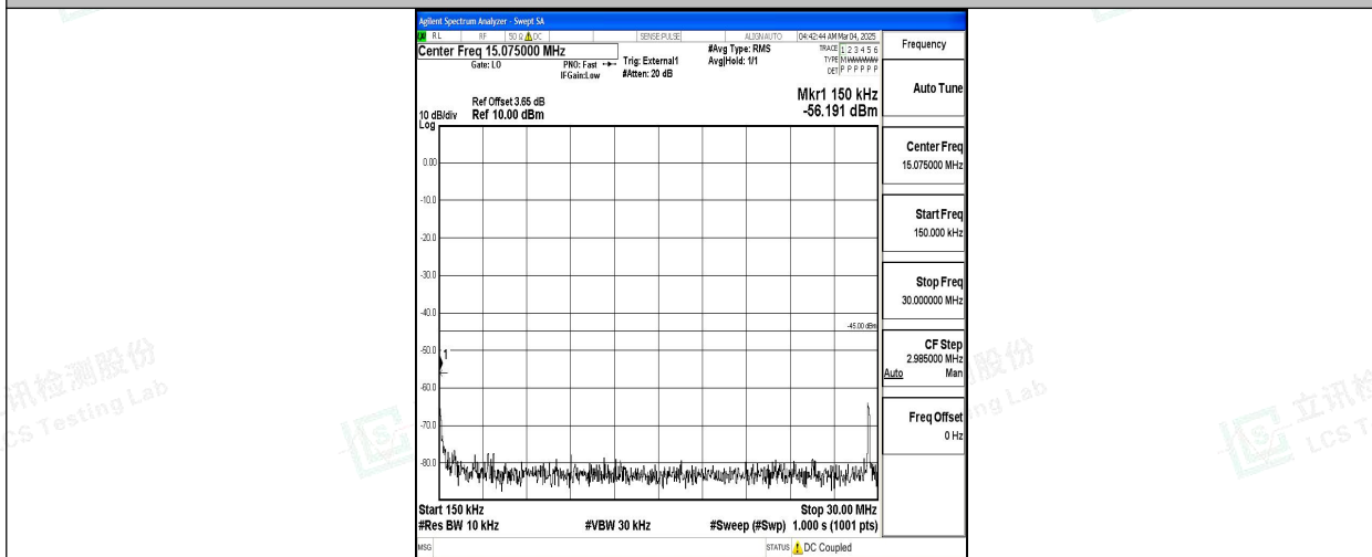
Band38_10MHz_16QAM_38000_1RB#0_0.15~30_0.15~30
