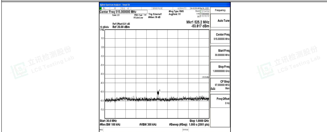
Band38_10MHz_16QAM_38000_1RB#0_30~1000_30~1000
