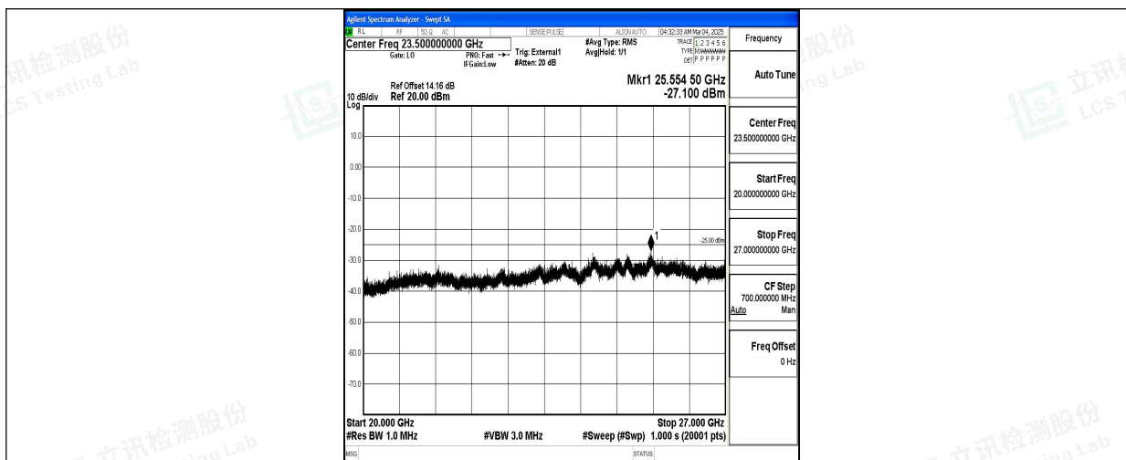
Band38_5MHz_QPSK_38225_1RB#0_20000~27000_20000~27000
