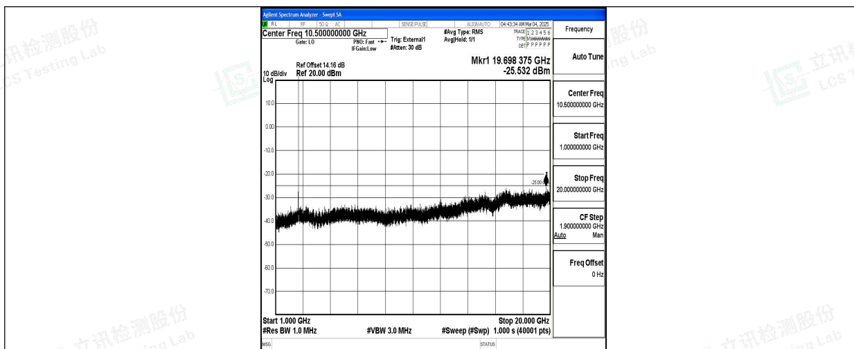
Band38_10MHz_16QAM_38000_1RB#0_1000~20000_1000~20000
