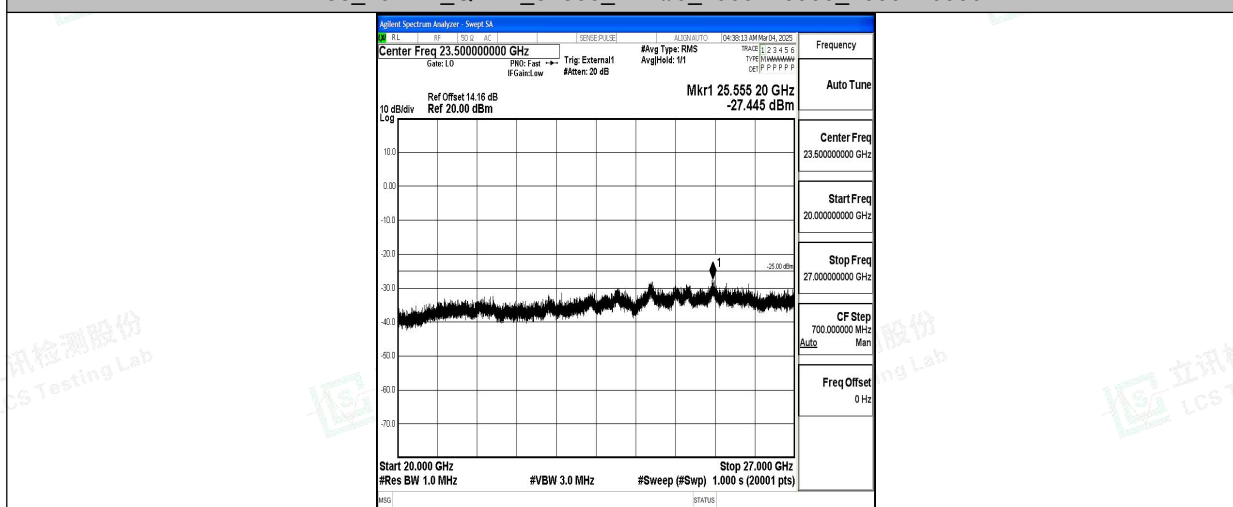
Band38_10MHz_QPSK_37800_1RB#0_20000~27000_20000~27000
