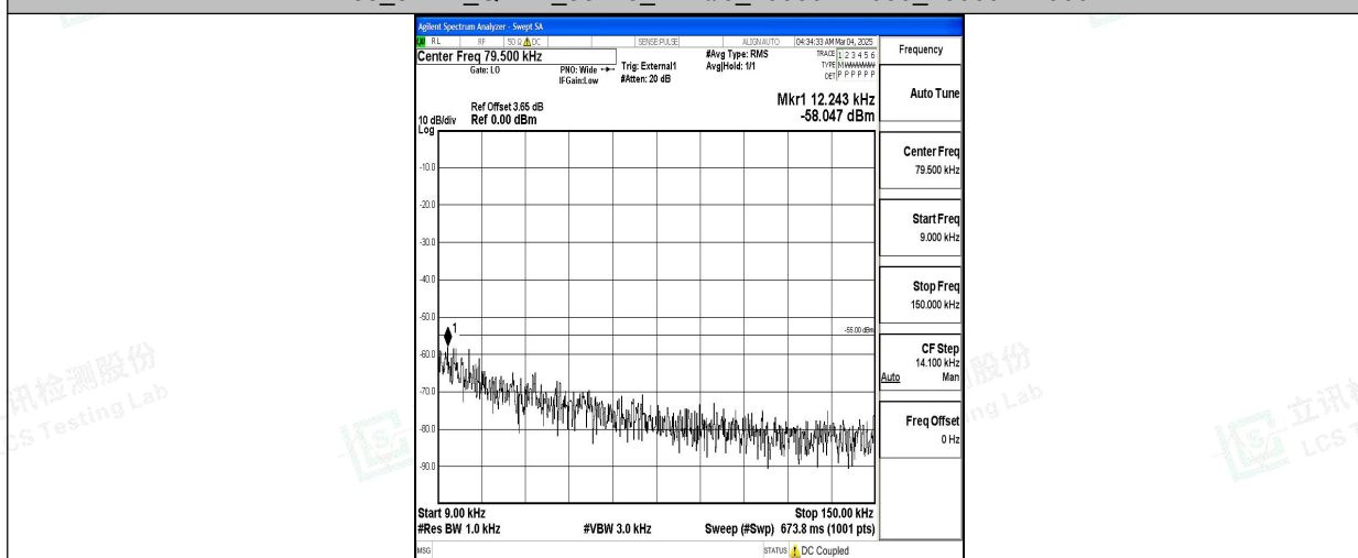
Band38_5MHz_16QAM_38225_1RB#0_0.009~0.15_0.009~0.15
