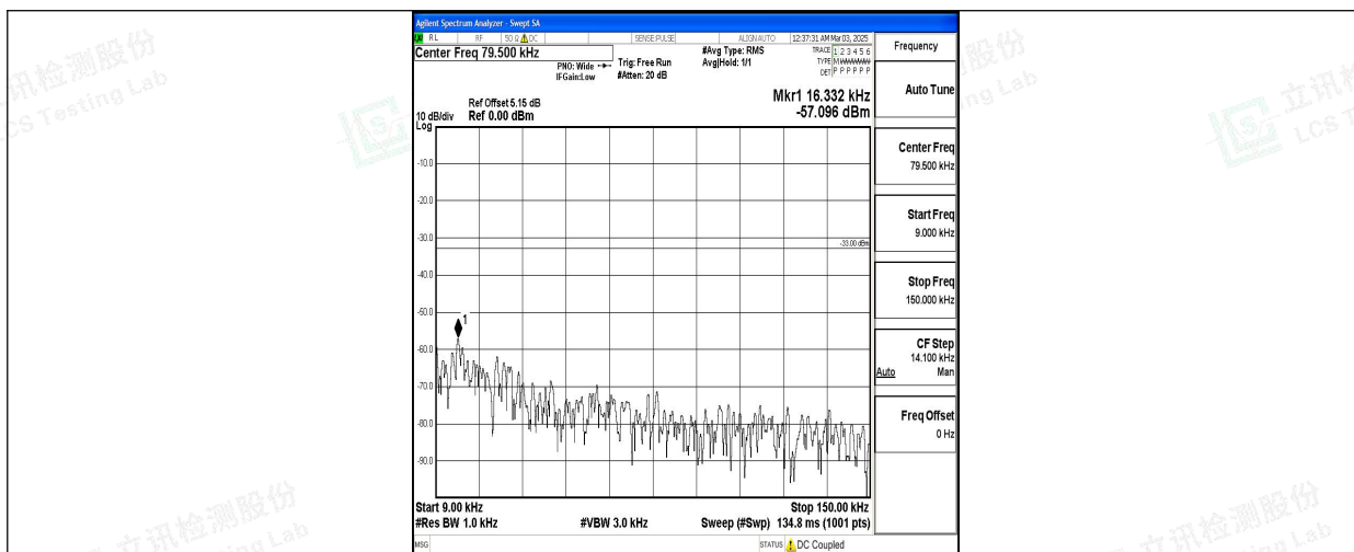
Band5_10MHz_QPSK_20450_1RB#0_0.009~0.15_0.009~0.15
