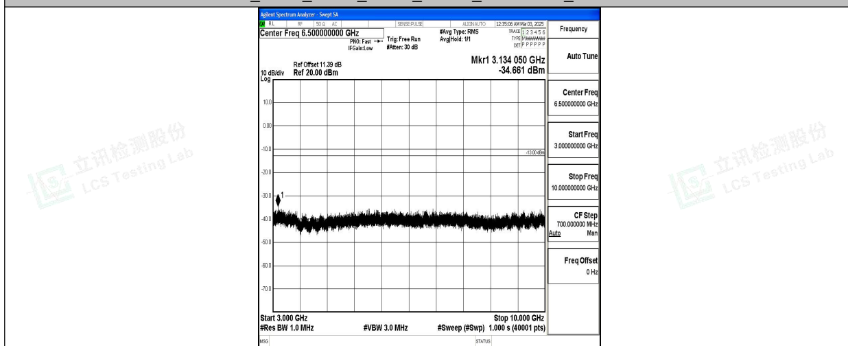
Band5_5MHz_QPSK_20525_1RB#0_3000~10000_3000~10000
