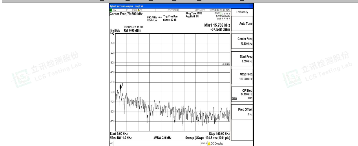
Band5_10MHz_16QAM_20450_1RB#0_0.009~0.15_0.009~0.15
