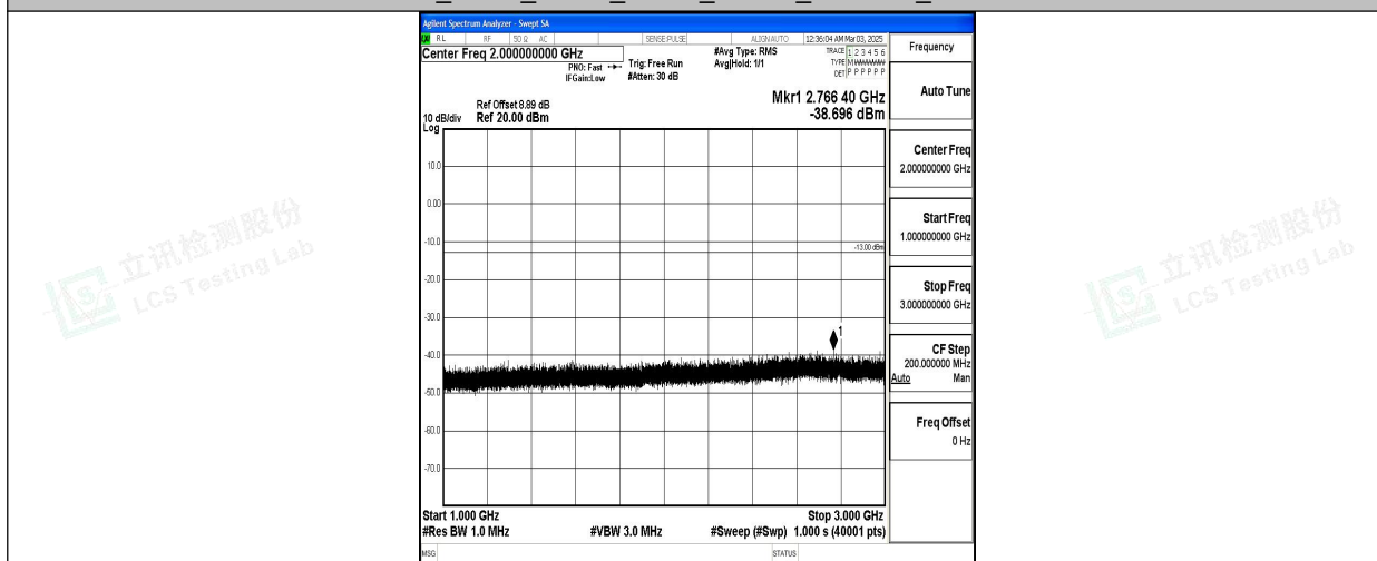
Band5_5MHz_QPSK_20625_1RB#0_1000~3000_1000~3000
