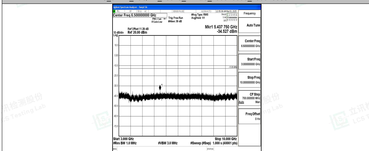
Band5_5MHz_16QAM_20525_1RB#0_3000~10000_3000~10000
