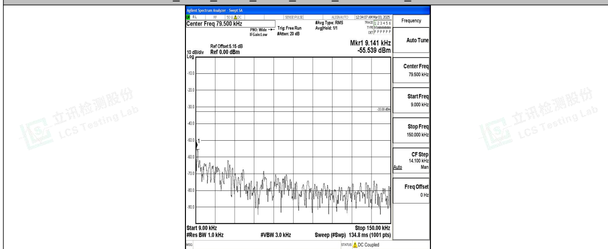
Band5_5MHz_16QAM_20425_1RB#0_0.009~0.15_0.009~0.15
