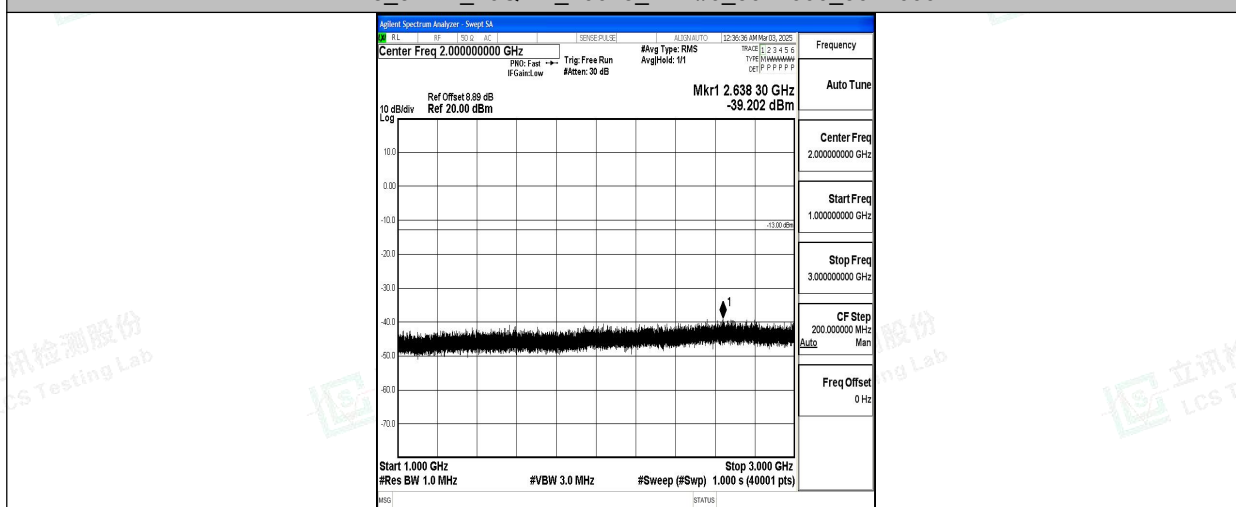
Band5_5MHz_16QAM_20625_1RB#0_1000~3000_1000~3000
