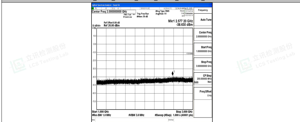
Band5_5MHz_16QAM_20425_1RB#0_1000~3000_1000~3000
