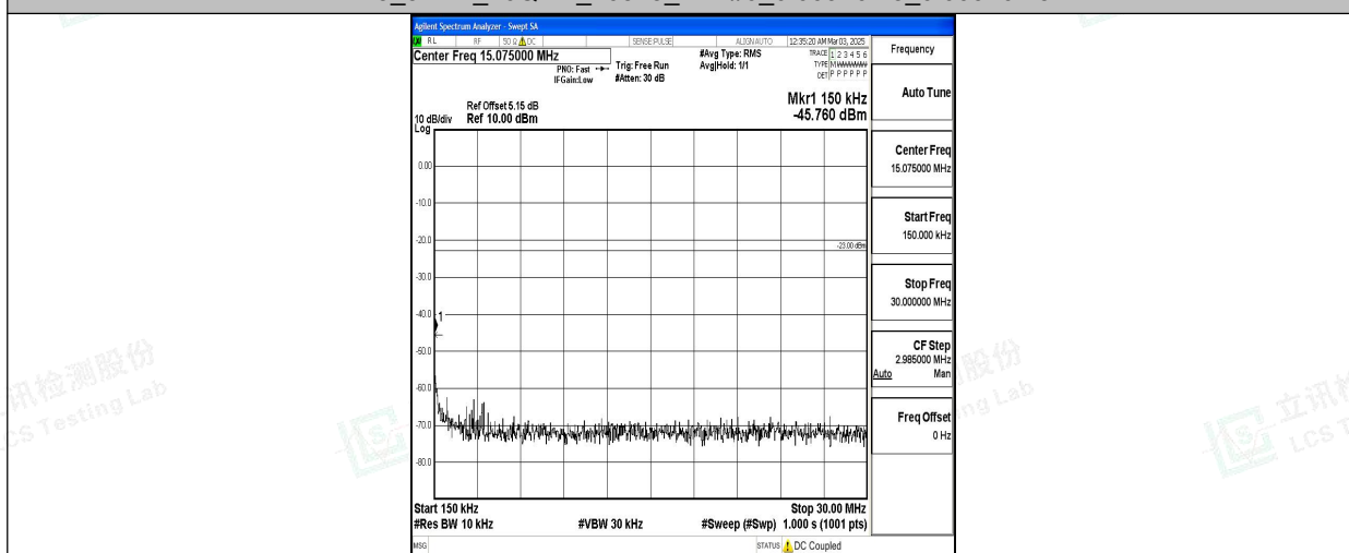
Band5_5MHz_16QAM_20525_1RB#0_0.15~30_0.15~30
