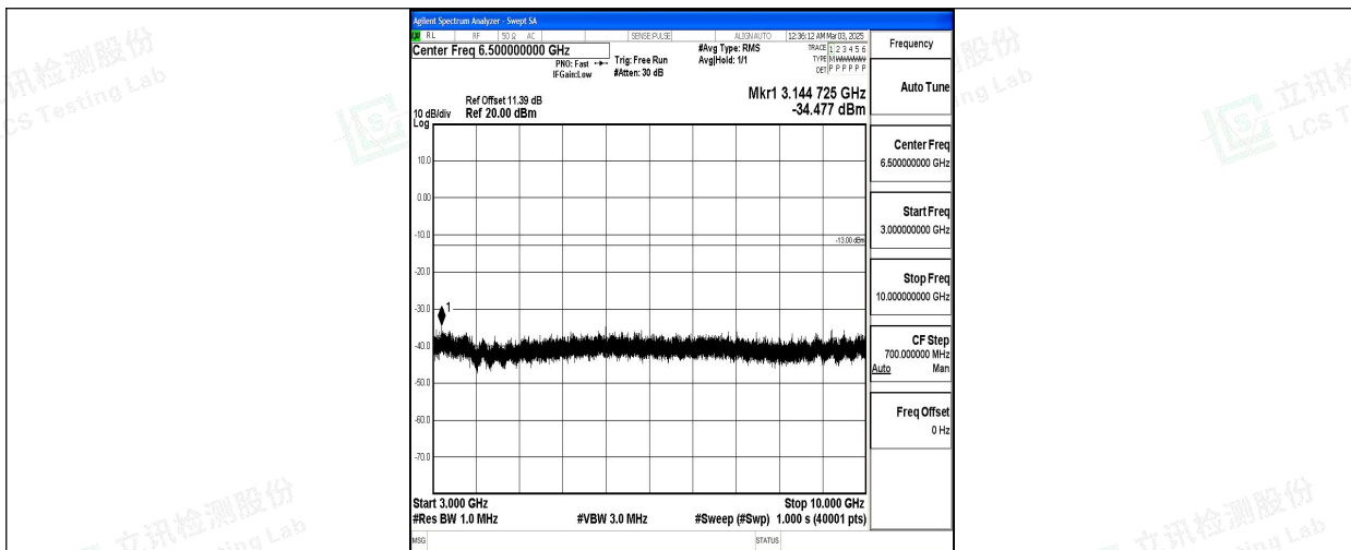
Band5_5MHz_QPSK_20625_1RB#0_3000~10000_3000~10000
