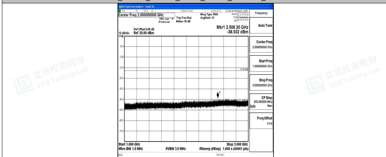
Band5_10MHz_16QAM_20450_1RB#0_1000~3000_1000~3000
