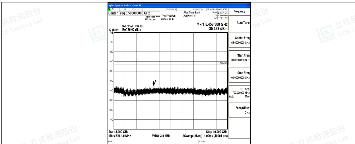
Band5_5MHz_16QAM_20425_1RB#0_3000~10000_3000~10000
