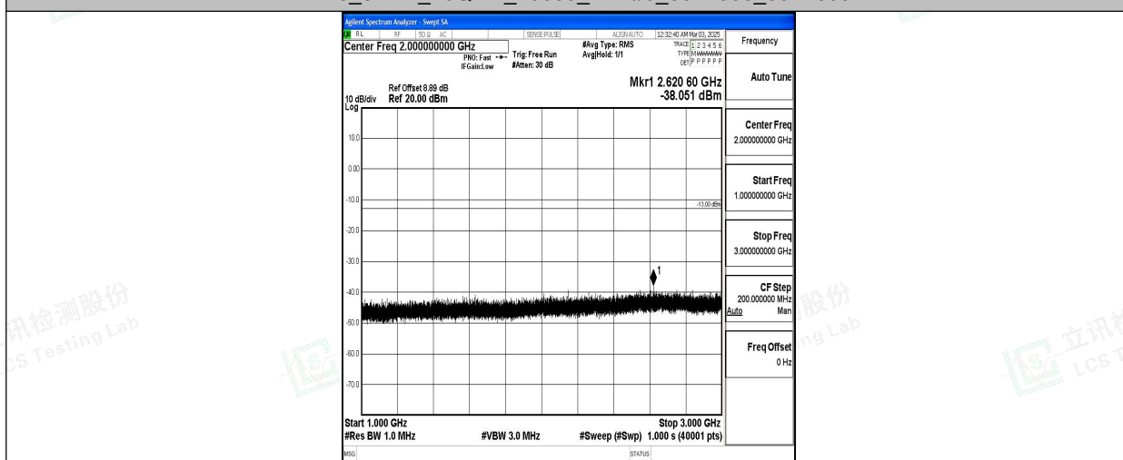
Band5_3MHz_16QAM_20635_1RB#0_1000~3000_1000~3000
