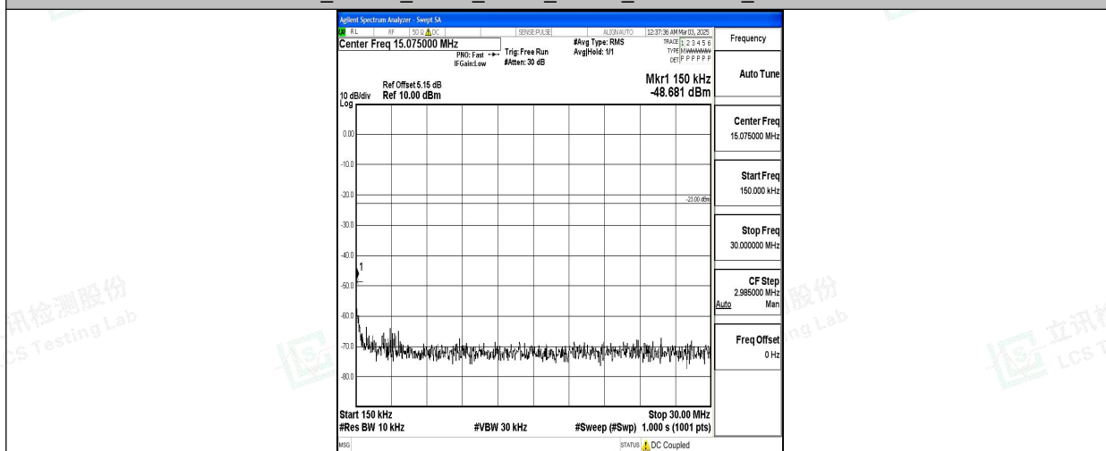
Band5_10MHz_QPSK_20450_1RB#0_0.15~30_0.15~30
