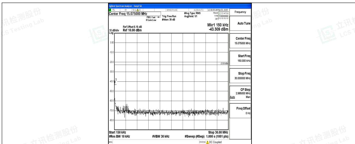
Band5_10MHz_16QAM_20450_1RB#0_0.15~30_0.15~30
