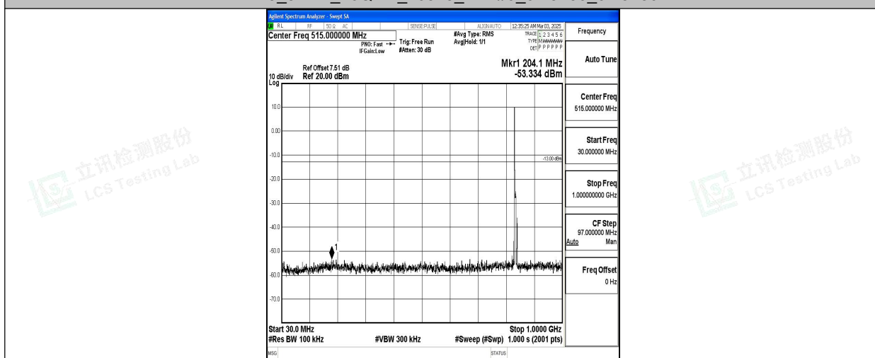
Band5_5MHz_16QAM_20525_1RB#0_30~1000_30~1000
