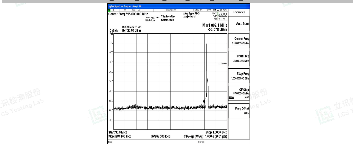
Band5_10MHz_16QAM_20450_1RB#0_30~1000_30~1000
