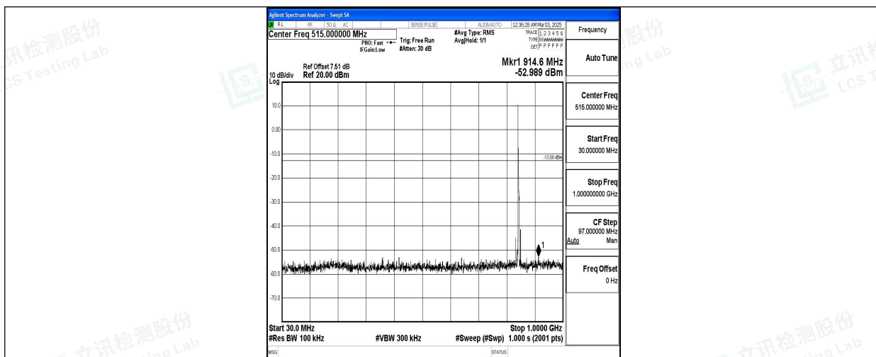
Band5_5MHz_16QAM_20625_1RB#0_30~1000_30~1000
