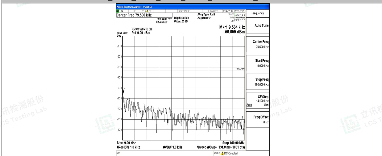
Band5_5MHz_16QAM_20625_1RB#0_0.009~0.15_0.009~0.15
