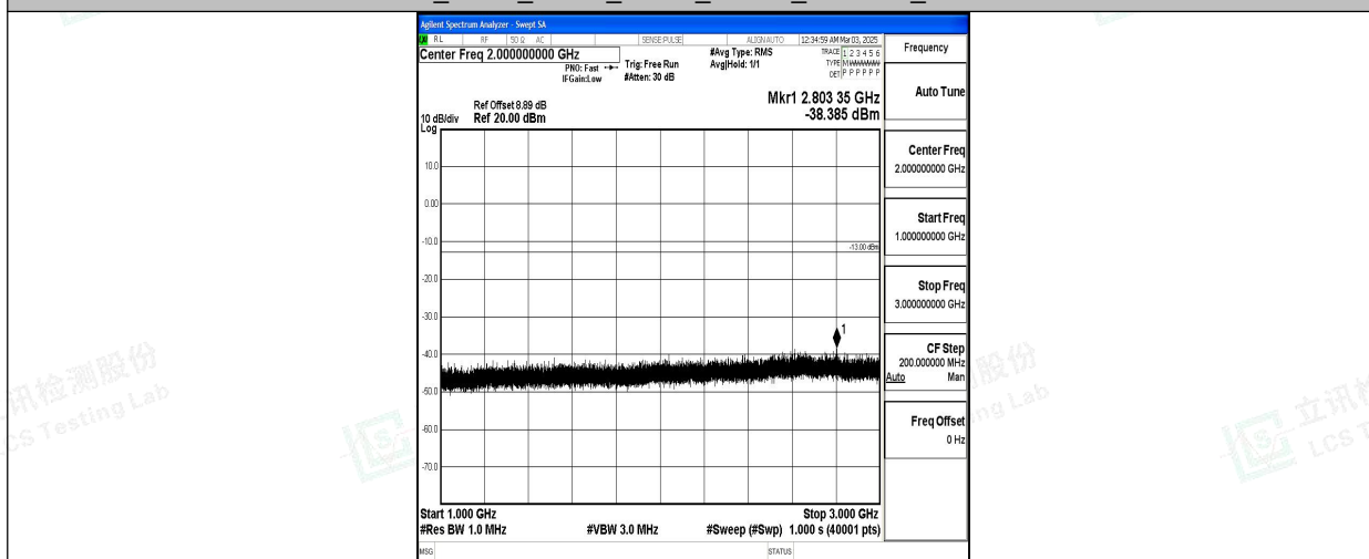
Band5_5MHz_QPSK_20525_1RB#0_1000~3000_1000~3000
