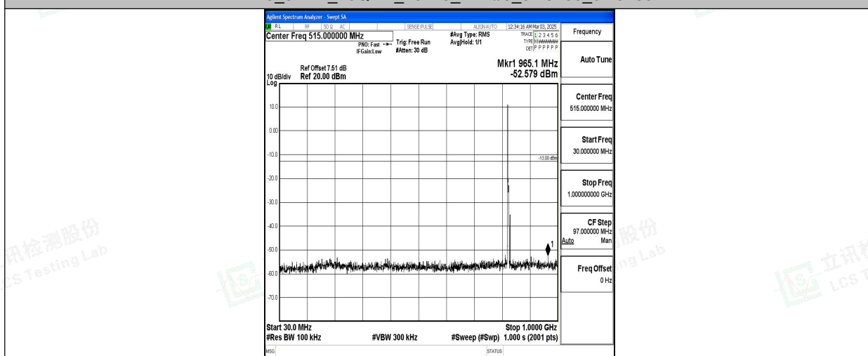
Band5_5MHz_16QAM_20425_1RB#0_30~1000_30~1000
