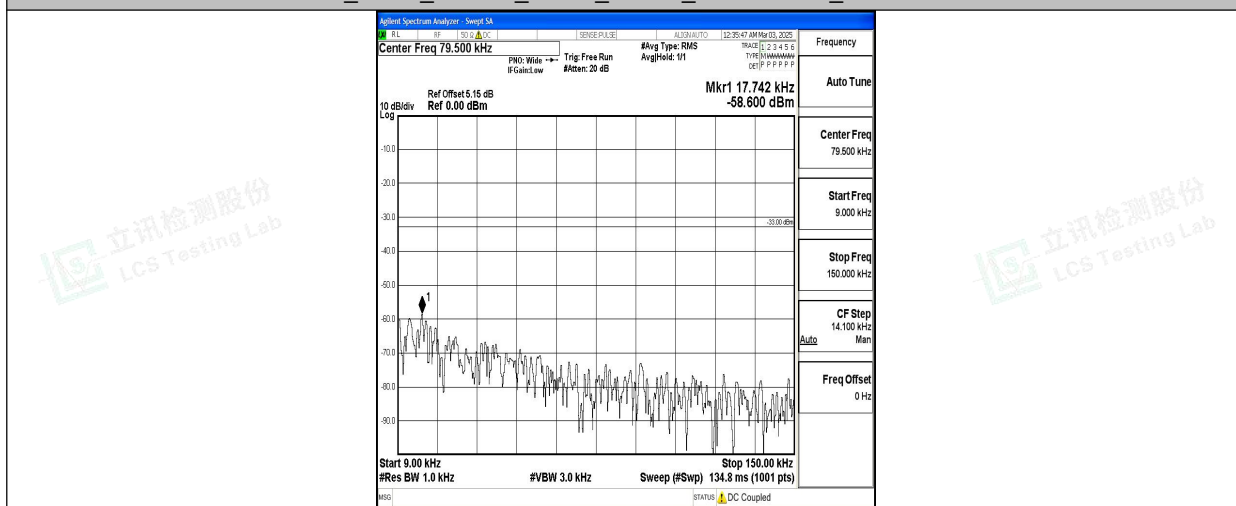
Band5_5MHz_QPSK_20625_1RB#0_0.009~0.15_0.009~0.15
