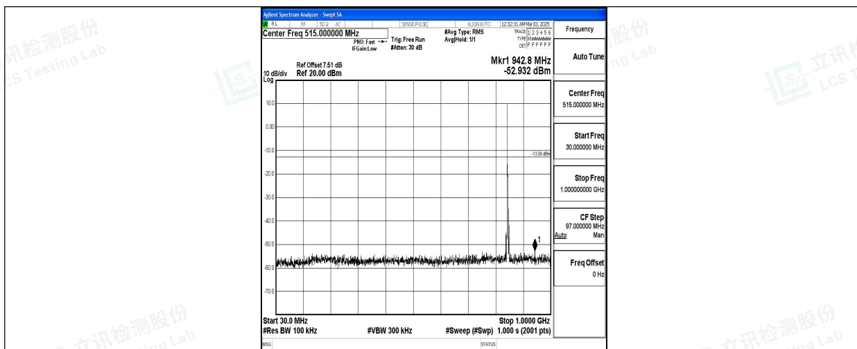
Band5_3MHz_16QAM_20635_1RB#0_30~1000_30~1000
