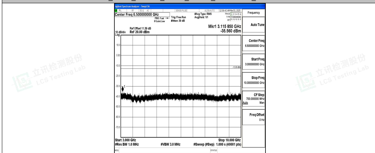
Band5_5MHz_16QAM_20625_1RB#0_3000~10000_3000~10000
