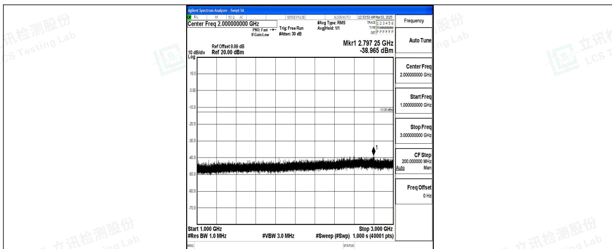
Band5_5MHz_QPSK_20425_1RB#0_1000~3000_1000~3000
