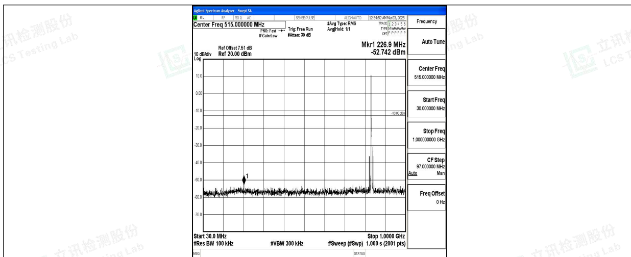
Band5_5MHz_QPSK_20525_1RB#0_30~1000_30~1000
