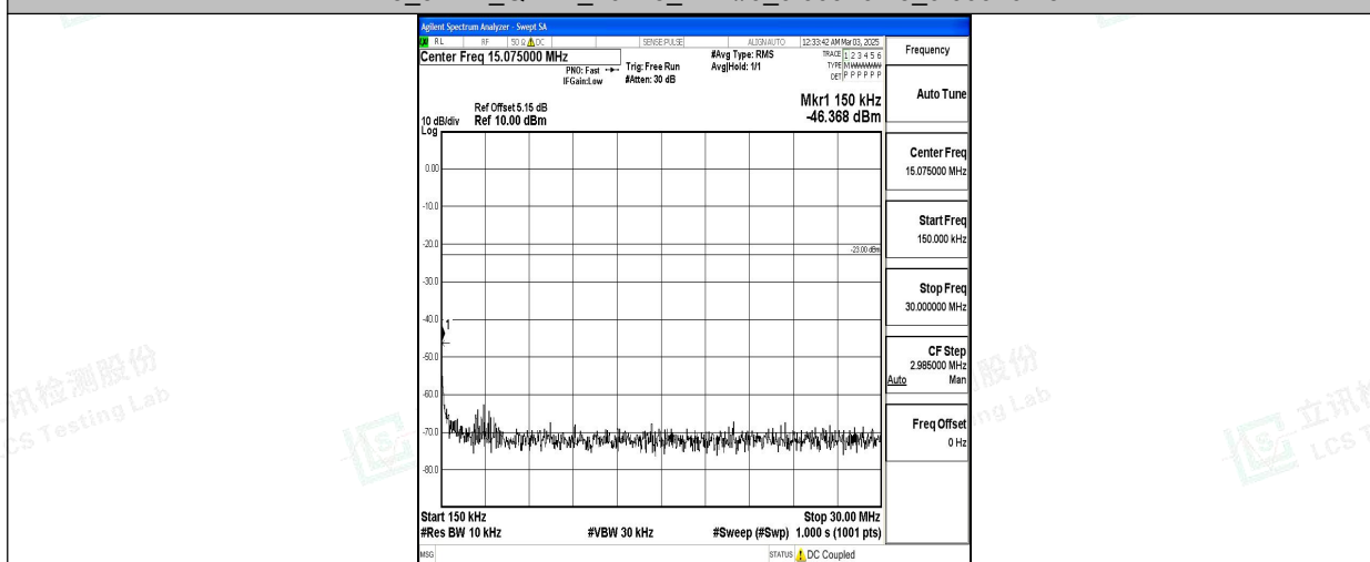
Band5_5MHz_QPSK_20425_1RB#0_0.15~30_0.15~30
