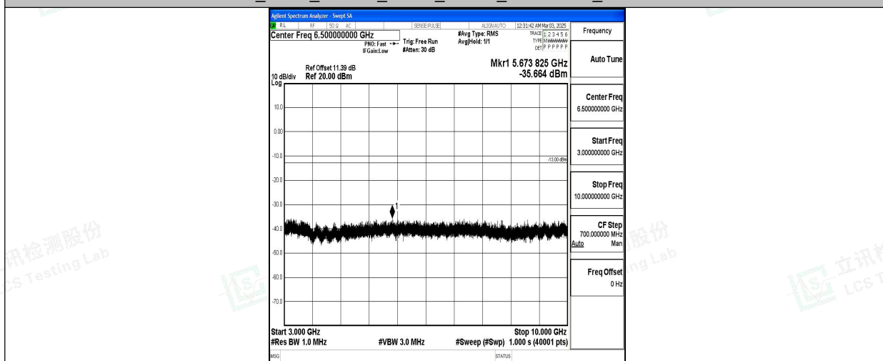
Band5_3MHz_16QAM_20525_1RB#0_3000~10000_3000~10000
