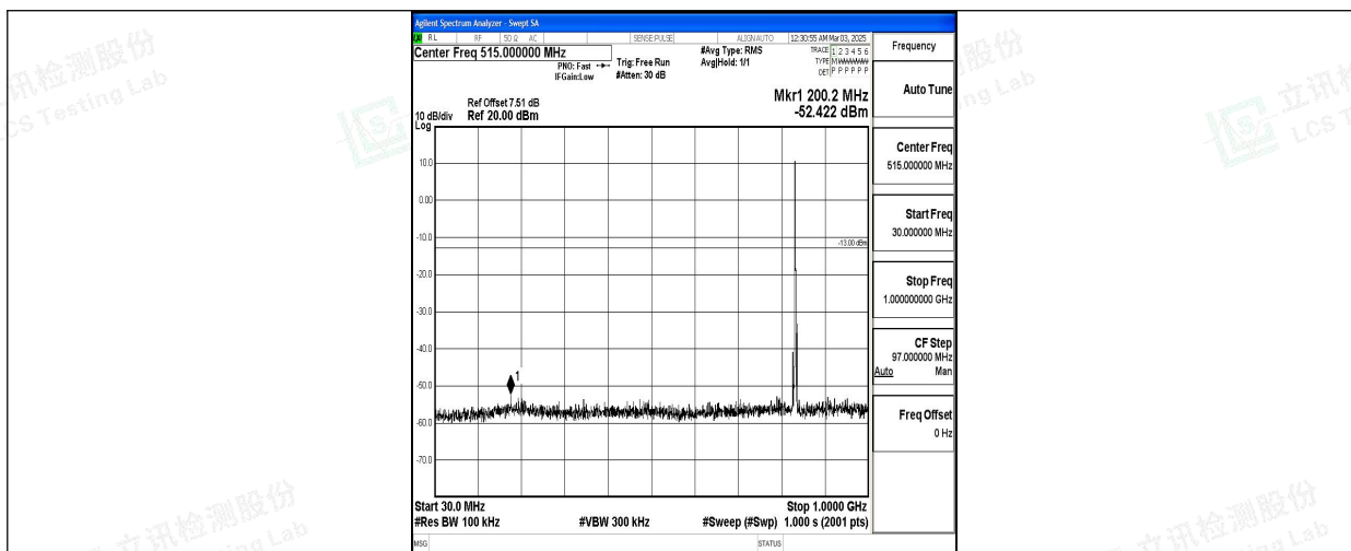
Band5_3MHz_QPSK_20525_1RB#0_30~1000_30~1000
