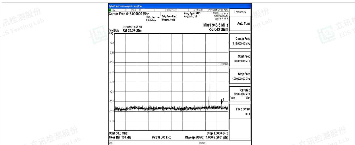
Band5_1.4MHz_QPSK_20525_1RB#0_30~1000_30~1000
