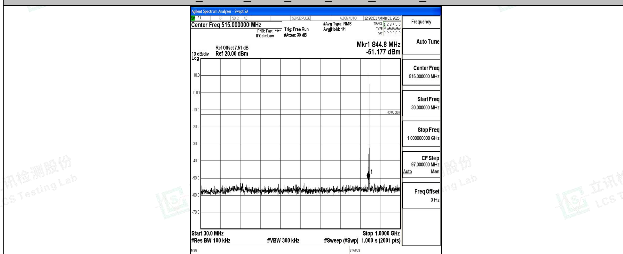
Band5_1.4MHz_QPSK_20643_1RB#0_30~1000_30~1000
