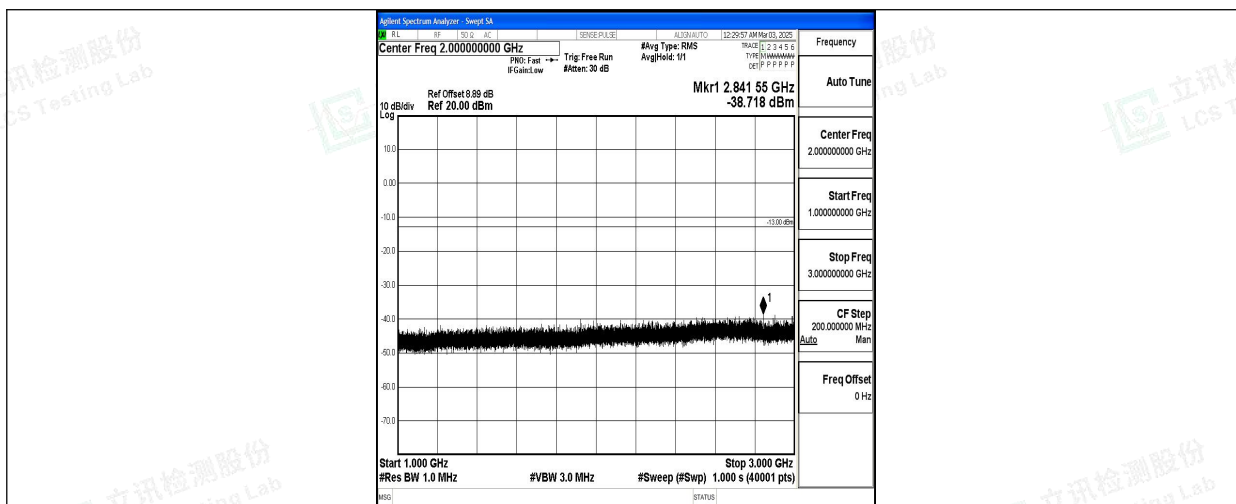
Band5_3MHz_QPSK_20415_1RB#0_1000~3000_1000~3000
