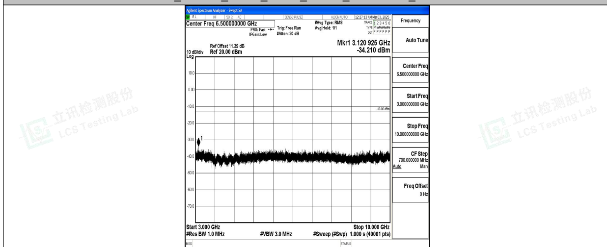
Band5_1.4MHz_QPSK_20525_1RB#0_3000~10000_3000~10000
