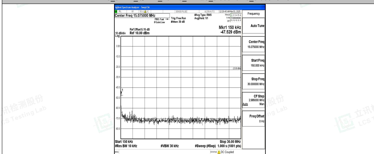
Band5_3MHz_QPSK_20415_1RB#0_0.15~30_0.15~30
