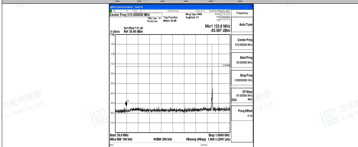
Band5_3MHz_QPSK_20635_1RB#0_30~1000_30~1000
