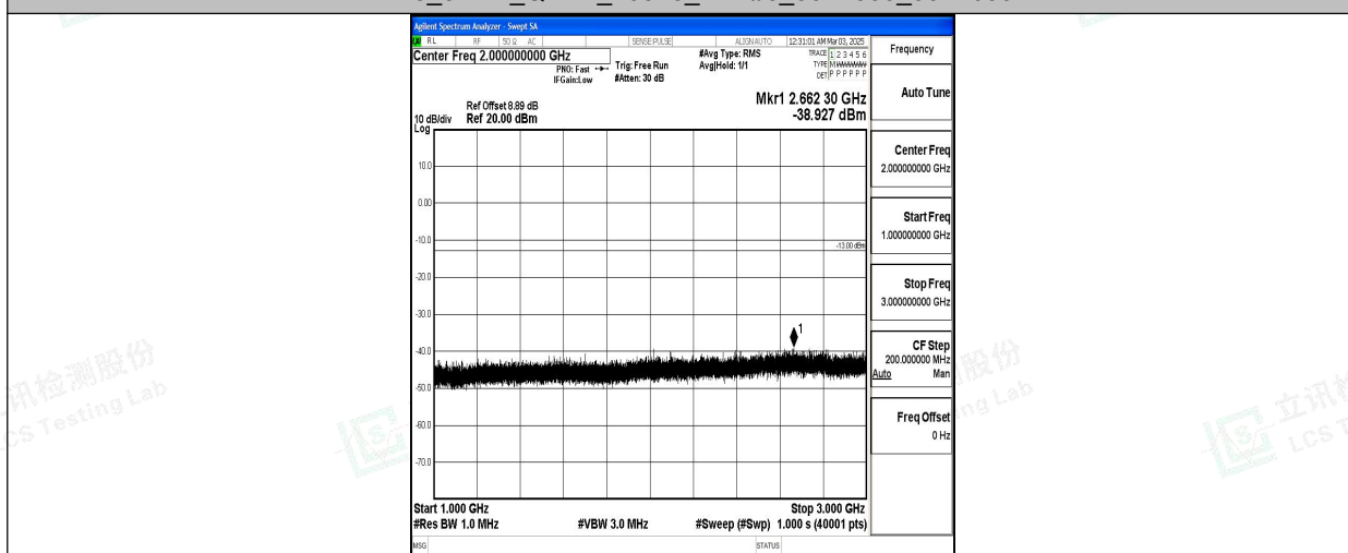
Band5_3MHz_QPSK_20525_1RB#0_1000~3000_1000~3000
