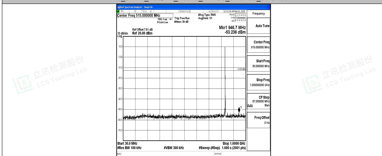
Band5_3MHz_16QAM_20525_1RB#0_30~1000_30~1000
