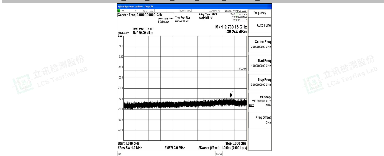
Band5_3MHz_QPSK_20635_1RB#0_1000~3000_1000~3000
