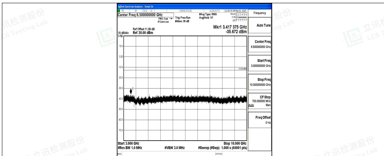
Band5_1.4MHz_QPSK_20643_1RB#0_3000~10000_3000~10000
