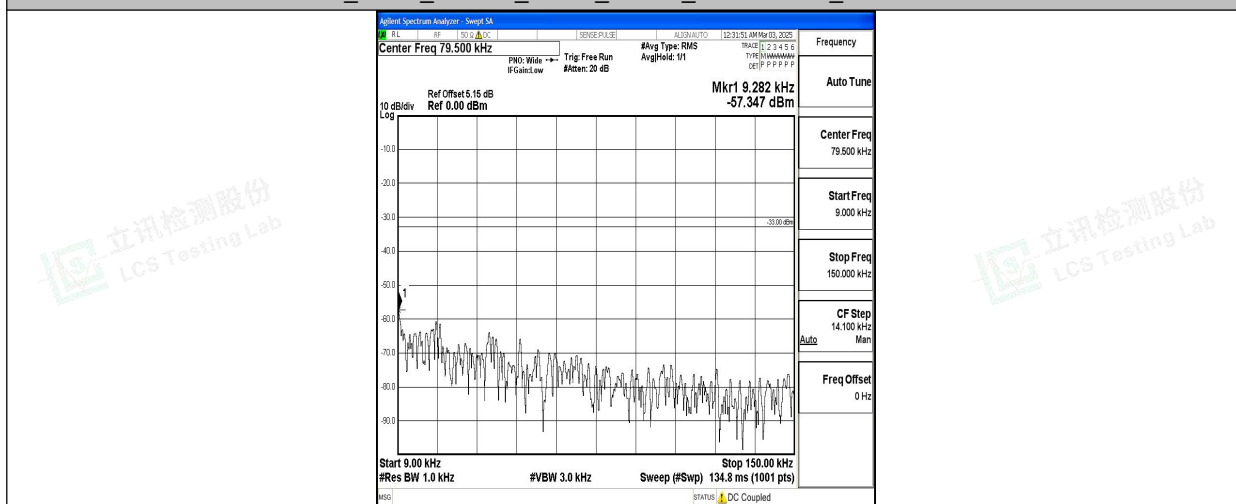
Band5_3MHz_QPSK_20635_1RB#0_0.009~0.15_0.009~0.15
