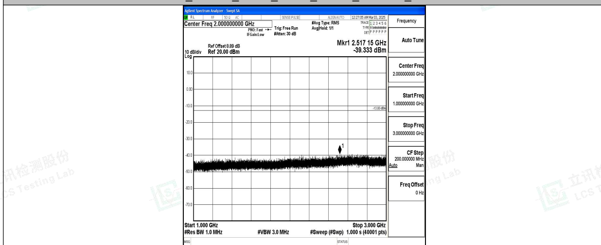
Band5_1.4MHz_QPSK_20525_1RB#0_1000~3000_1000~3000
