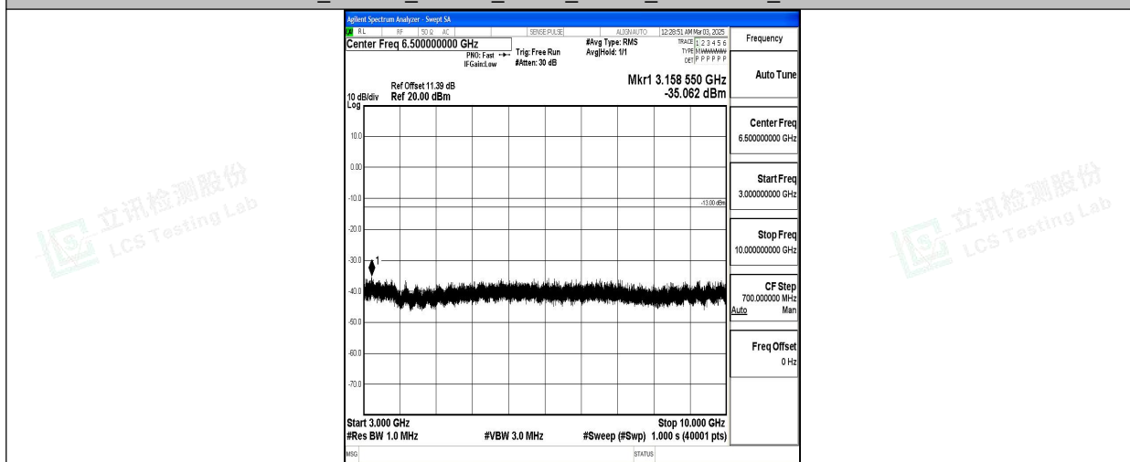
Band5_1.4MHz_16QAM_20643_1RB#0_3000~10000_3000~10000
