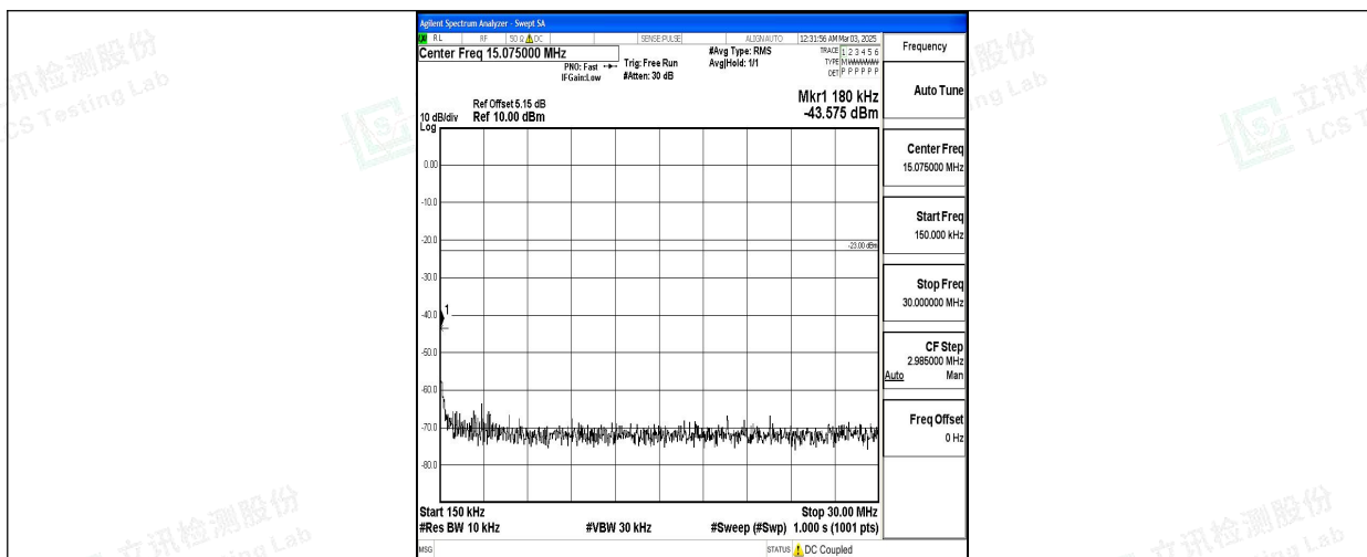
Band5_3MHz_QPSK_20635_1RB#0_0.15~30_0.15~30
