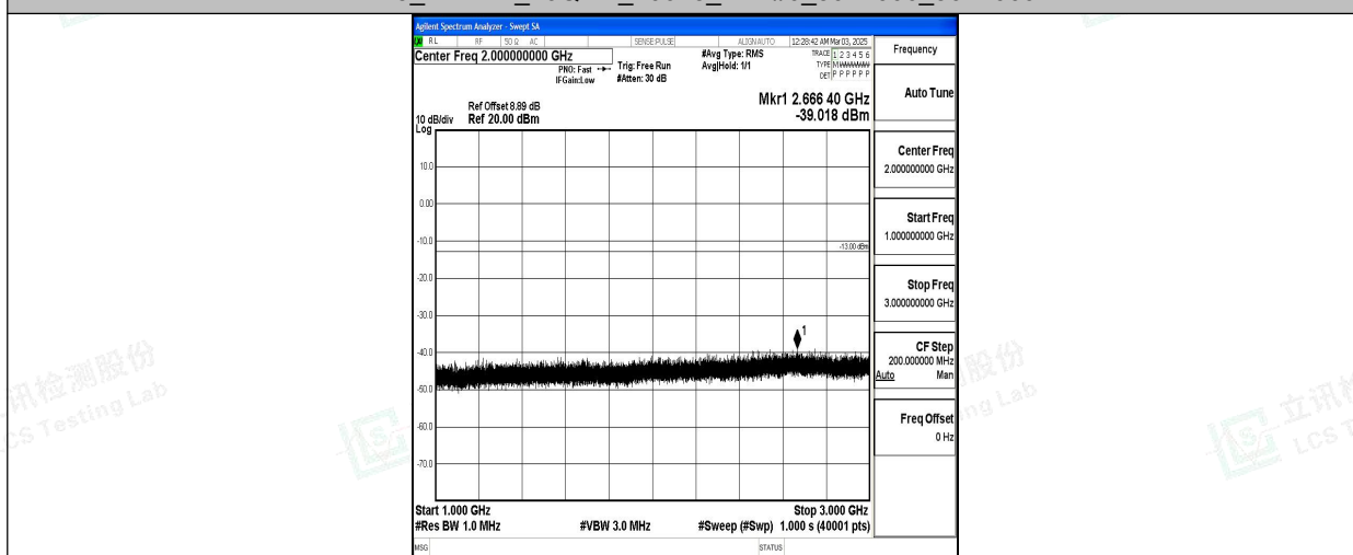
Band5_1.4MHz_16QAM_20643_1RB#0_1000~3000_1000~3000
