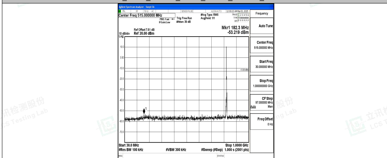
Band5_3MHz_16QAM_20415_1RB#0_30~1000_30~1000
