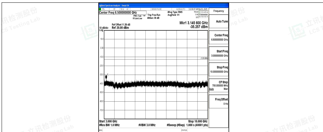
Band5_3MHz_16QAM_20415_1RB#0_3000~10000_3000~10000
