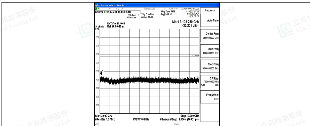
Band5_1.4MHz_16QAM_20407_1RB#0_3000~10000_3000~10000
