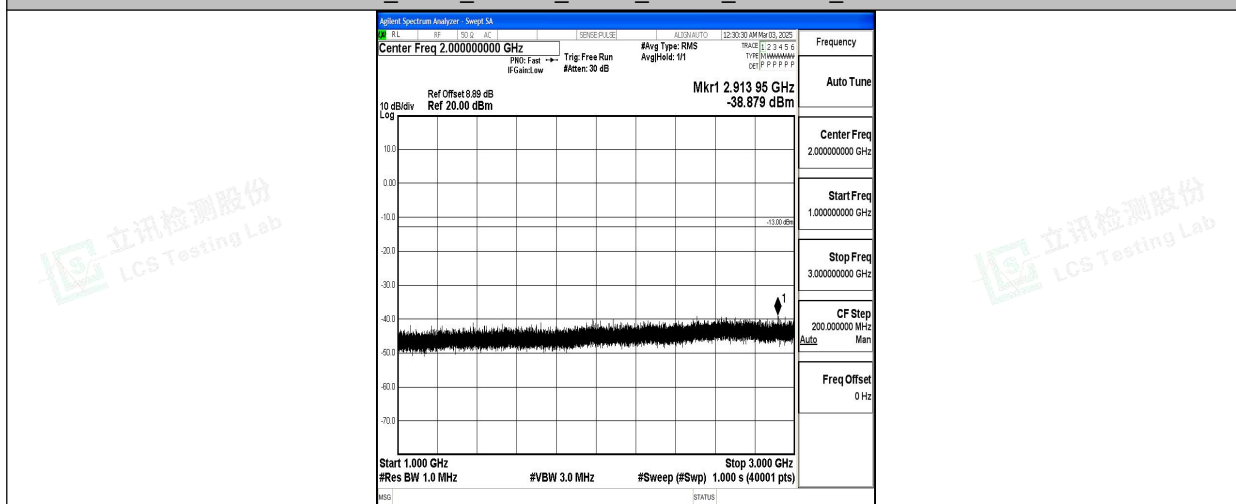
Band5_3MHz_16QAM_20415_1RB#0_1000~3000_1000~3000
