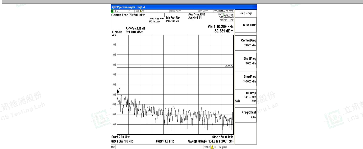
Band5_3MHz_QPSK_20525_1RB#0_0.009~0.15_0.009~0.15
