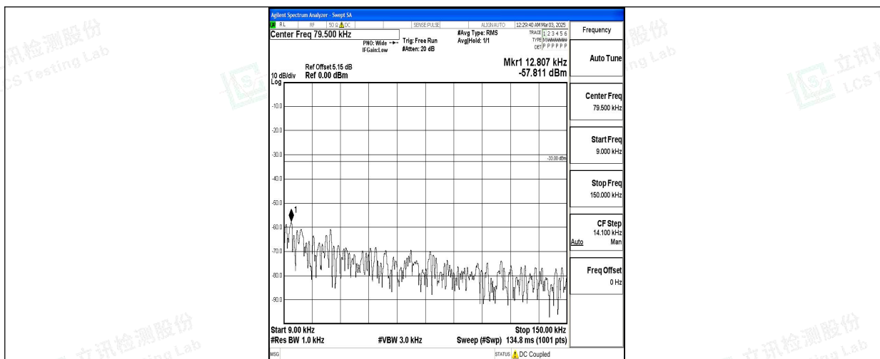
Band5_3MHz_QPSK_20415_1RB#0_0.009~0.15_0.009~0.15
