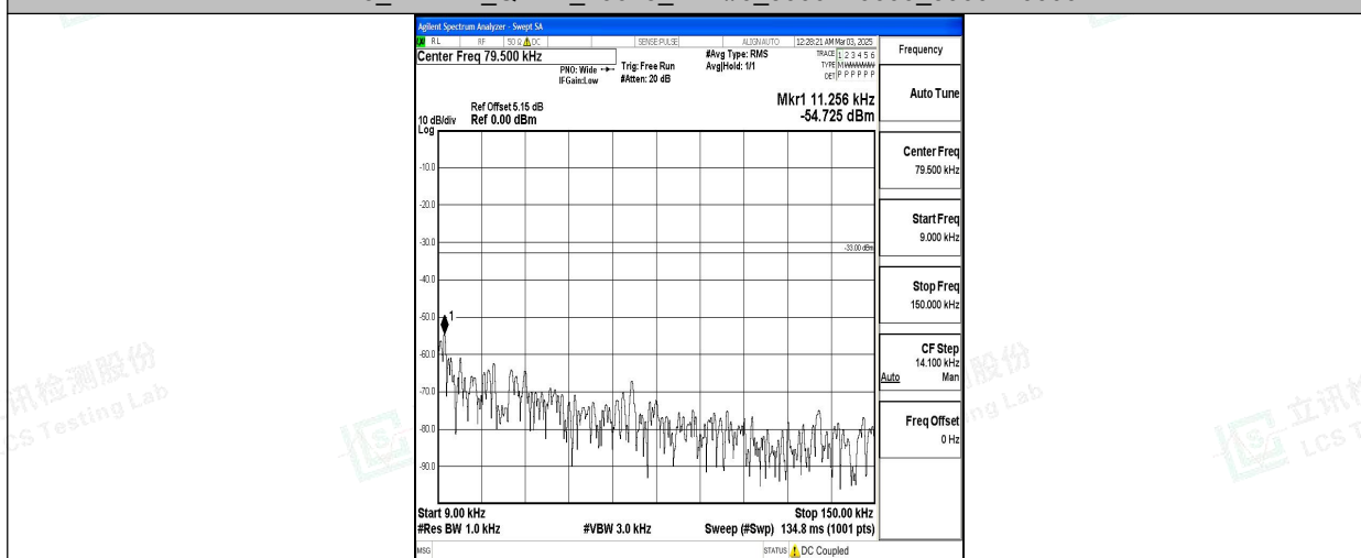
Band5_1.4MHz_16QAM_20643_1RB#0_0.009~0.15_0.009~0.15
