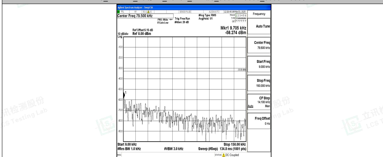
Band5_1.4MHz_QPSK_20525_1RB#0_0.009~0.15_0.009~0.15
