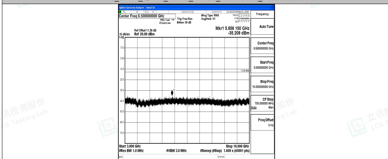
Band5_3MHz_QPSK_20415_1RB#0_3000~10000_3000~10000
