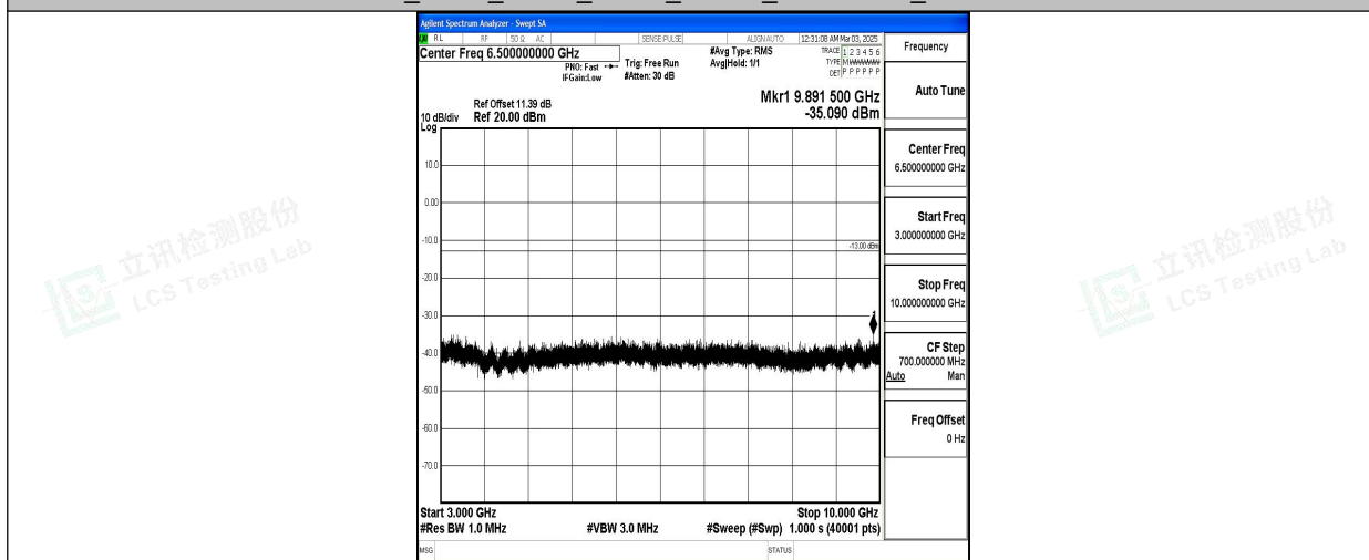
Band5_3MHz_QPSK_20525_1RB#0_3000~10000_3000~10000
