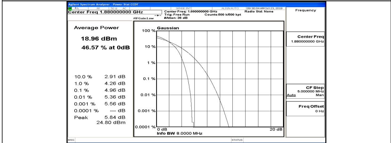
Peak-to Average Ratio Test Graph(s) (Channel Bandwidth:15 MHz)_MCH_QPSK
