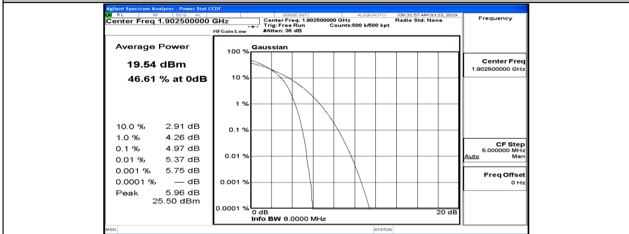
Peak-to Average Ratio Test Graph(s) (Channel Bandwidth:15 MHz)_HCH_QPSK
