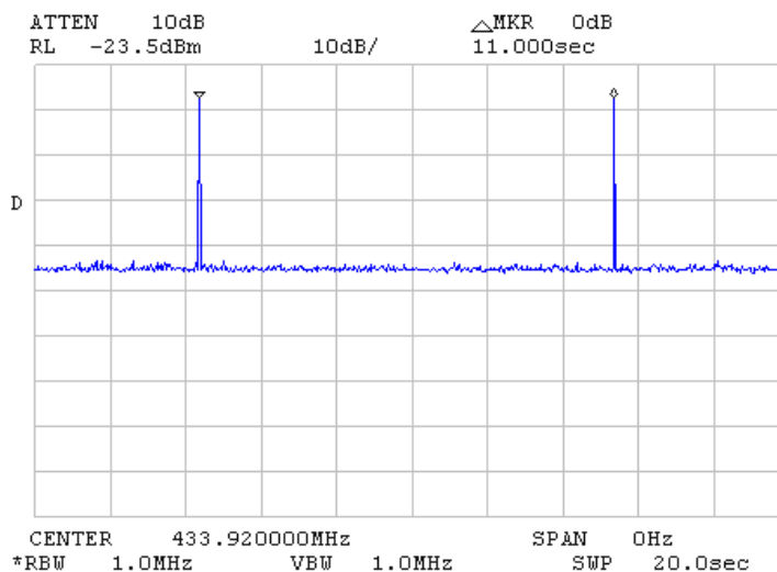
Plot 7.2.17 Transmission pulse period
