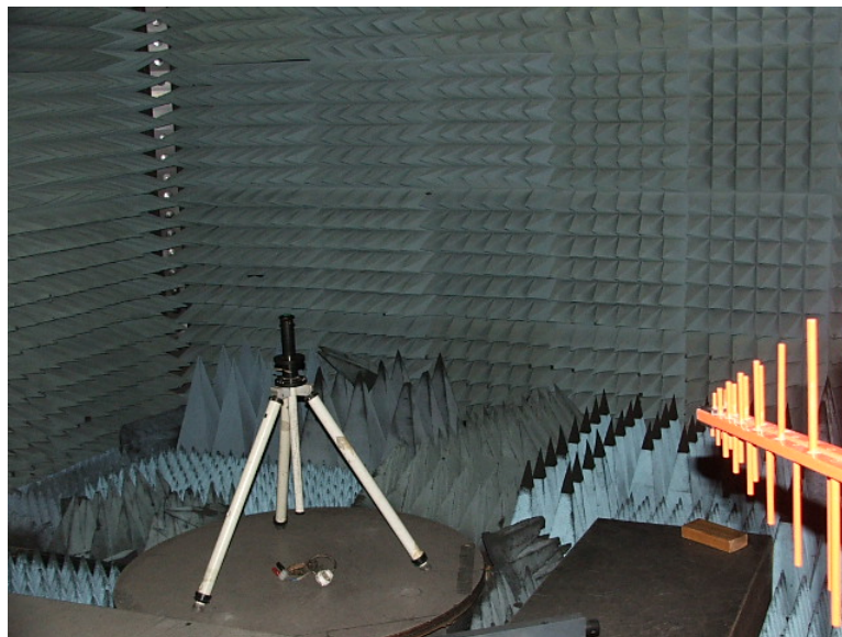
Photograph 8.1.1 Setup for p radiated emission measurements
