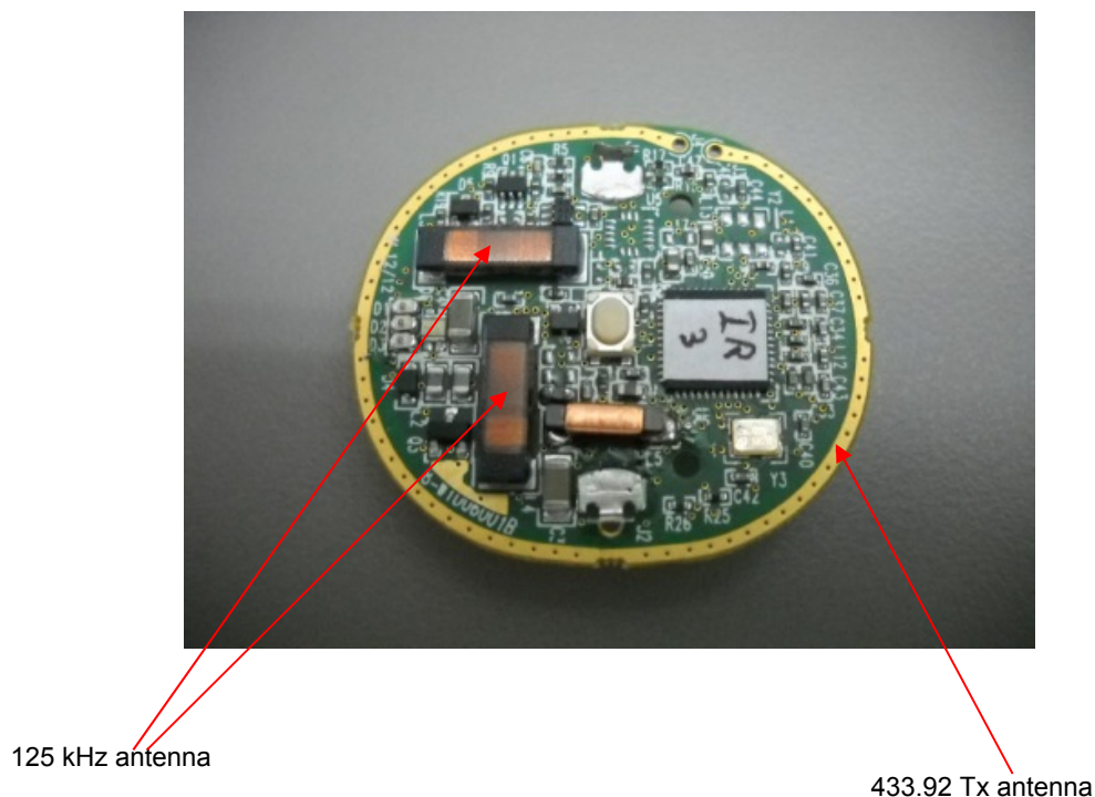
Photograph 7.4.1 Antenna assembly
