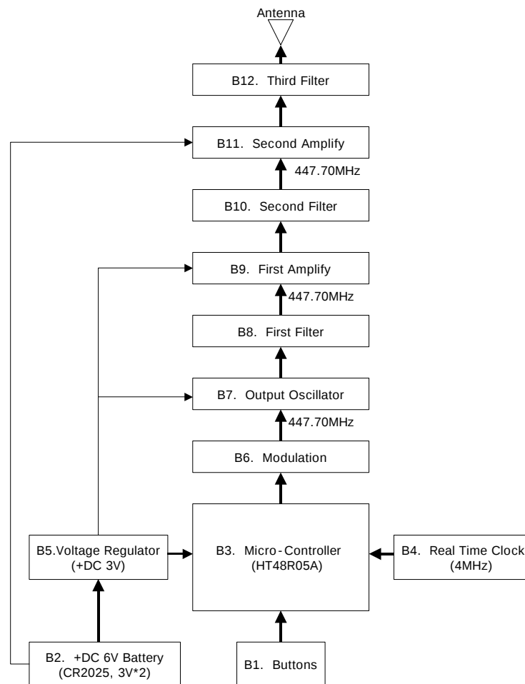
O44JR1700F447 Block Diagram (B1<Block1> ~ B12<Block12>)
