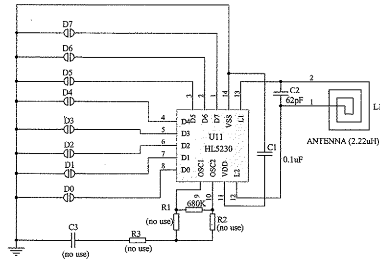
Big TAG CIRCUIT( PCB Size: 20X20mm )
