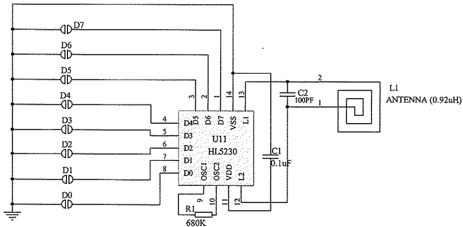
Little TAG CIRCUIT(PCB SIZE: 10X10mm)
