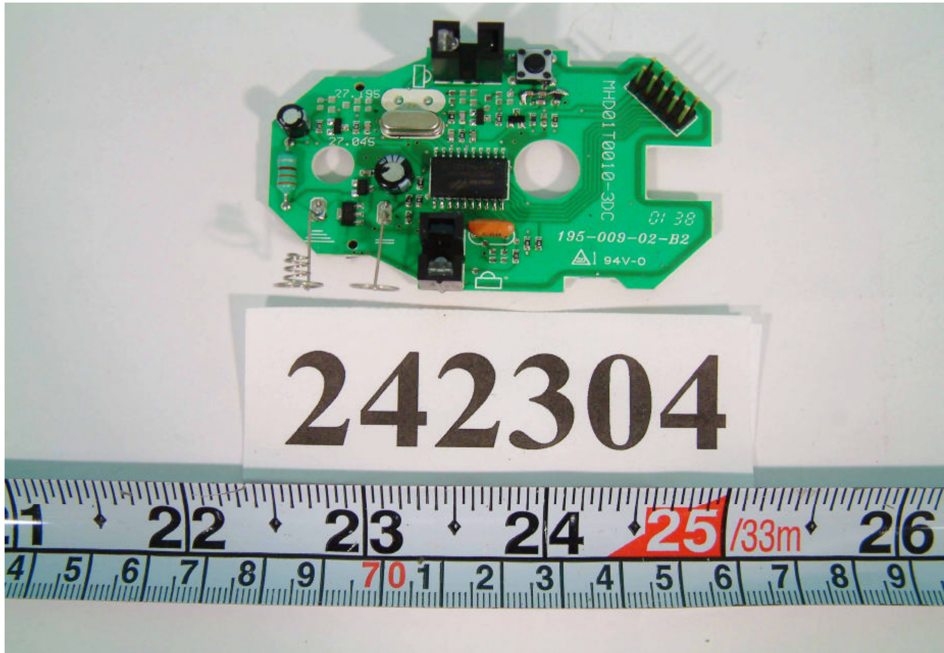
Front side of Main Board Of Mouse
