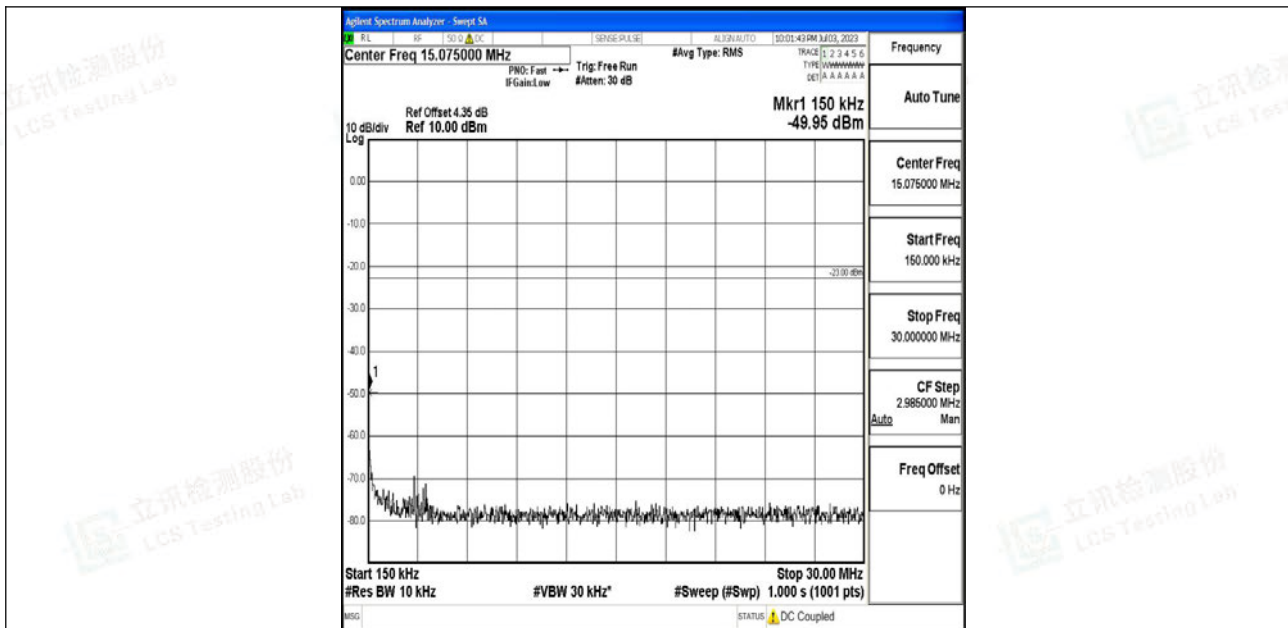
Band12_5MHz_16QAM_23035_1RB#0_0.15~30_0.15~30
