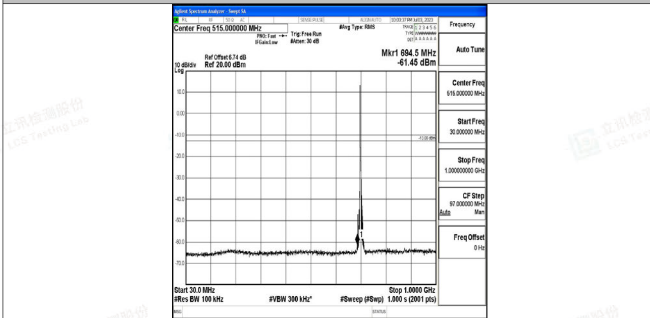
Band12_5MHz_16QAM_23095_1RB#0_30~1000_30~1000
