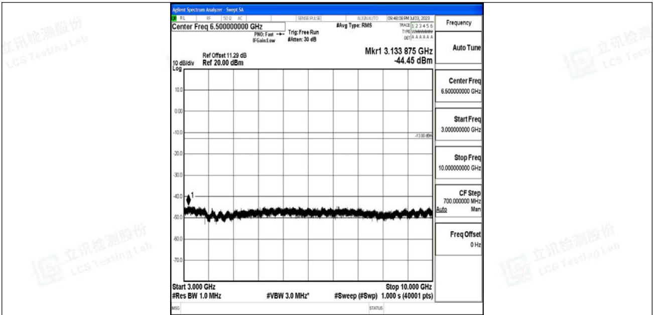
Band12_1.4MHz_QPSK_23173_1RB#0_3000~10000_3000~10000
