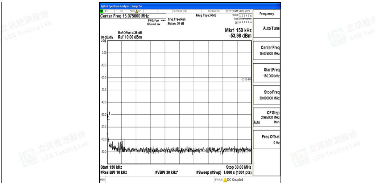
Band12_5MHz_16QAM_23155_1RB#0_0.15~30_0.15~30
