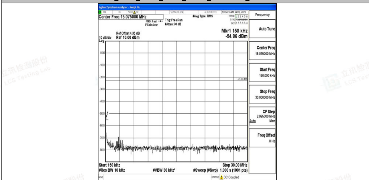
Band12_5MHz_QPSK_23155_1RB#0_0.15~30_0.15~30
