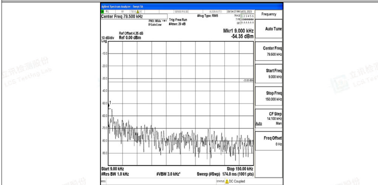
Band12_3MHz_16QAM_23095_1RB#0_0.009~0.15_0.009~0.15
