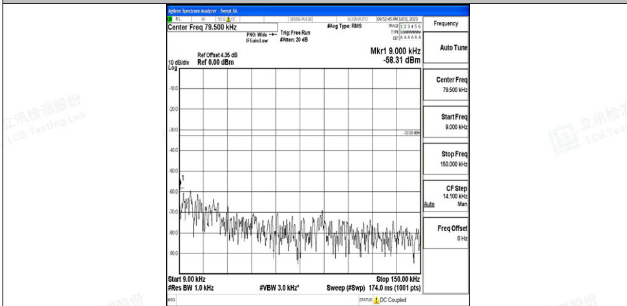
Band12_3MHz_16QAM_23025_1RB#0_0.009~0.15_0.009~0.15
