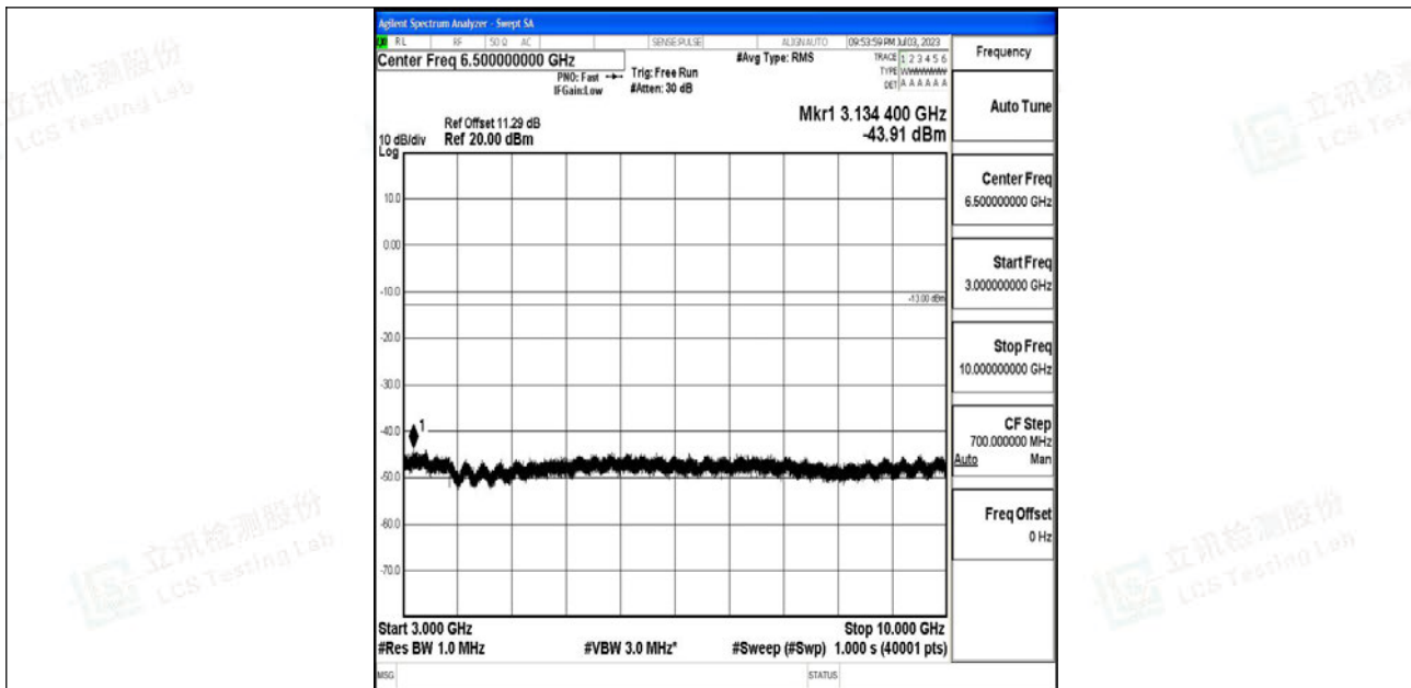
Band12_3MHz_QPSK_23095_1RB#0_3000~10000_3000~10000
