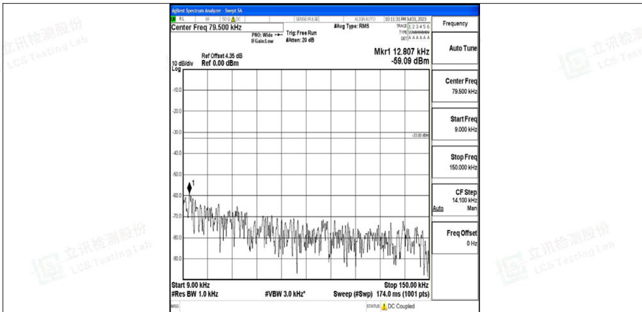
Band12_10MHz_QPSK_23130_1RB#0_0.009~0.15_0.009~0.15
