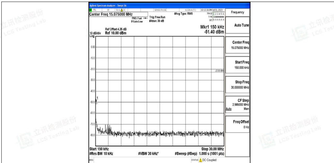
Band12_10MHz_16QAM_23130_1RB#0_0.15~30_0.15~30
