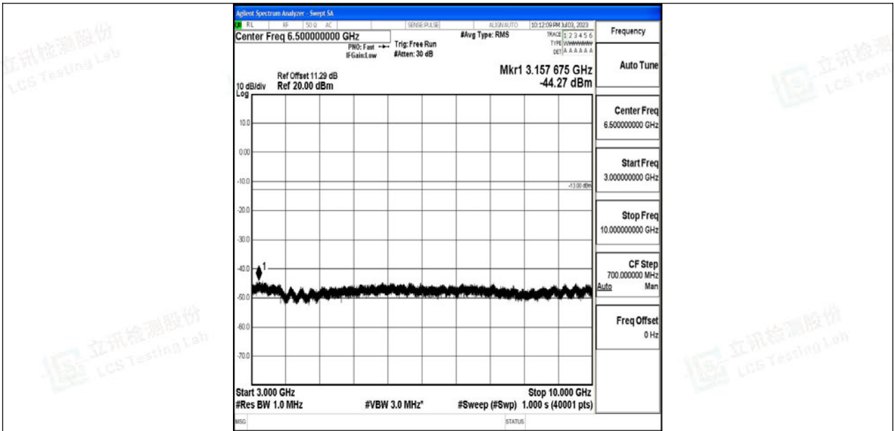
Band12_10MHz_QPSK_23130_1RB#0_3000~10000_3000~10000
