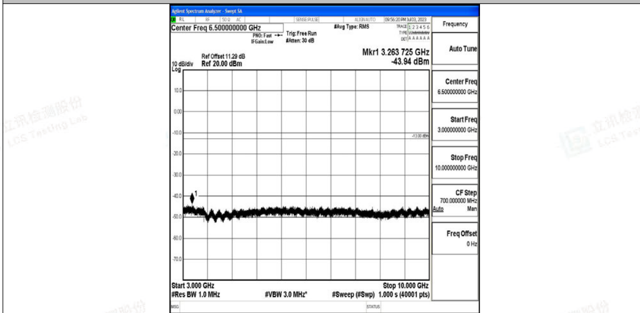
Band12_3MHz_16QAM_23165_1RB#0_3000~10000_3000~10000
