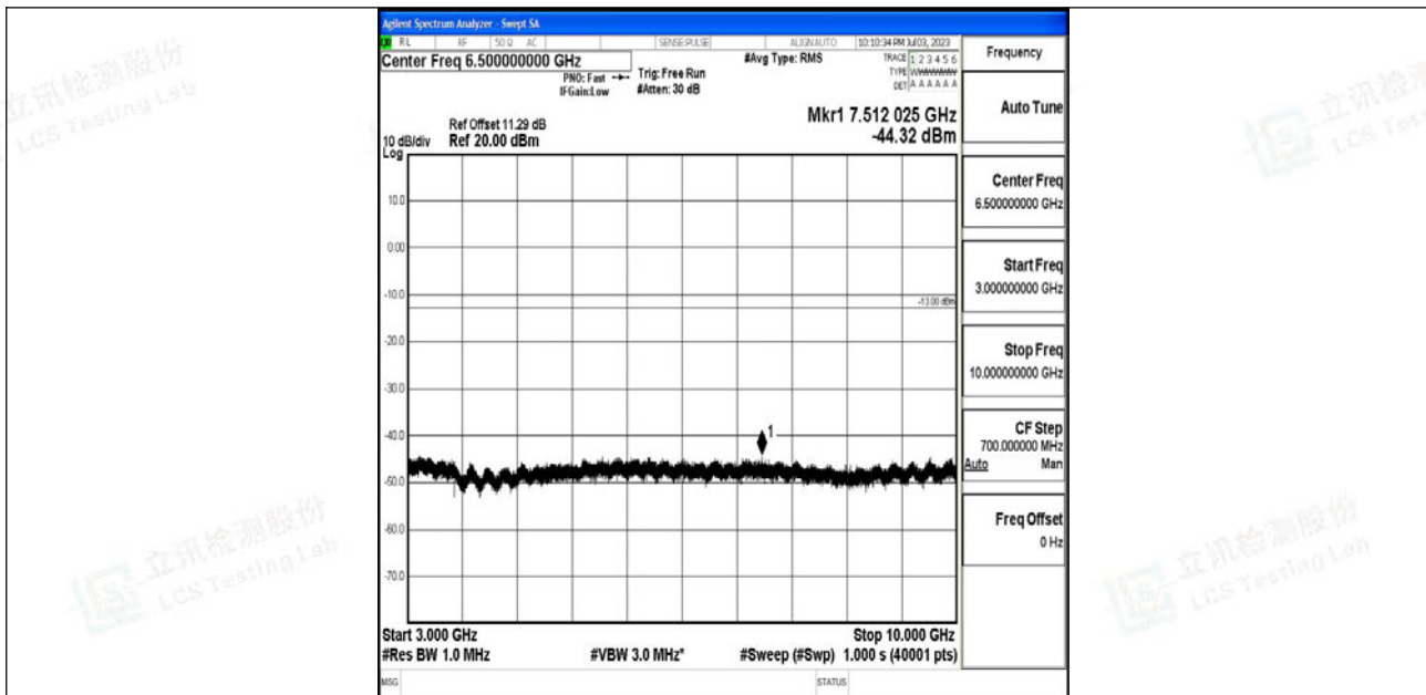
Band12_10MHz_QPSK_23095_1RB#0_3000~10000_3000~10000
