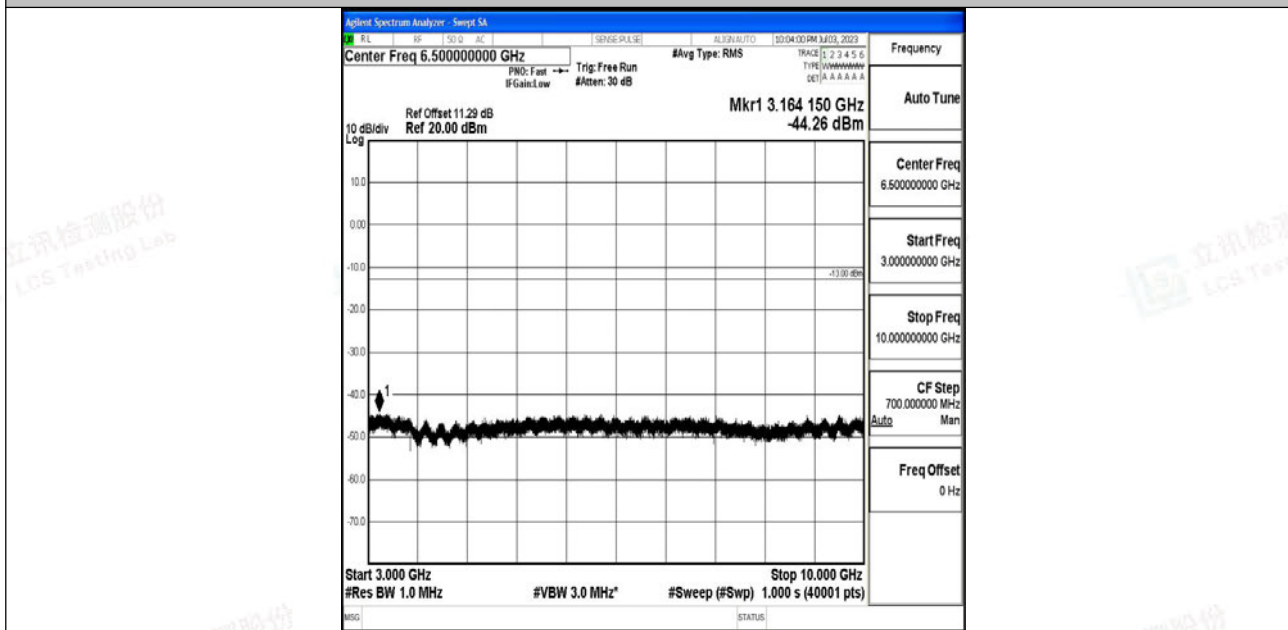
Band12_5MHz_16QAM_23095_1RB#0_3000~10000_3000~10000
