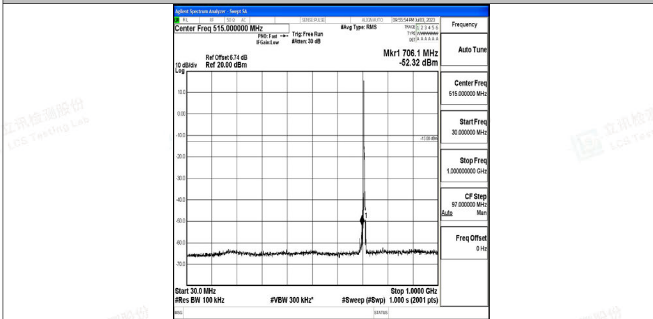
Band12_3MHz_16QAM_23165_1RB#0_30~1000_30~1000
