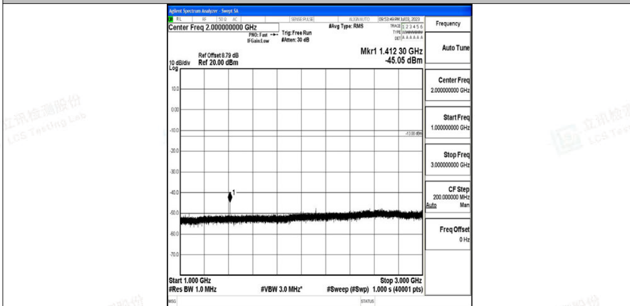
Band12_3MHz_QPSK_23095_1RB#0_1000~3000_1000~3000
