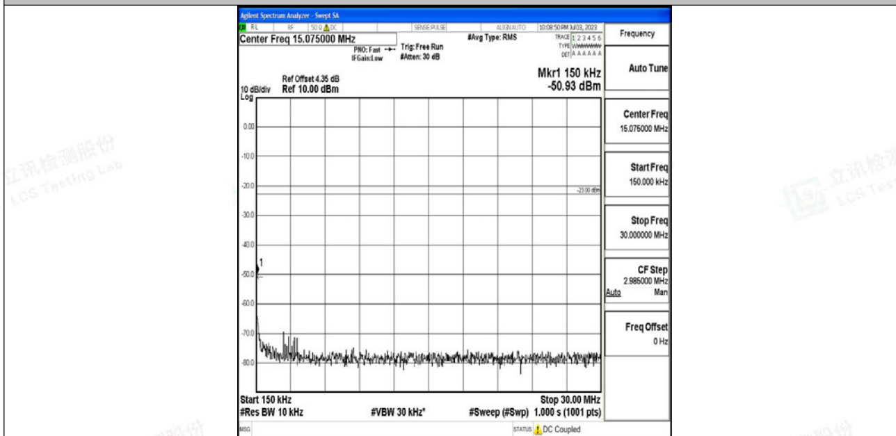
Band12_10MHz_QPSK_23060_1RB#0_0.15~30_0.15~30
