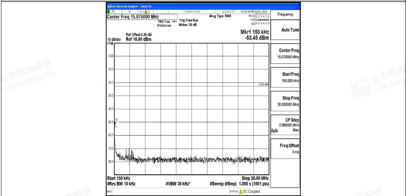
Band12_5MHz_QPSK_23095_1RB#0_0.15~30_0.15~30
