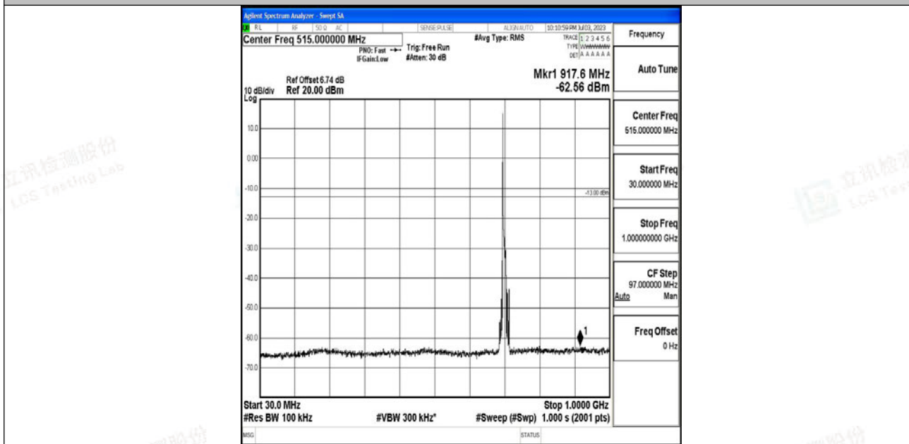
Band12_10MHz_16QAM_23095_1RB#0_30~1000_30~1000
