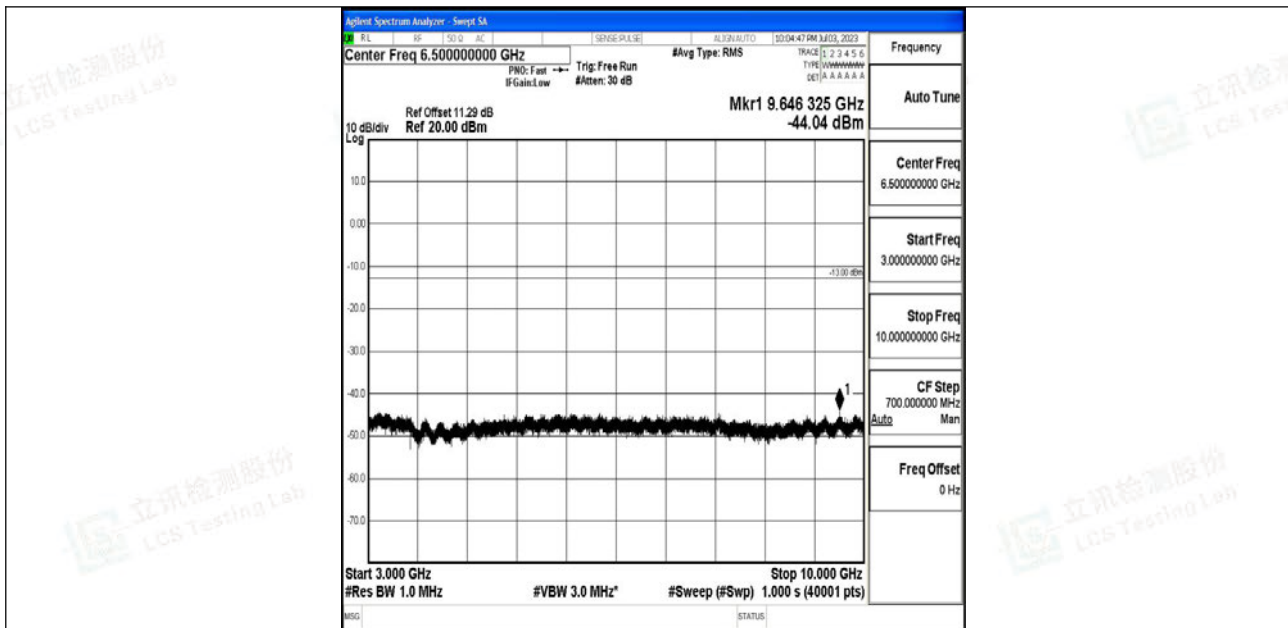
Band12_5MHz_QPSK_23155_1RB#0_3000~10000_3000~10000
