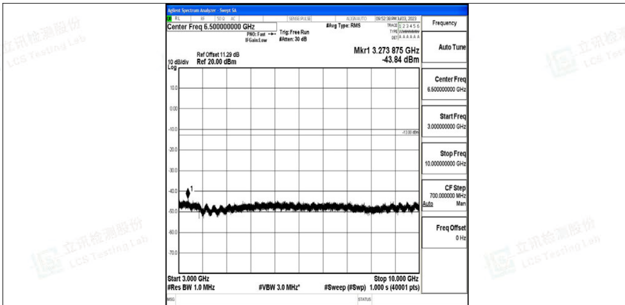
Band12_3MHz_QPSK_23025_1RB#0_3000~10000_3000~10000
