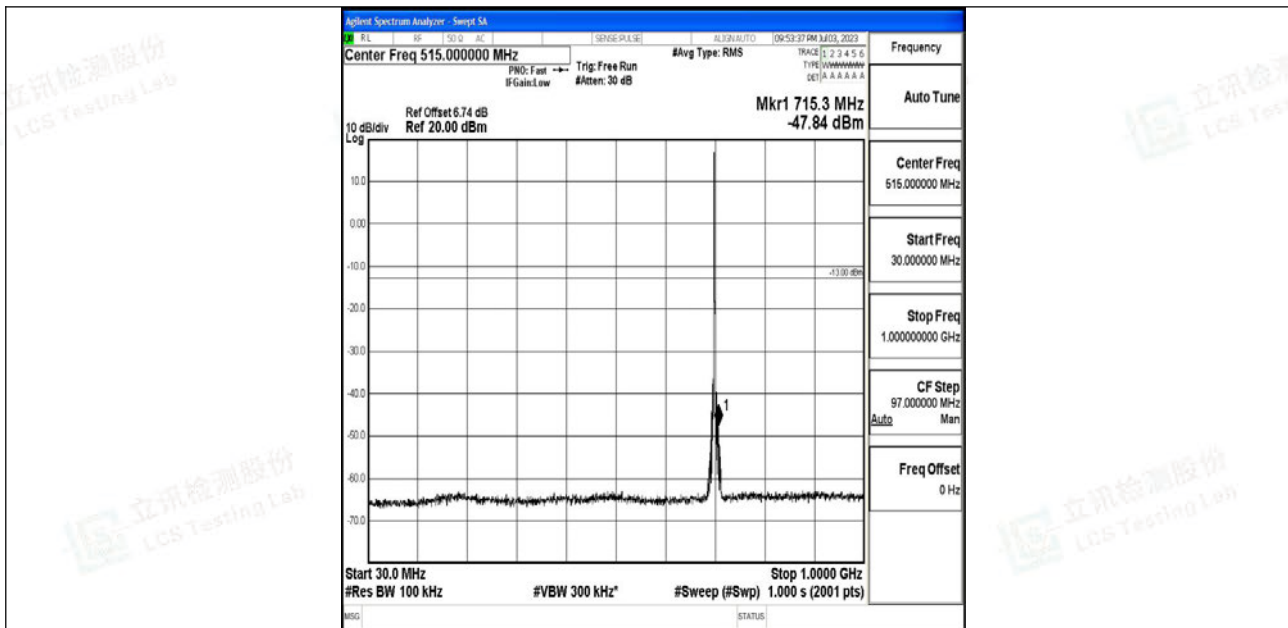
Band12_3MHz_QPSK_23095_1RB#0_30~1000_30~1000
