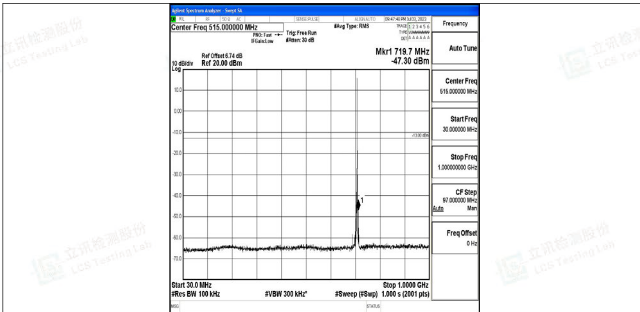
Band12_1.4MHz_QPSK_23173_1RB#0_30~1000_30~1000
