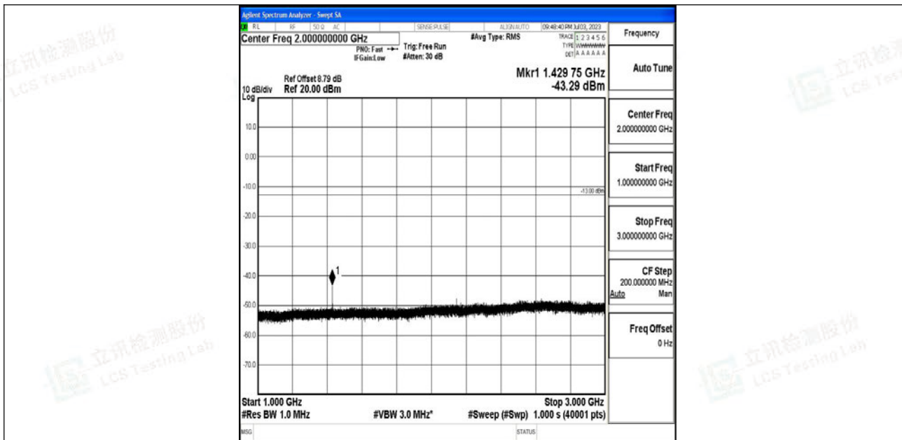
Band12_1.4MHz_16QAM_23173_1RB#0_1000~3000_1000~3000
