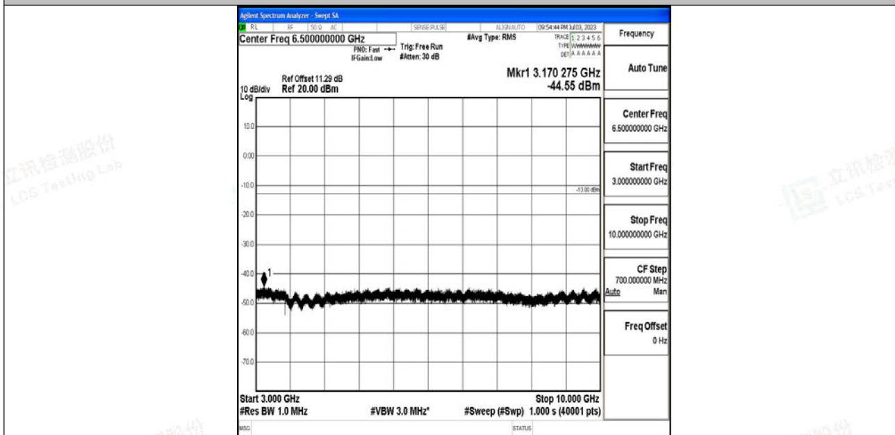
Band12_3MHz_16QAM_23095_1RB#0_3000~10000_3000~10000
