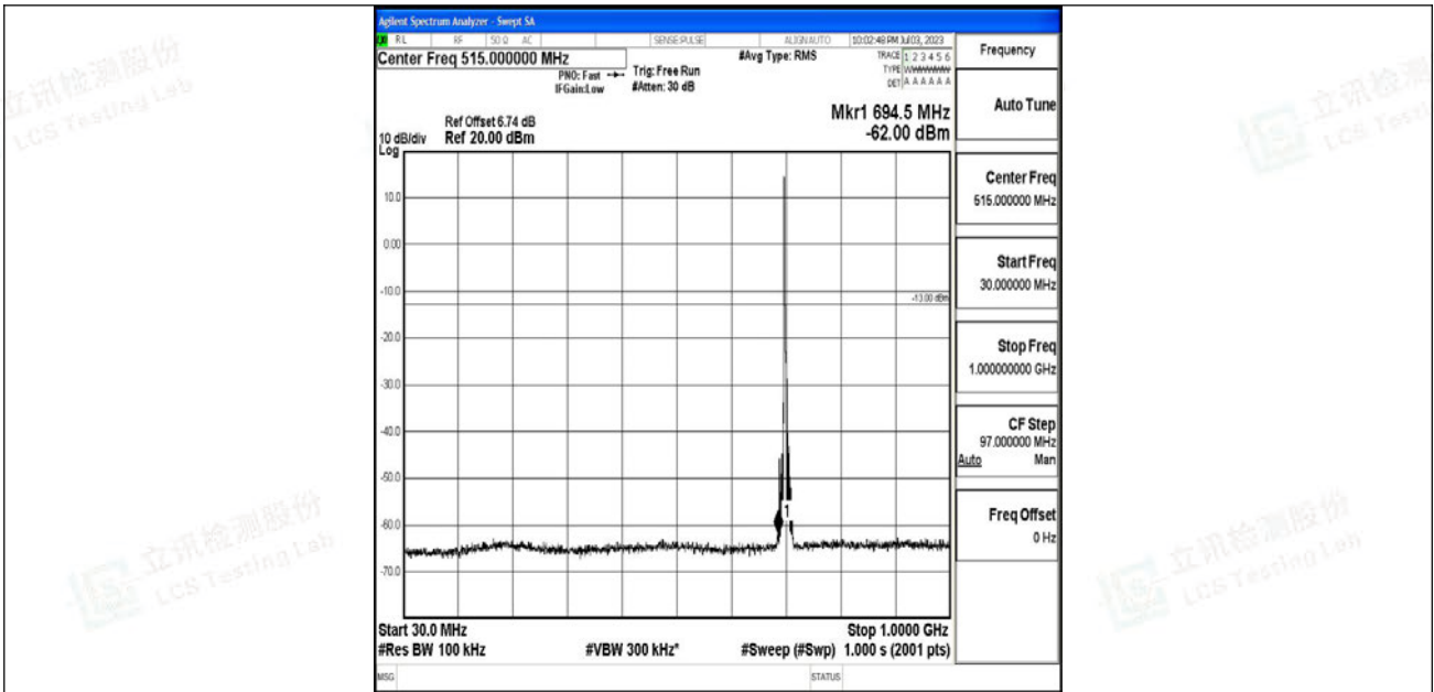
Band12_5MHz_QPSK_23095_1RB#0_30~1000_30~1000
