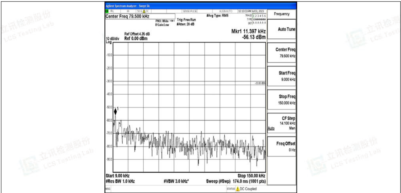
Band12_10MHz_QPSK_23095_1RB#0_0.009~0.15_0.009~0.15
