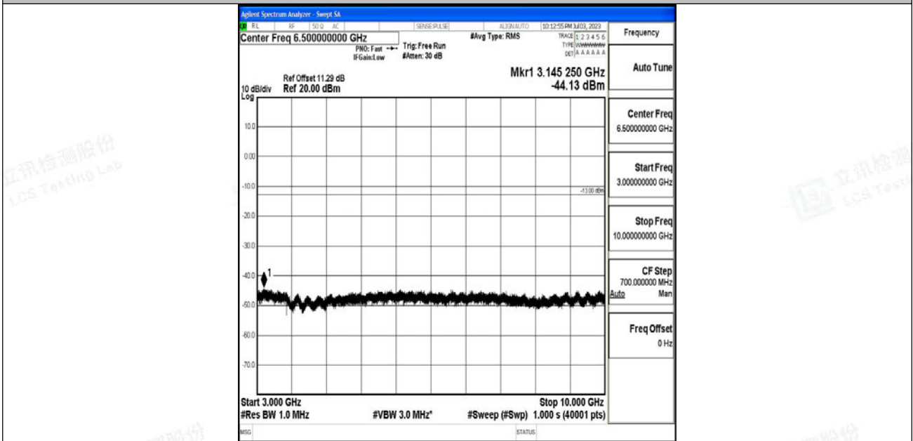
Band12_10MHz_16QAM_23130_1RB#0_3000~10000_3000~10000
