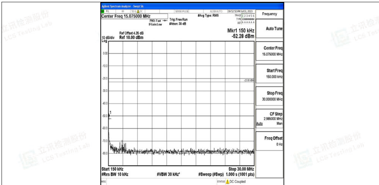
Band12_3MHz_16QAM_23025_1RB#0_0.15~30_0.15~30
