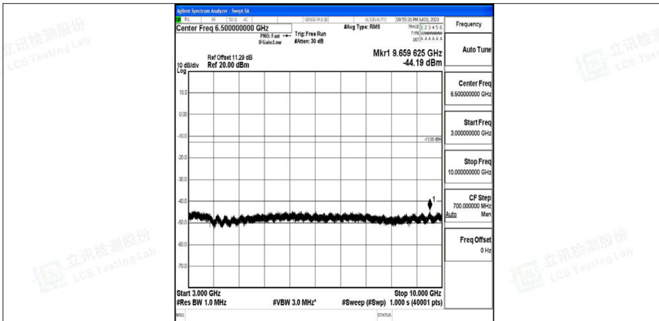
Band12_3MHz_QPSK_23165_1RB#0_3000~10000_3000~10000
