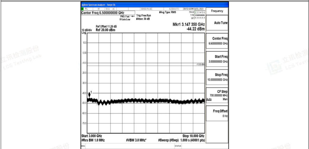
Band12_3MHz_16QAM_23025_1RB#0_3000~10000_3000~10000
