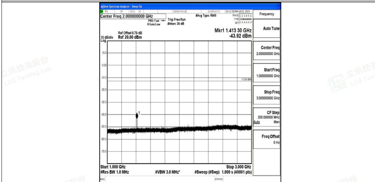
Band12_10MHz_QPSK_23130_1RB#0_1000~3000_1000~3000
