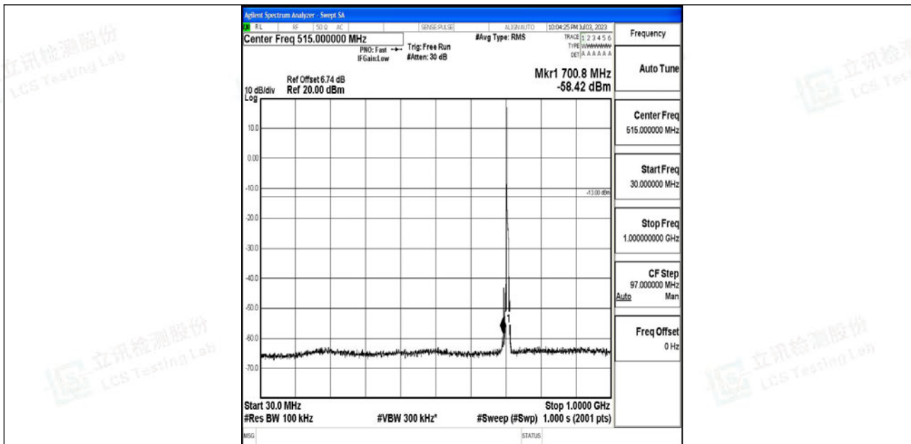
Band12_5MHz_QPSK_23155_1RB#0_30~1000_30~1000
