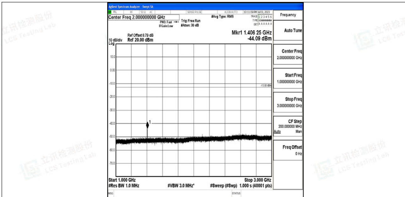
Band12_10MHz_16QAM_23095_1RB#0_1000~3000_1000~3000
