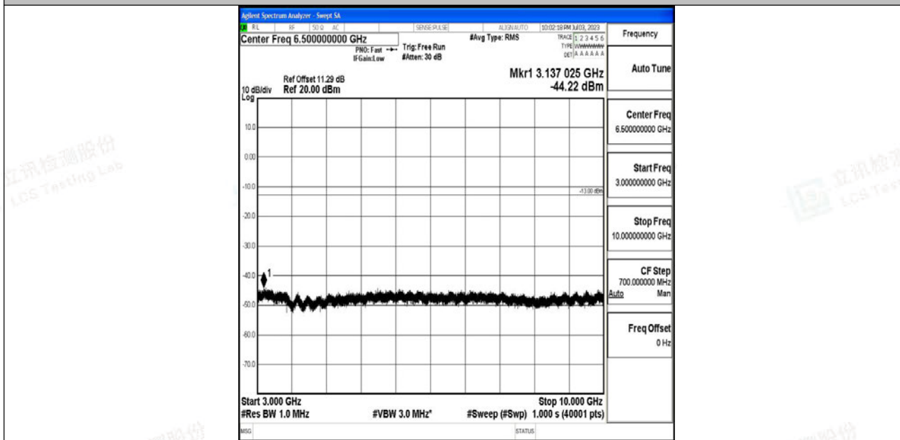
Band12_5MHz_16QAM_23035_1RB#0_3000~10000_3000~10000
