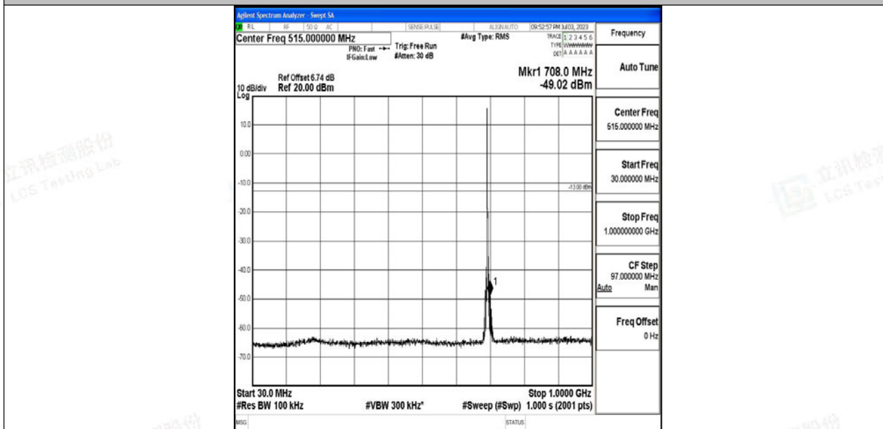
Band12_3MHz_16QAM_23025_1RB#0_30~1000_30~1000
