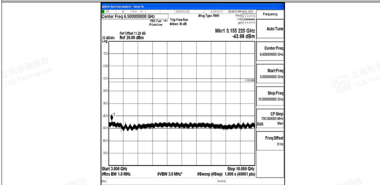
Band12_1.4MHz_16QAM_23173_1RB#0_3000~10000_3000~10000
