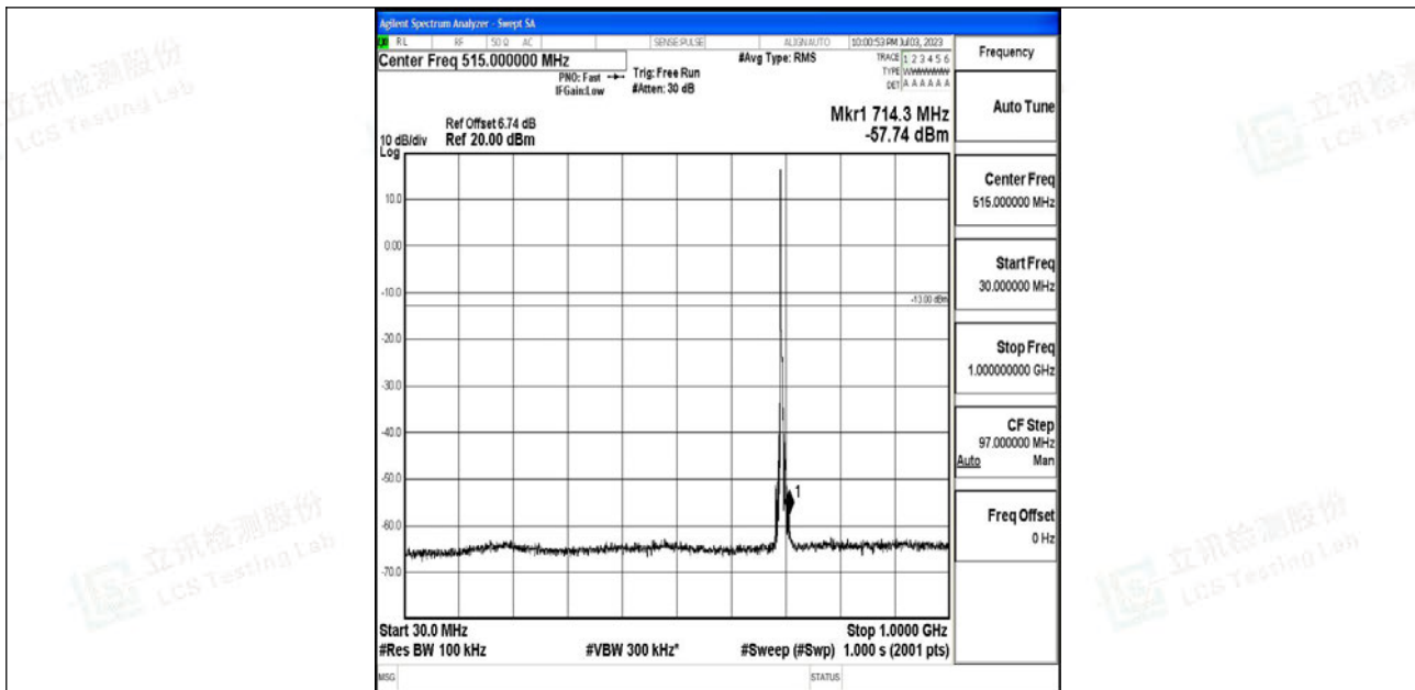
Band12_5MHz_QPSK_23035_1RB#0_30~1000_30~1000
