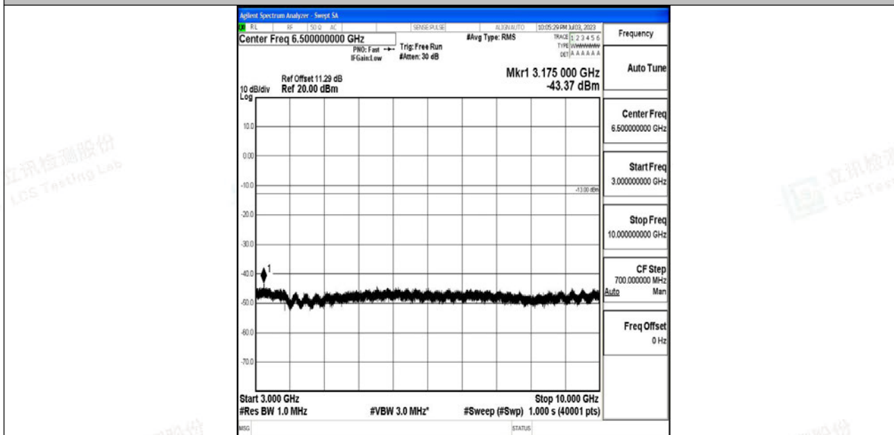
Band12_5MHz_16QAM_23155_1RB#0_3000~10000_3000~10000
