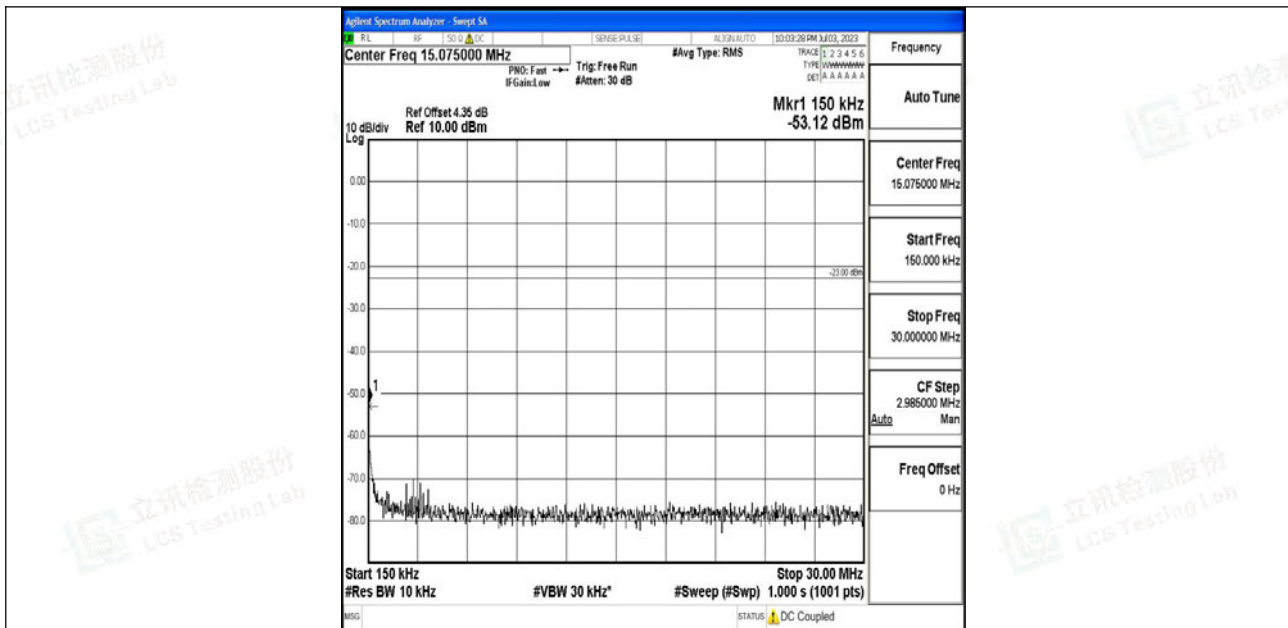
Band12_5MHz_16QAM_23095_1RB#0_0.15~30_0.15~30
