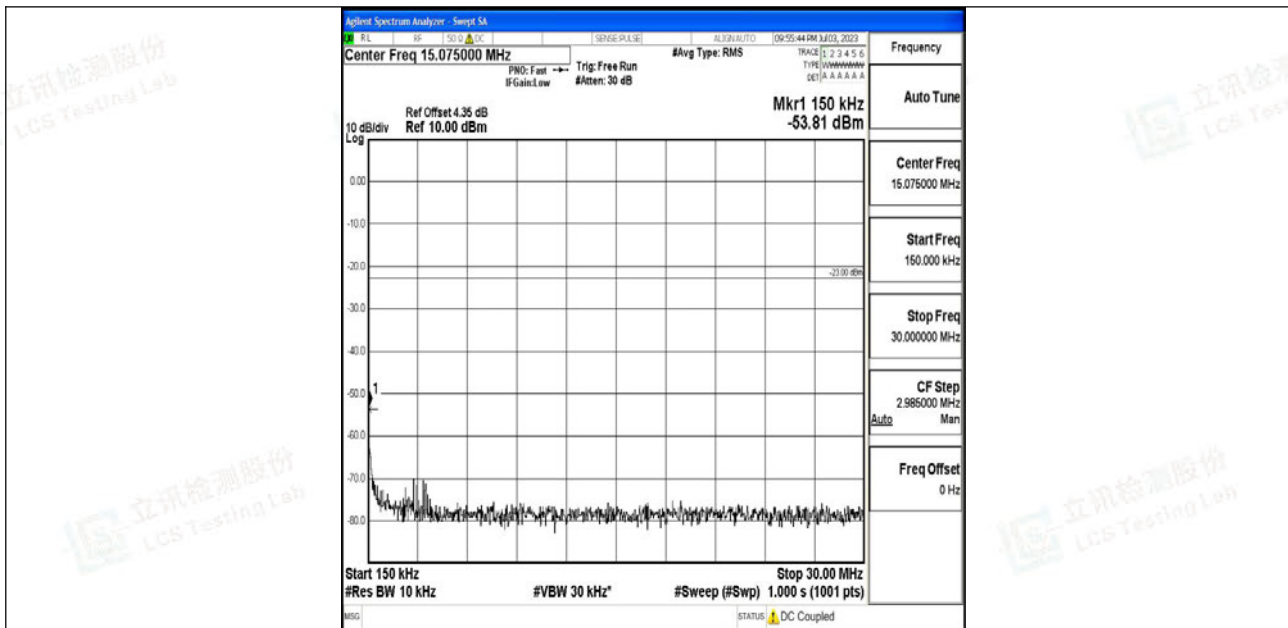
Band12_3MHz_16QAM_23165_1RB#0_0.15~30_0.15~30
