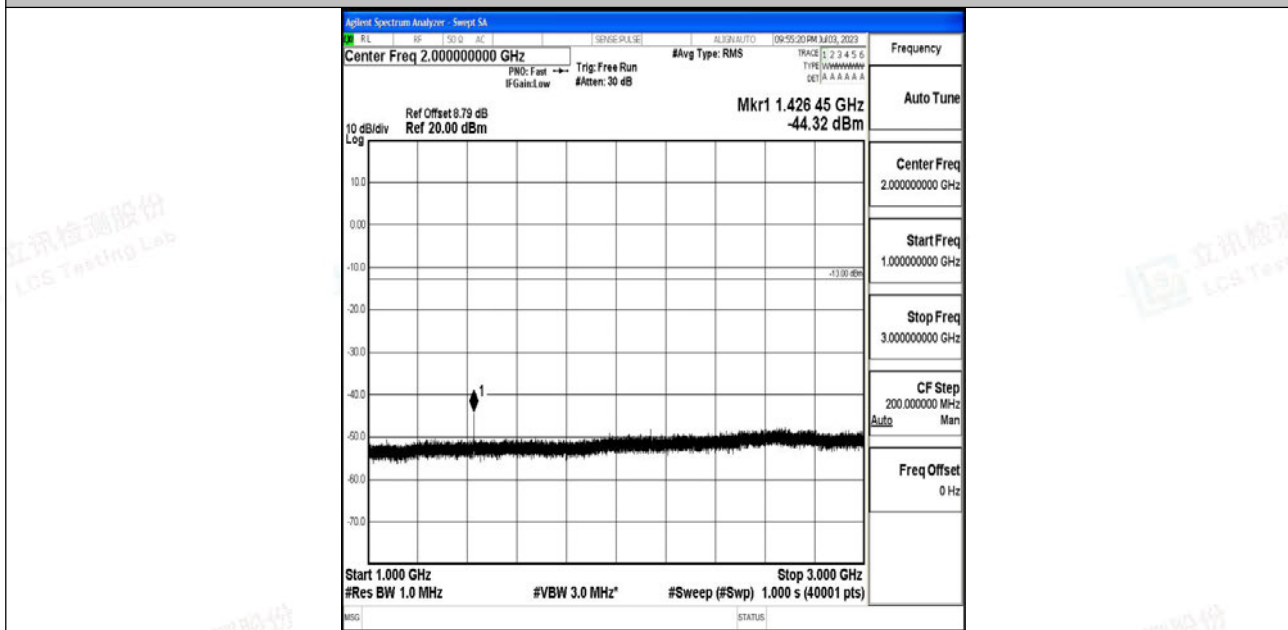
Band12_3MHz_QPSK_23165_1RB#0_1000~3000_1000~3000
