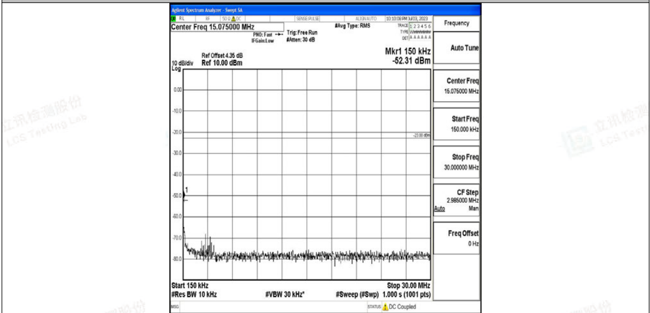
Band12_10MHz_QPSK_23095_1RB#0_0.15~30_0.15~30
