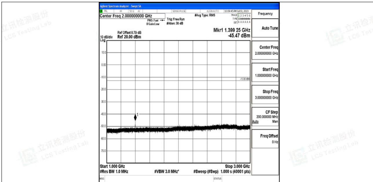
Band12_10MHz_16QAM_23060_1RB#0_1000~3000_1000~3000
