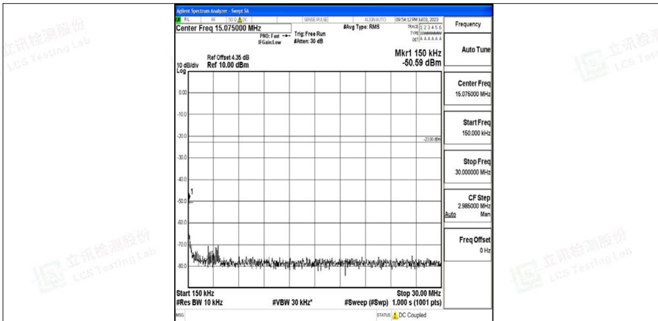
Band12_3MHz_16QAM_23095_1RB#0_0.15~30_0.15~30
