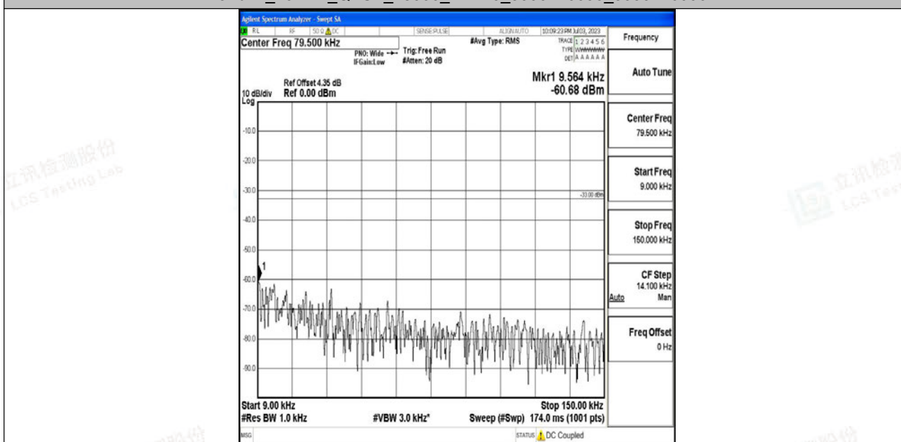
Band12_10MHz_16QAM_23060_1RB#0_0.009~0.15_0.009~0.15
