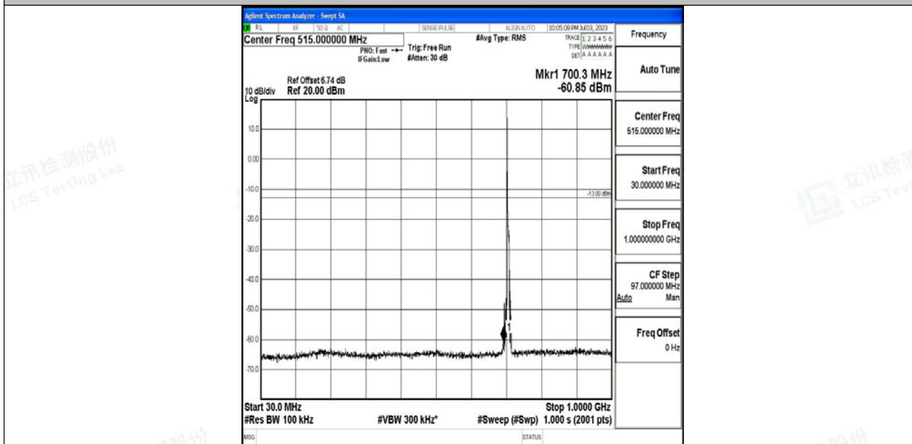
Band12_5MHz_16QAM_23155_1RB#0_30~1000_30~1000
