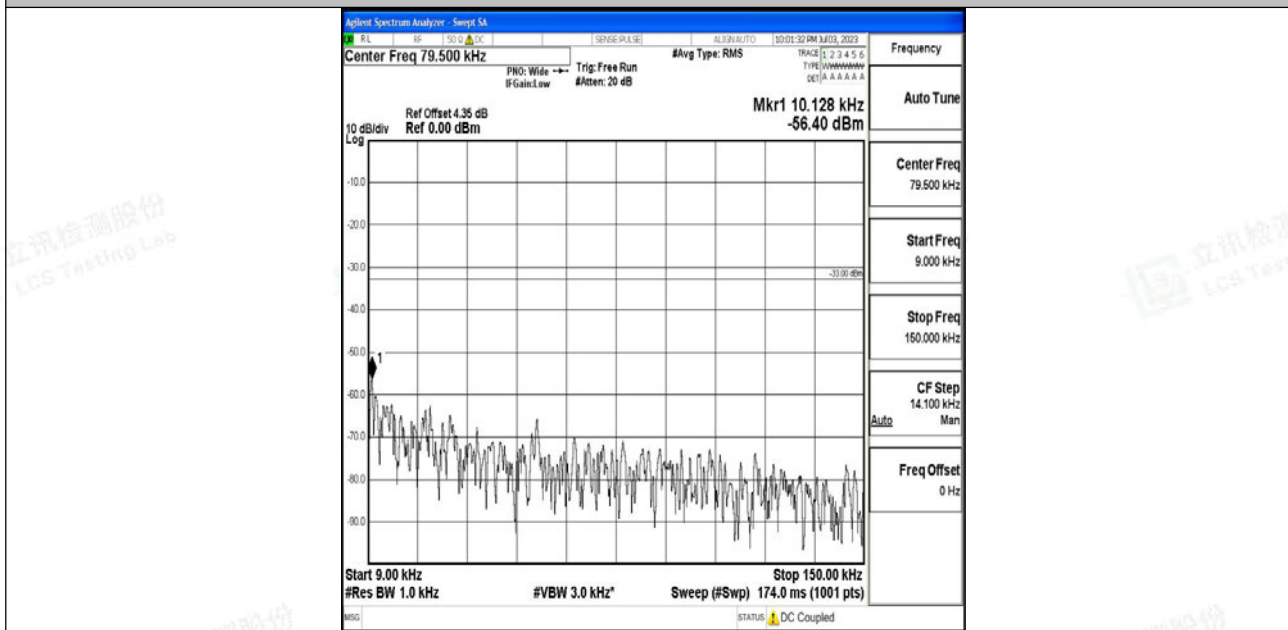
Band12_5MHz_16QAM_23035_1RB#0_0.009~0.15_0.009~0.15
