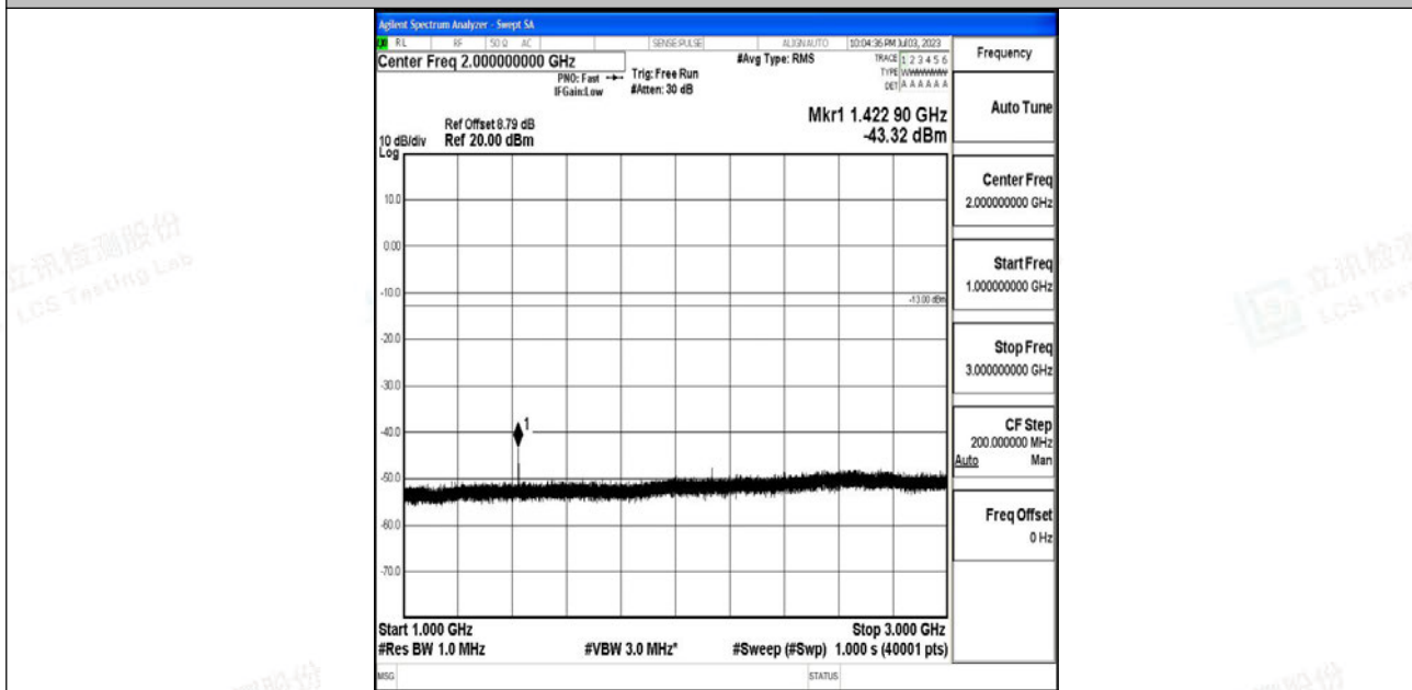
Band12_5MHz_QPSK_23155_1RB#0_1000~3000_1000~3000
