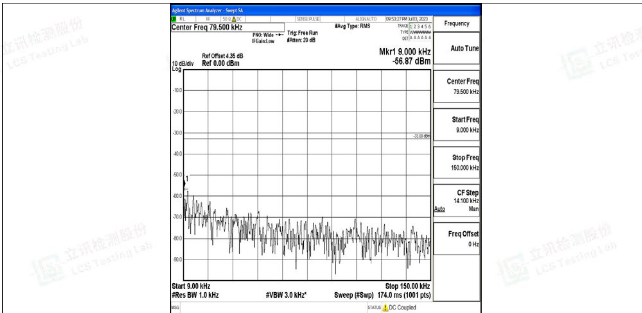
Band12_3MHz_QPSK_23095_1RB#0_0.009~0.15_0.009~0.15
