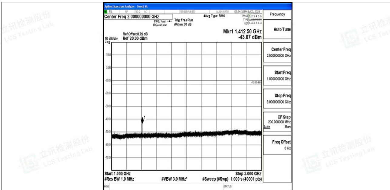
Band12_3MHz_16QAM_23095_1RB#0_1000~3000_1000~3000
