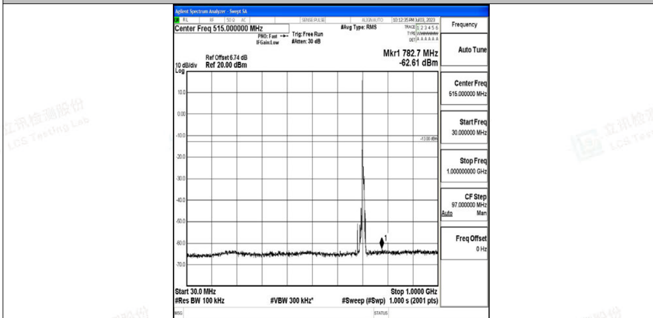
Band12_10MHz_16QAM_23130_1RB#0_30~1000_30~1000
