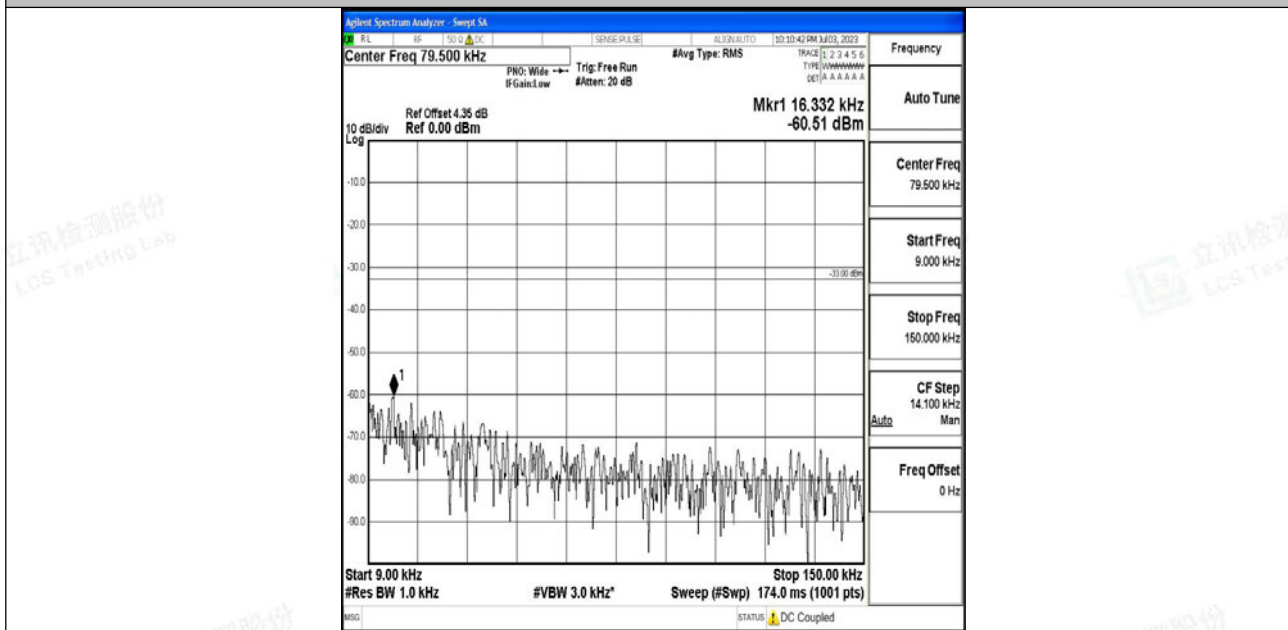
Band12_10MHz_16QAM_23095_1RB#0_0.009~0.15_0.009~0.15
