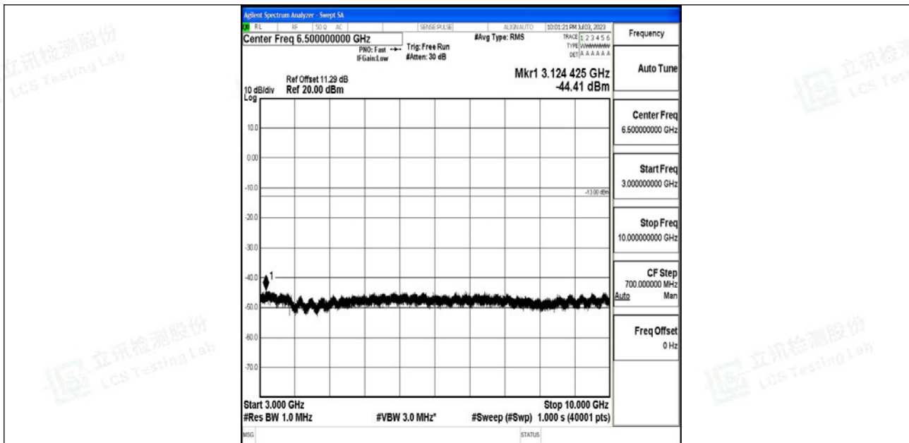
Band12_5MHz_QPSK_23035_1RB#0_3000~10000_3000~10000
