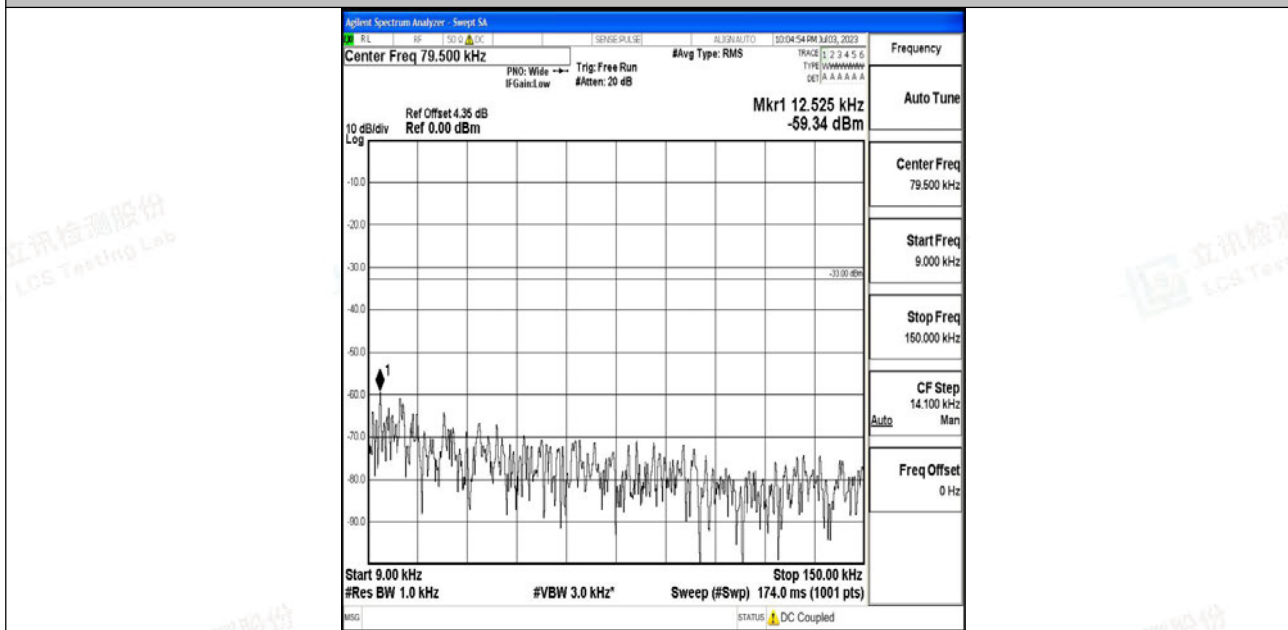
Band12_5MHz_16QAM_23155_1RB#0_0.009~0.15_0.009~0.15
