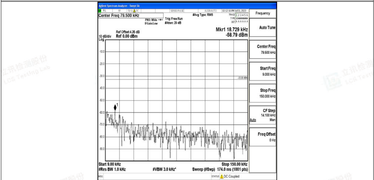
Band12_10MHz_16QAM_23130_1RB#0_0.009~0.15_0.009~0.15
