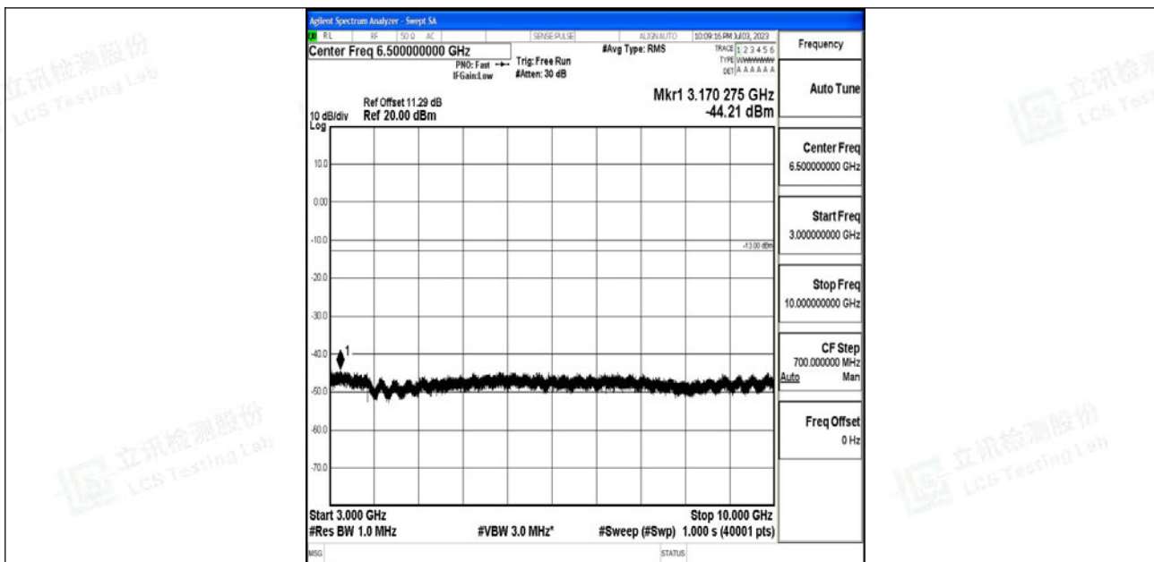
Band12_10MHz_QPSK_23060_1RB#0_3000~10000_3000~10000
