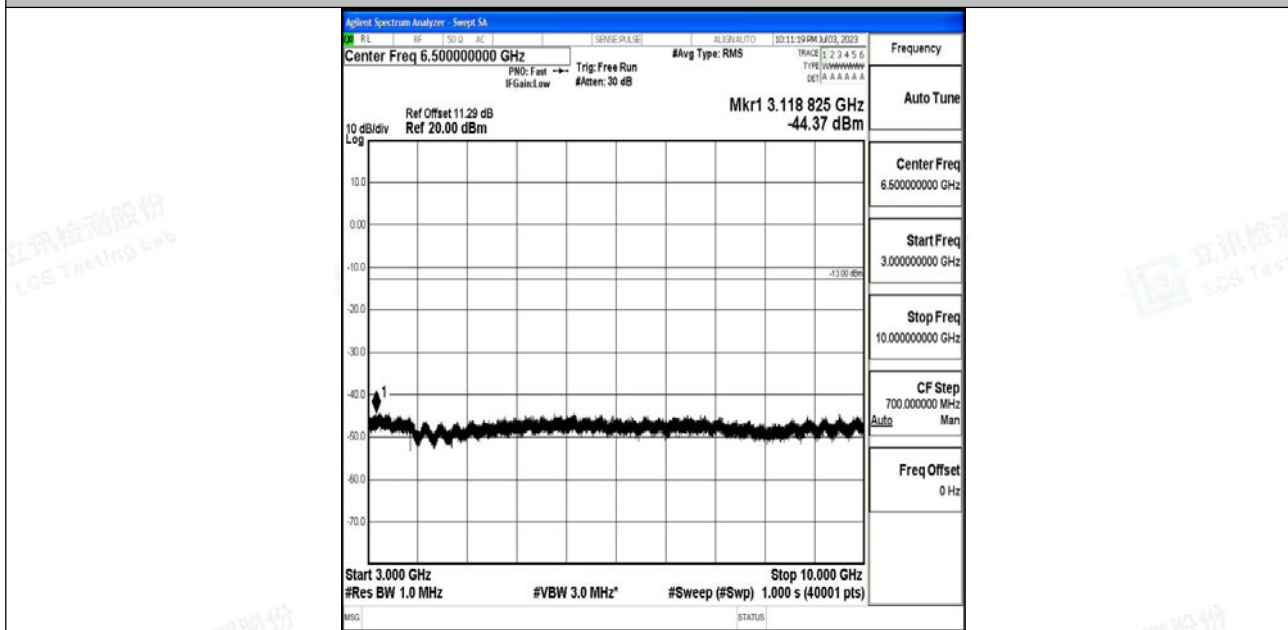
Band12_10MHz_16QAM_23095_1RB#0_3000~10000_3000~10000
