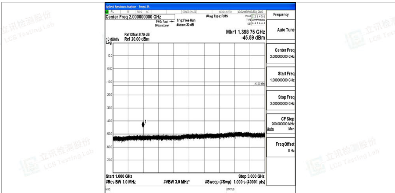
Band12_5MHz_16QAM_23035_1RB#0_1000~3000_1000~3000
