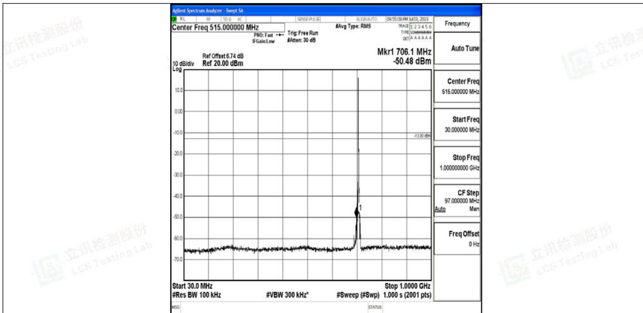
Band12_3MHz_QPSK_23165_1RB#0_30~1000_30~1000
