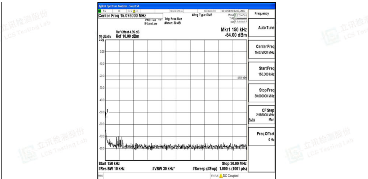
Band12_10MHz_16QAM_23095_1RB#0_0.15~30_0.15~30
