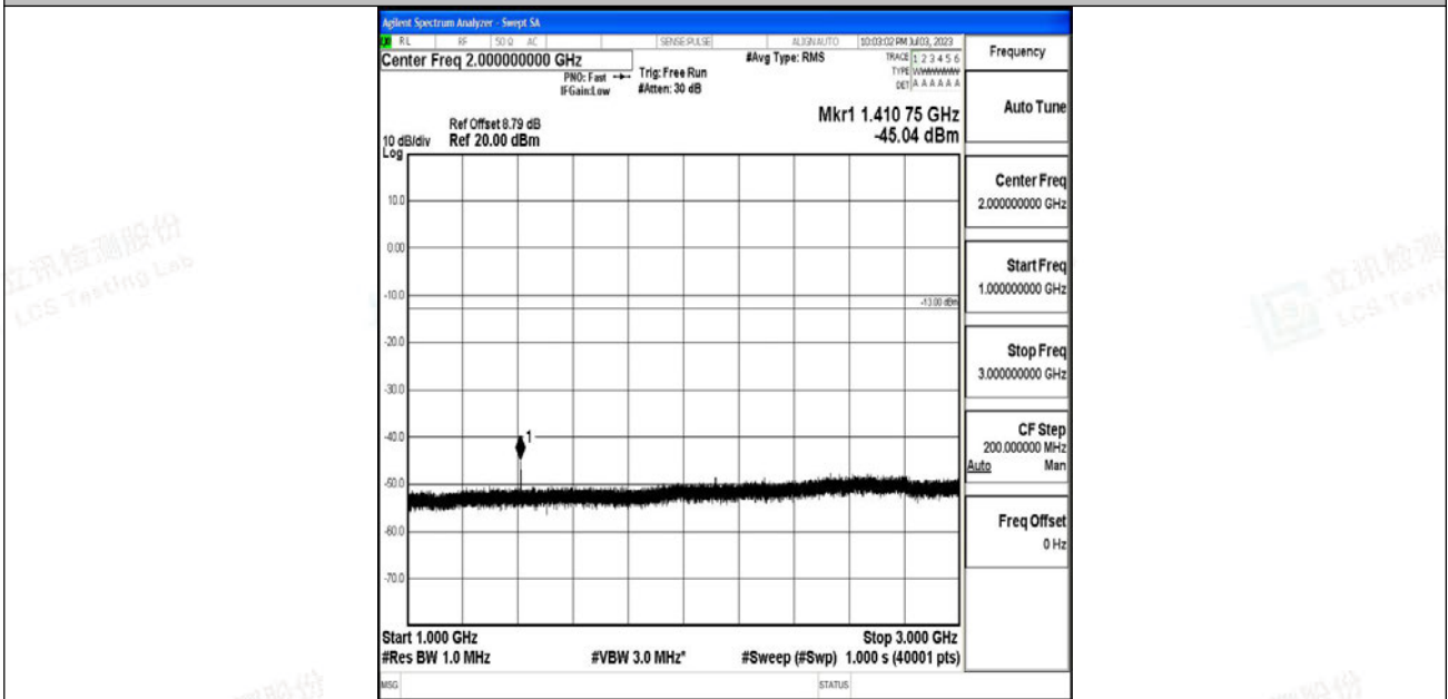
Band12_5MHz_QPSK_23095_1RB#0_1000~3000_1000~3000
