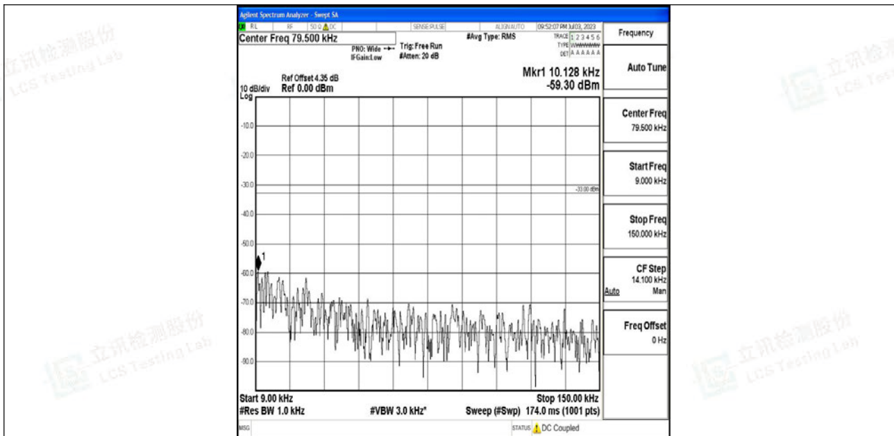
Band12_3MHz_QPSK_23025_1RB#0_0.009~0.15_0.009~0.15
