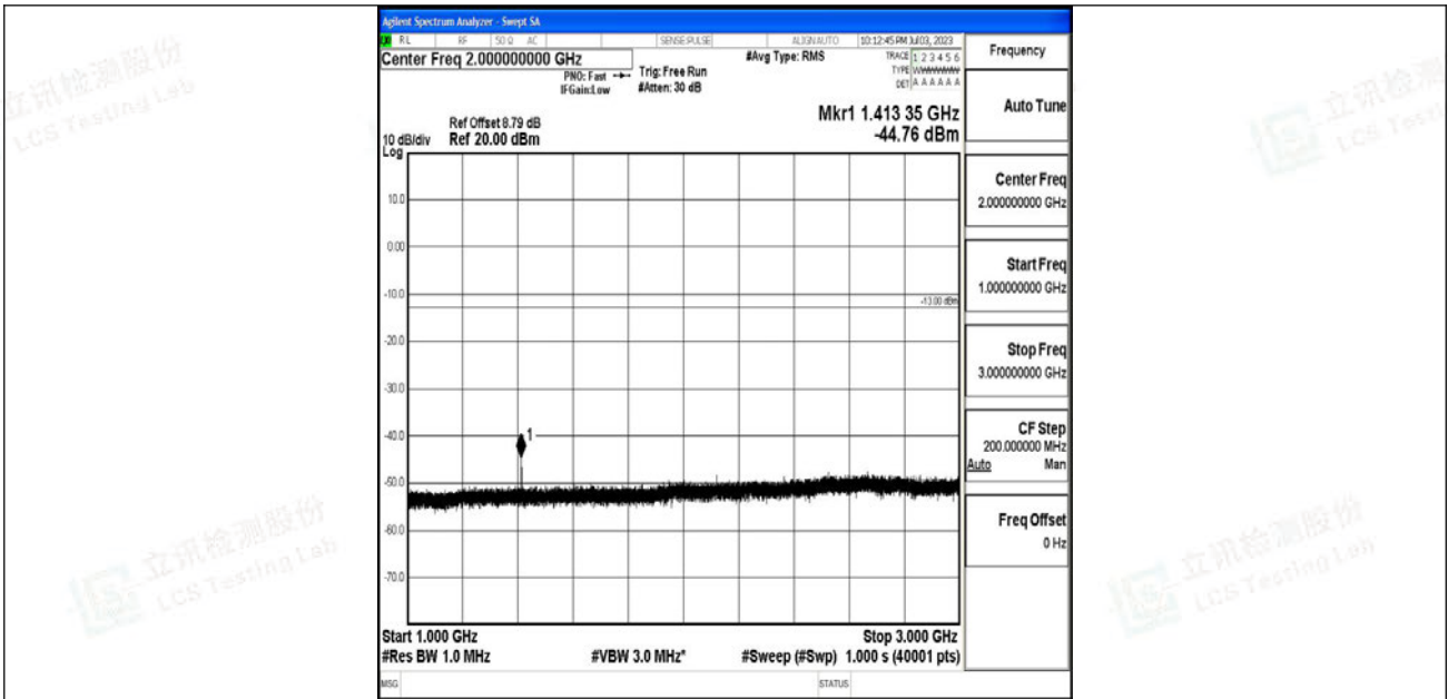
Band12_10MHz_16QAM_23130_1RB#0_1000~3000_1000~3000
