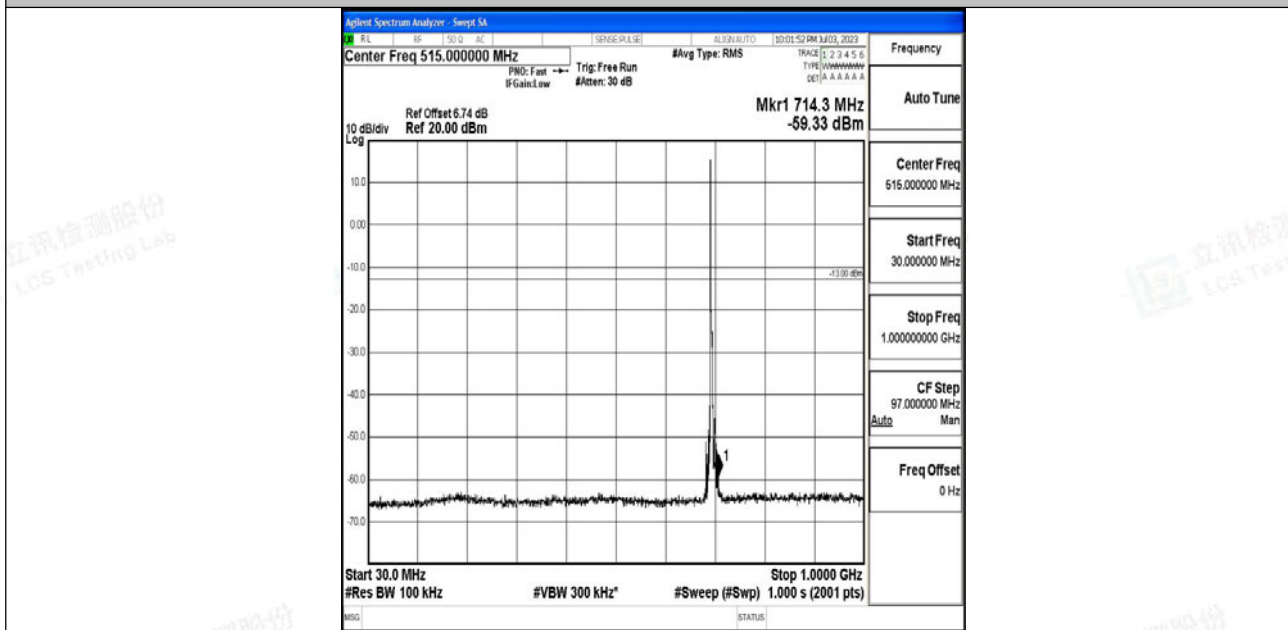
Band12_5MHz_16QAM_23035_1RB#0_30~1000_30~1000
