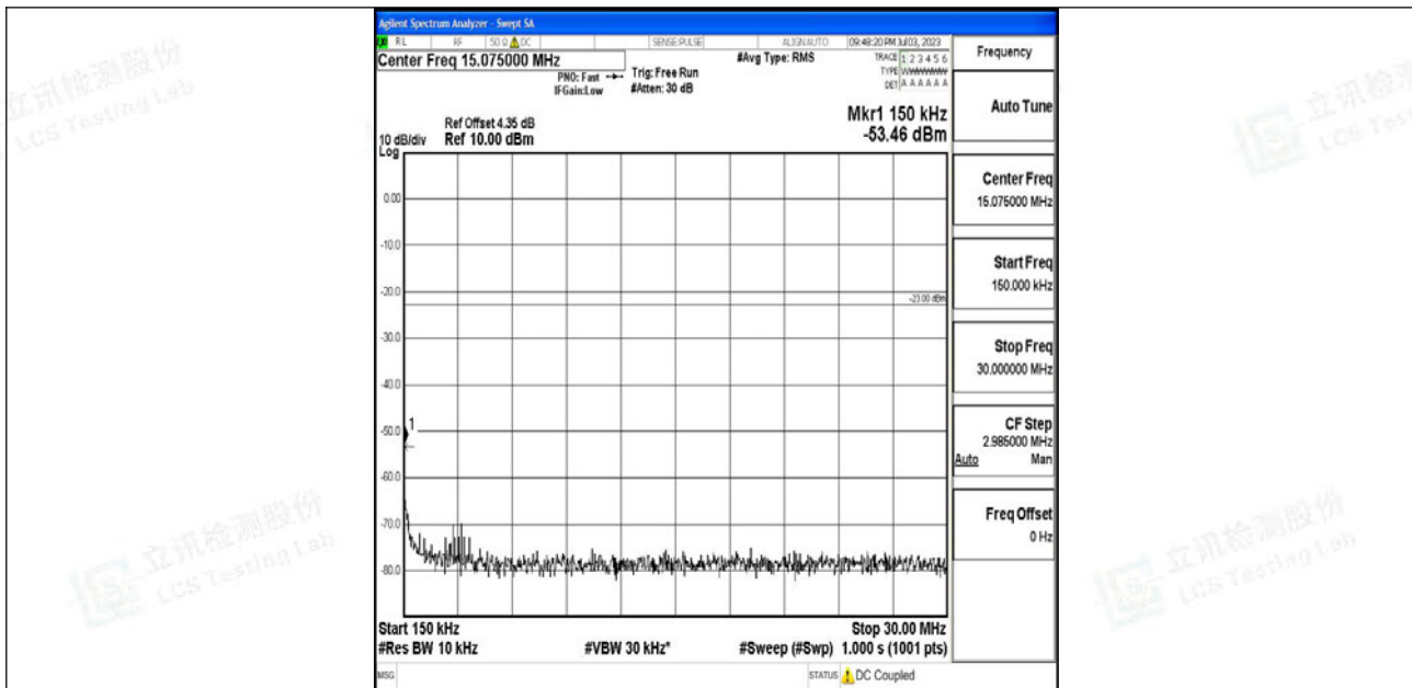
Band12_1.4MHz_16QAM_23173_1RB#0_0.15~30_0.15~30
