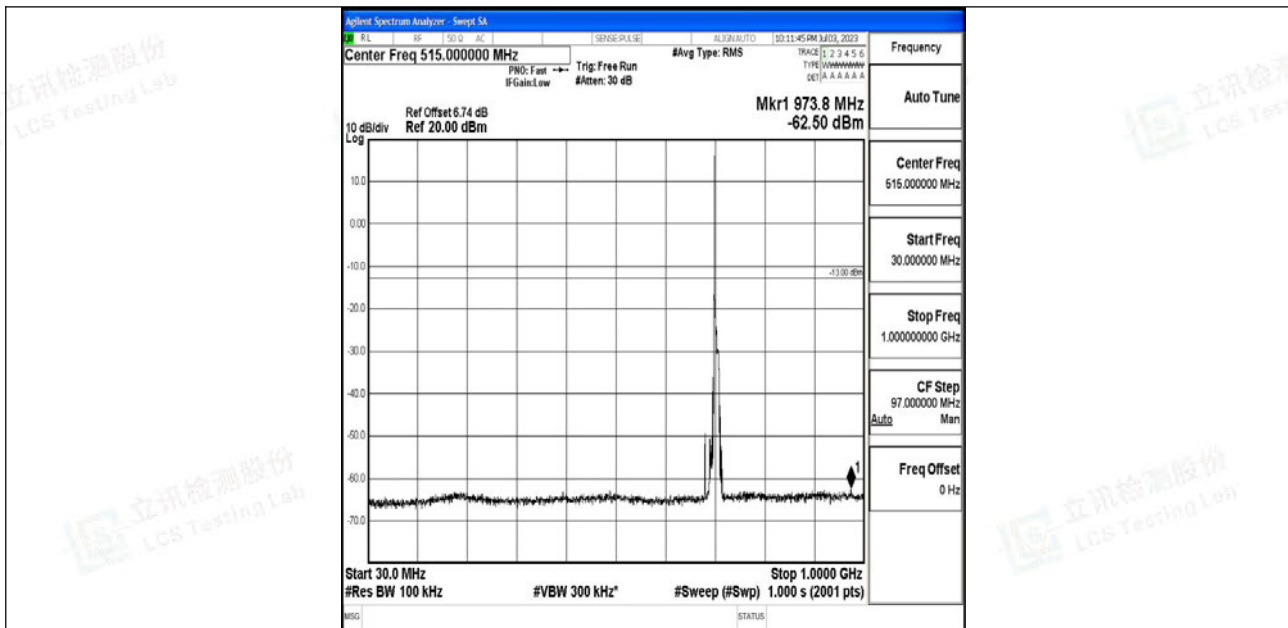
Band12_10MHz_QPSK_23130_1RB#0_30~1000_30~1000
