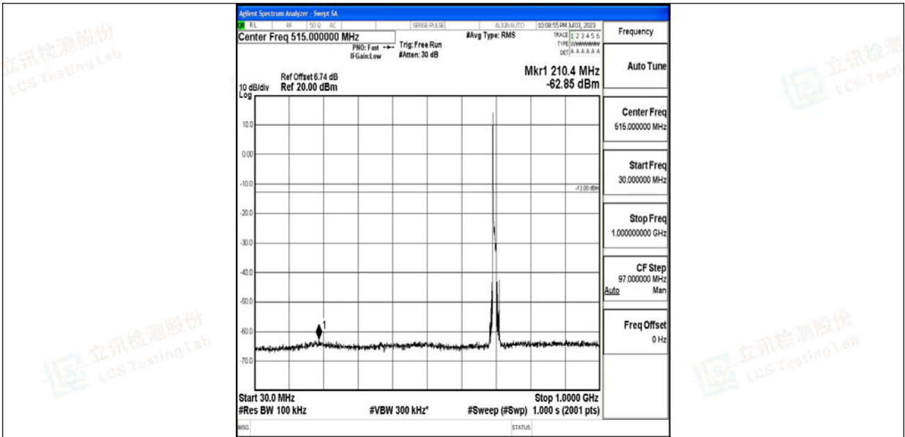
Band12_10MHz_QPSK_23060_1RB#0_30~1000_30~1000
