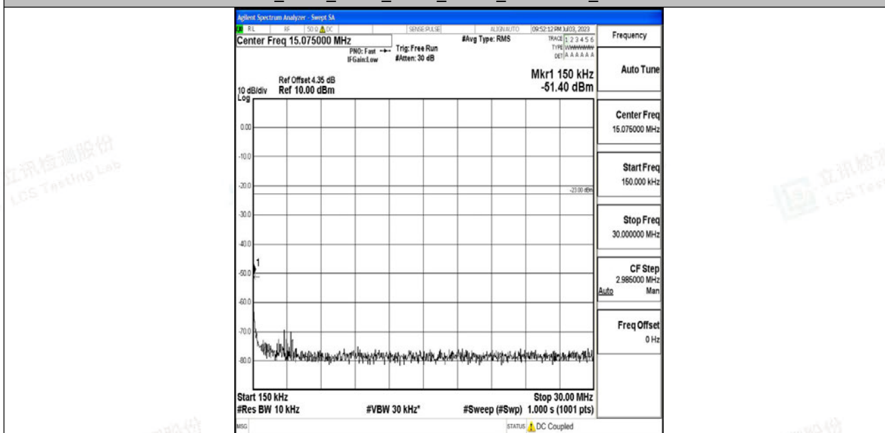
Band12_3MHz_QPSK_23025_1RB#0_0.15~30_0.15~30
