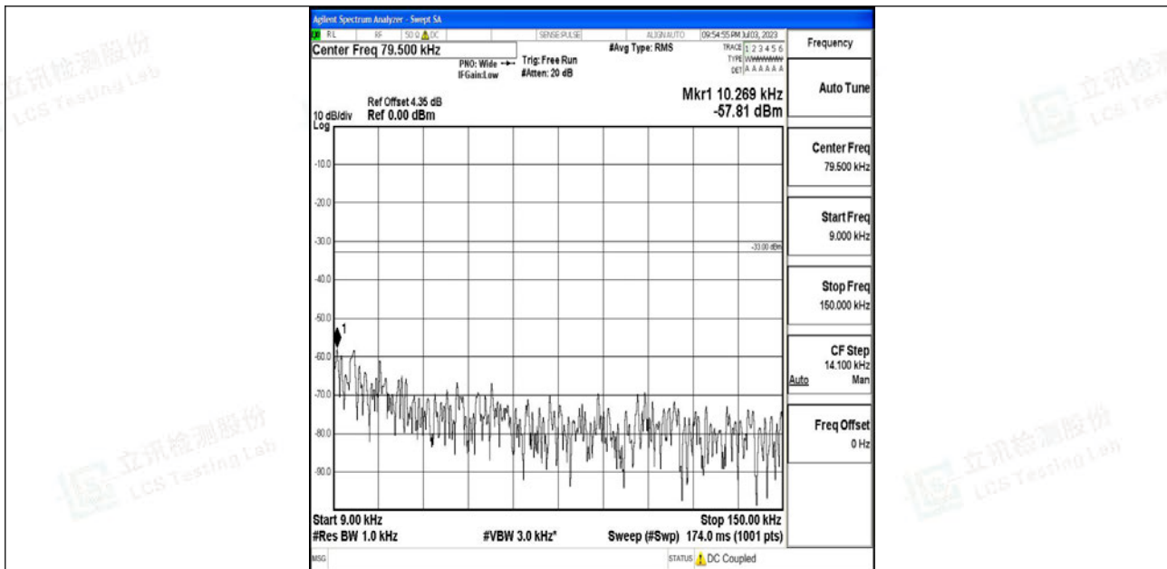
Band12_3MHz_QPSK_23165_1RB#0_0.009~0.15_0.009~0.15
