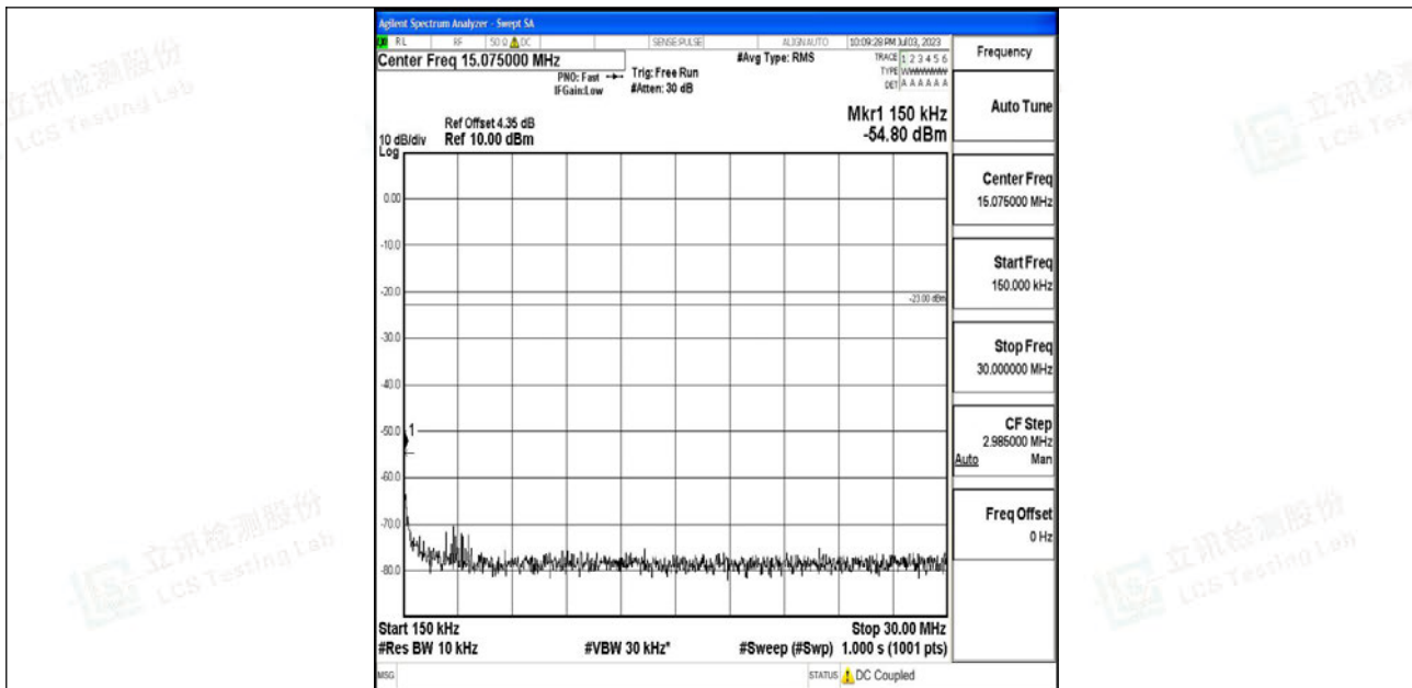
Band12_10MHz_16QAM_23060_1RB#0_0.15~30_0.15~30
