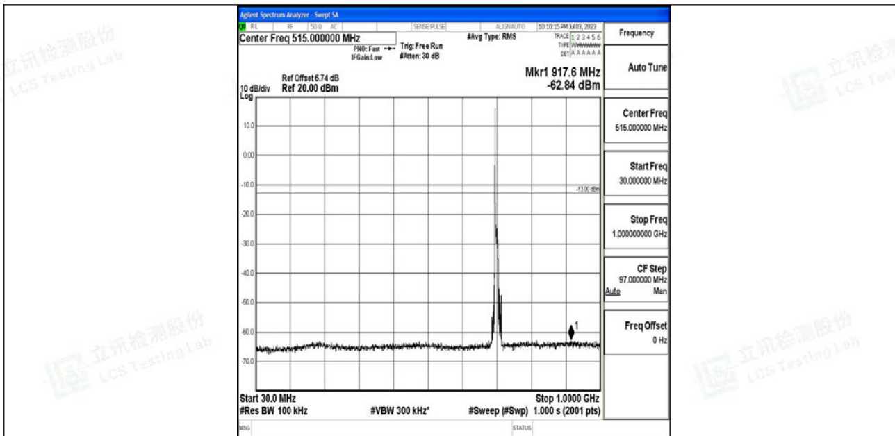
Band12_10MHz_QPSK_23095_1RB#0_30~1000_30~1000
