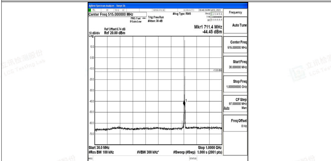
Band12_1.4MHz_16QAM_23173_1RB#0_30~1000_30~1000
