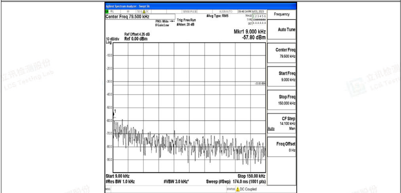
Band12_1.4MHz_16QAM_23173_1RB#0_0.009~0.15_0.009~0.15
