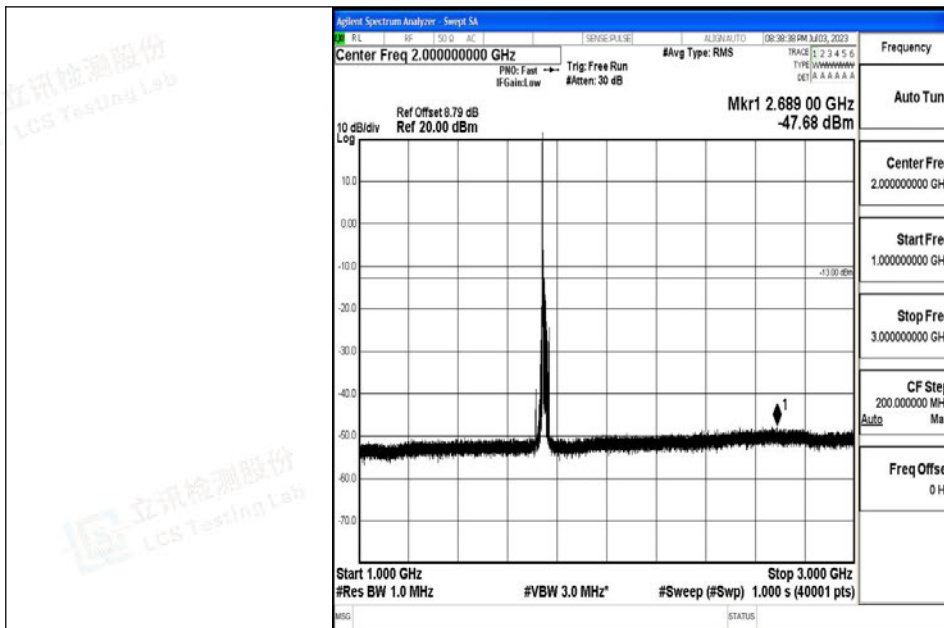
Band4_15MHz_QPSK_20325_1RB#0_1000~3000_1000~3000
