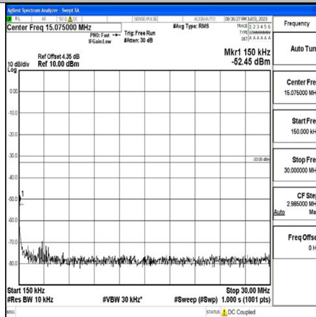
Band4_15MHz_16QAM_20025_1RB#0_0.15~30_0.15~30
