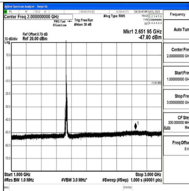
Band4_10MHz_QPSK_20175_1RB#0_1000~3000_1000~3000
