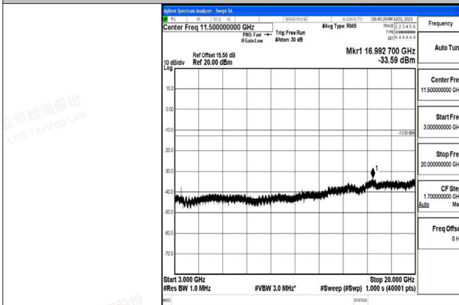
Band4_20MHz_QPSK_20300_1RB#0_3000~20000_3000~20000
