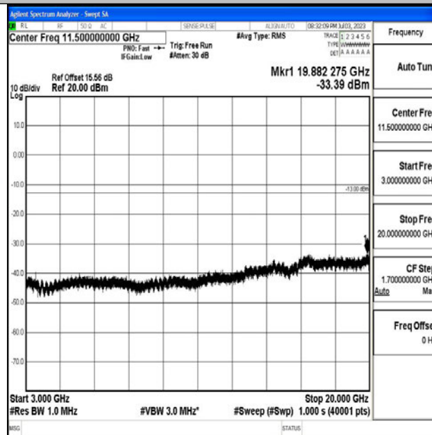
Band4_10MHz_QPSK_20350_1RB#0_3000~20000_3000~20000
