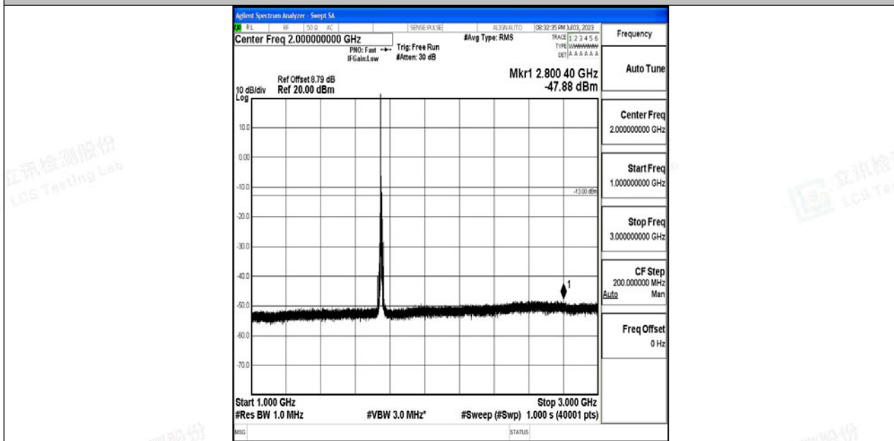
Band4_10MHz_16QAM_20350_1RB#0_1000~3000_1000~3000
