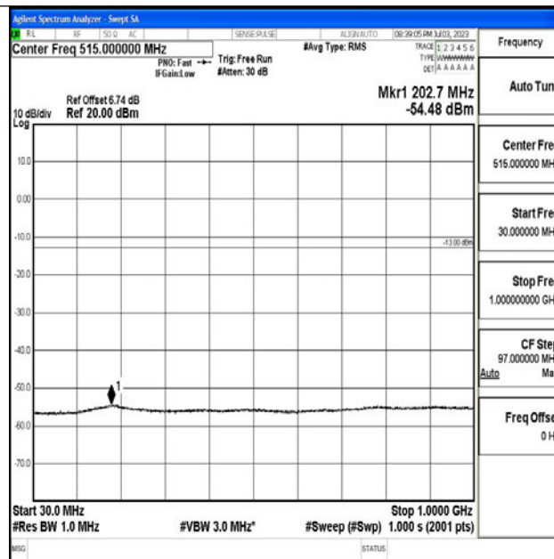
Band4_15MHz_16QAM_20325_1RB#0_30~1000_30~1000
