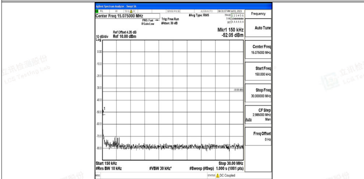
Band4_10MHz_16QAM_20175_1RB#0_0.15~30_0.15~30
