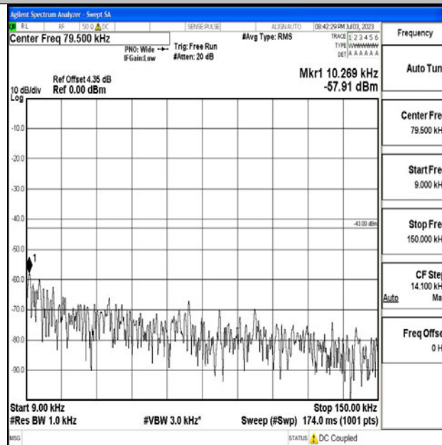
Band4_20MHz_QPSK_20050_1RB#0_0.009~0.15_0.009~0.15
