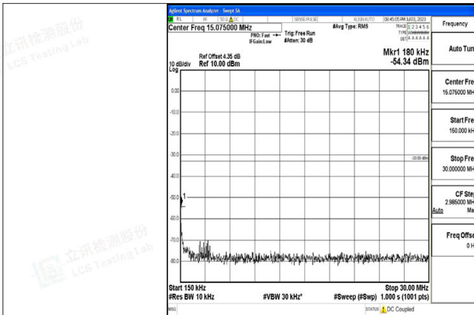
Band4_20MHz_QPSK_20300_1RB#0_0.15~30_0.15~30
