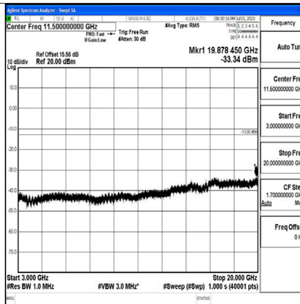
Band4_10MHz_16QAM_20000_1RB#0_3000~20000_3000~20000
