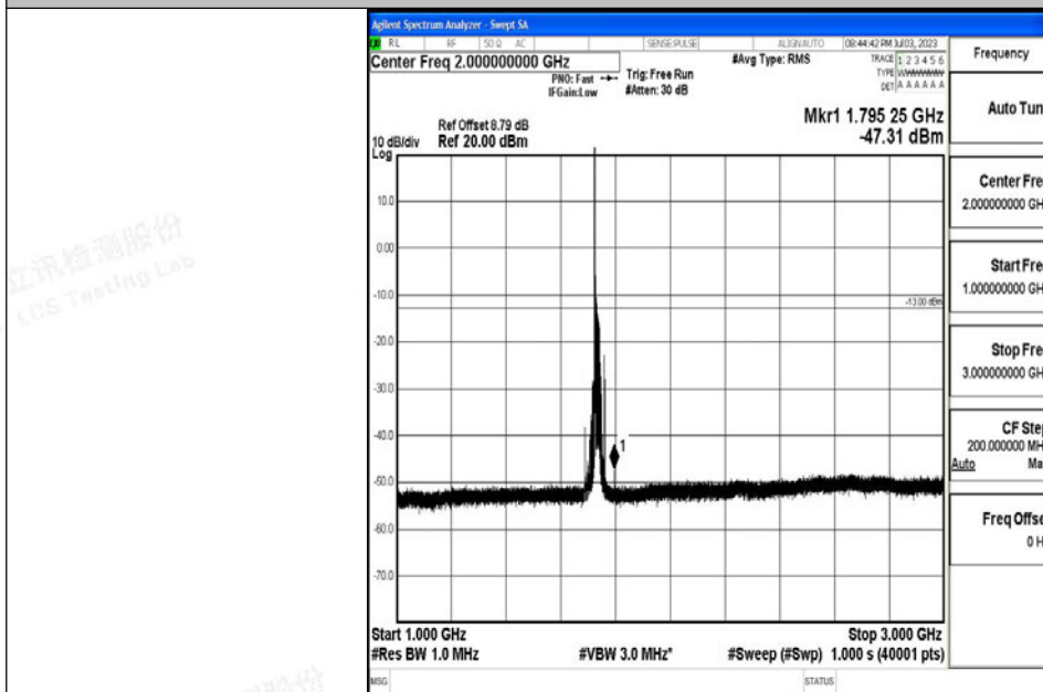
Band4_20MHz_16QAM_20175_1RB#0_1000~3000_1000~3000
