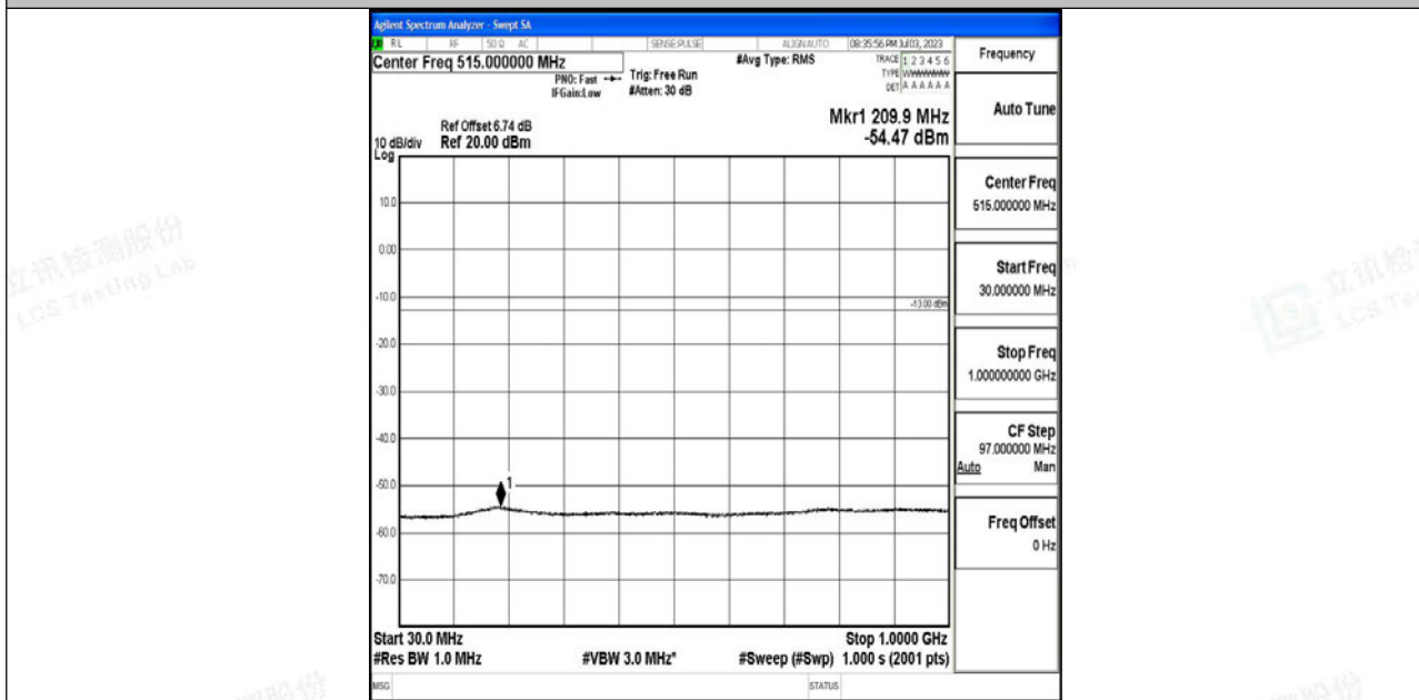
Band4_15MHz_QPSK_20025_1RB#0_30~1000_30~1000
