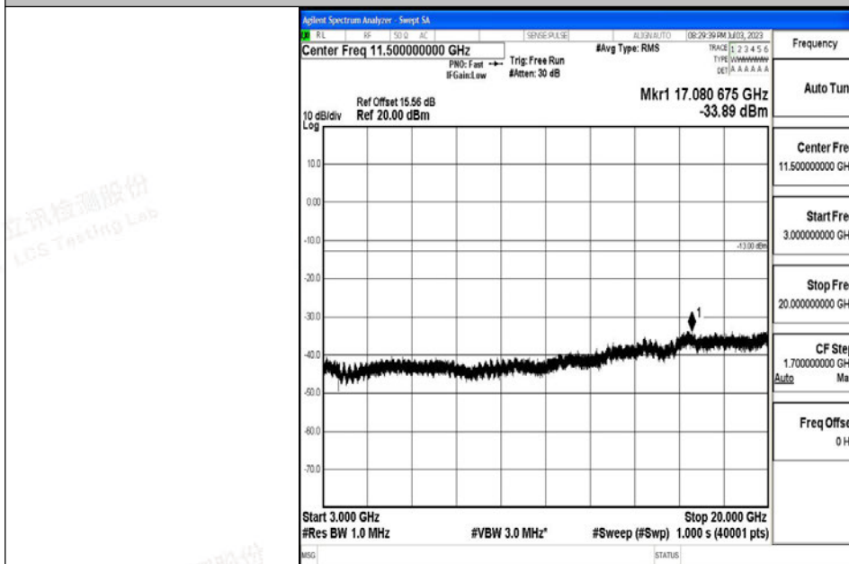
Band4_10MHz_QPSK_20000_1RB#0_3000~20000_3000~20000
