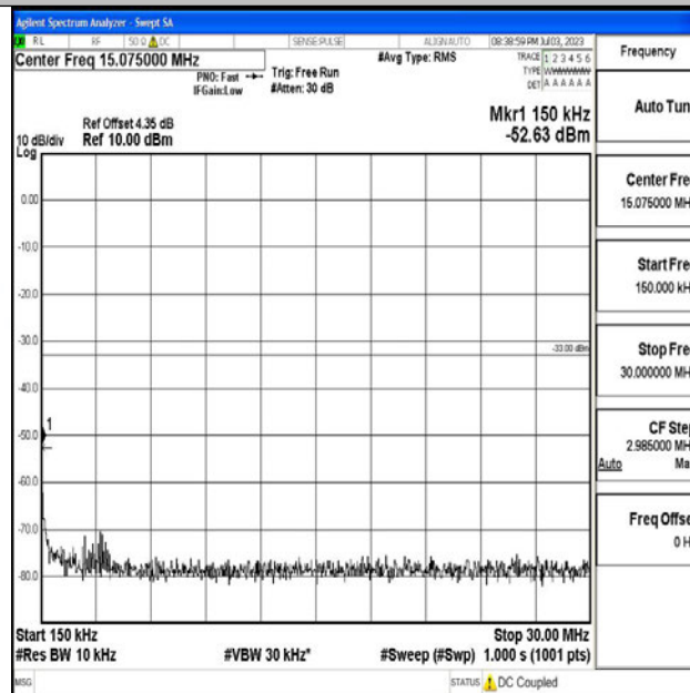
Band4_15MHz_16QAM_20325_1RB#0_0.15~30_0.15~30
