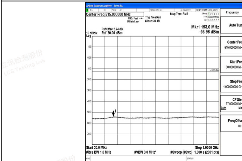
Band4_20MHz_QPSK_20300_1RB#0_30~1000_30~1000
