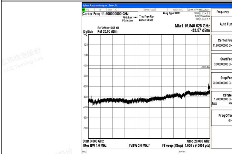
Band4_20MHz_QPSK_20175_1RB#0_3000~20000_3000~20000
