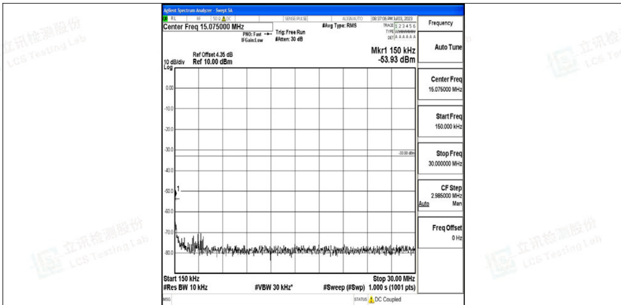
Band4_15MHz_QPSK_20175_1RB#0_0.15~30_0.15~30
