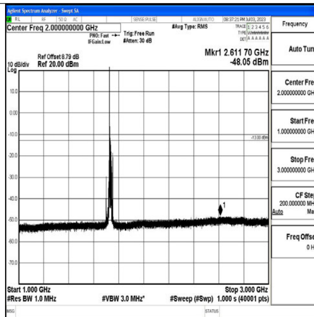
Band4_15MHz_QPSK_20175_1RB#0_1000~3000_1000~3000
