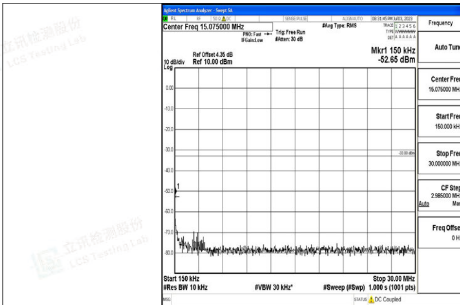
Band4_10MHz_QPSK_20350_1RB#0_0.15~30_0.15~30
