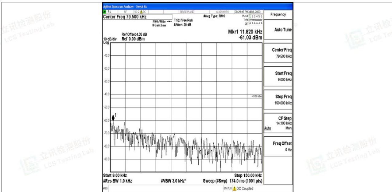
Band4_10MHz_16QAM_20000_1RB#0_0.009~0.15_0.009~0.15
