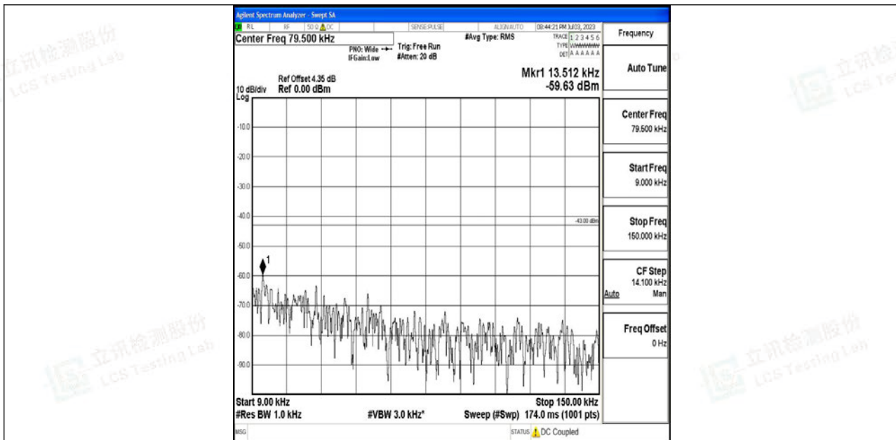
Band4_20MHz_16QAM_20175_1RB#0_0.009~0.15_0.009~0.15
