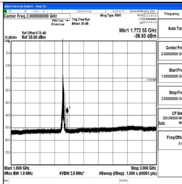
Band4_20MHz_QPSK_20050_1RB#0_1000~3000_1000~3000
