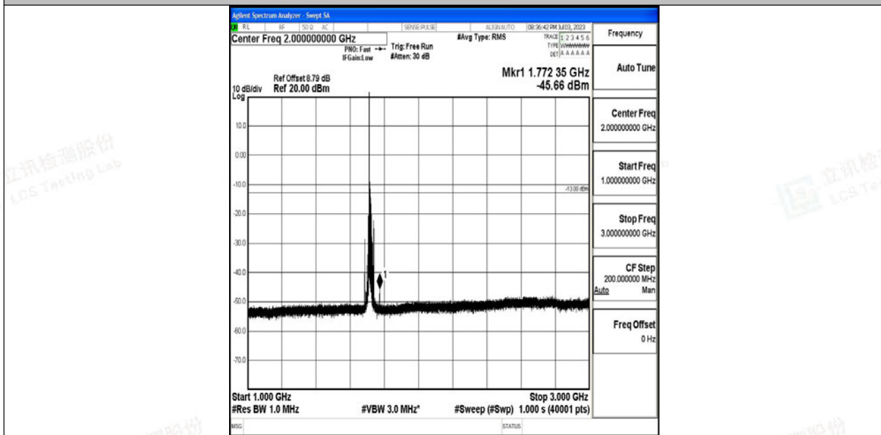
Band4_15MHz_16QAM_20025_1RB#0_1000~3000_1000~3000
