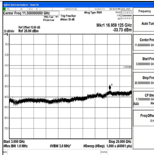
Band4_15MHz_16QAM_20325_1RB#0_3000~20000_3000~20000
