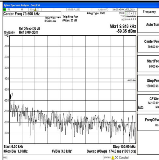
Band4_15MHz_QPSK_20025_1RB#0_0.009~0.15_0.009~0.15
