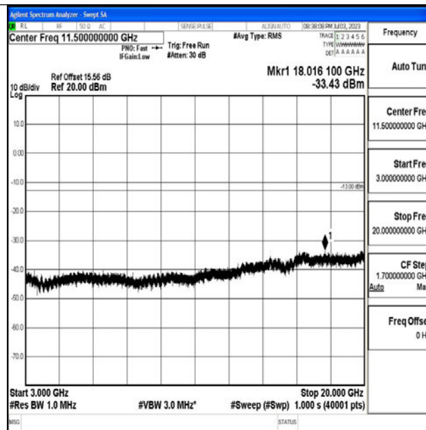
Band4_15MHz_16QAM_20175_1RB#0_3000~20000_3000~20000
