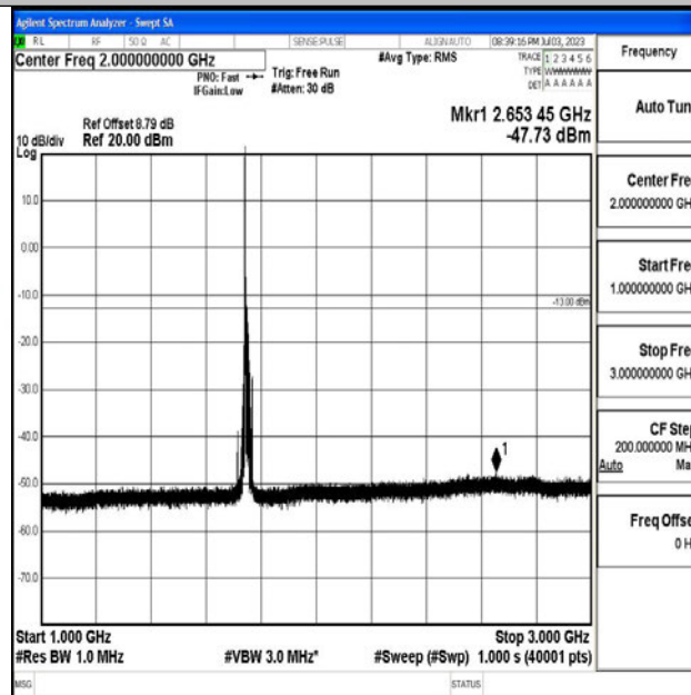
Band4_15MHz_16QAM_20325_1RB#0_1000~3000_1000~3000
