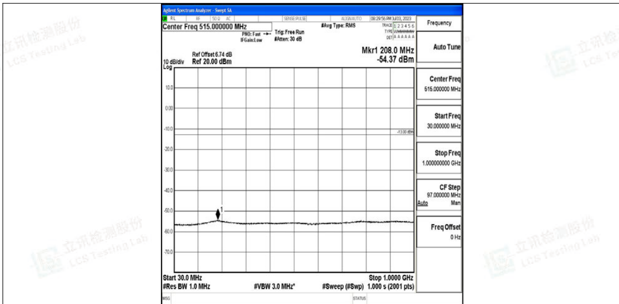
Band4_10MHz_16QAM_20000_1RB#0_30~1000_30~1000
