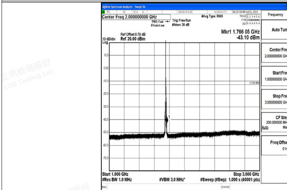
Band4_5MHz_16QAM_20375_1RB#0_1000~3000_1000~3000
