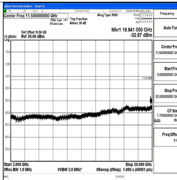
Band4_20MHz_16QAM_20050_1RB#0_3000~20000_3000~20000
