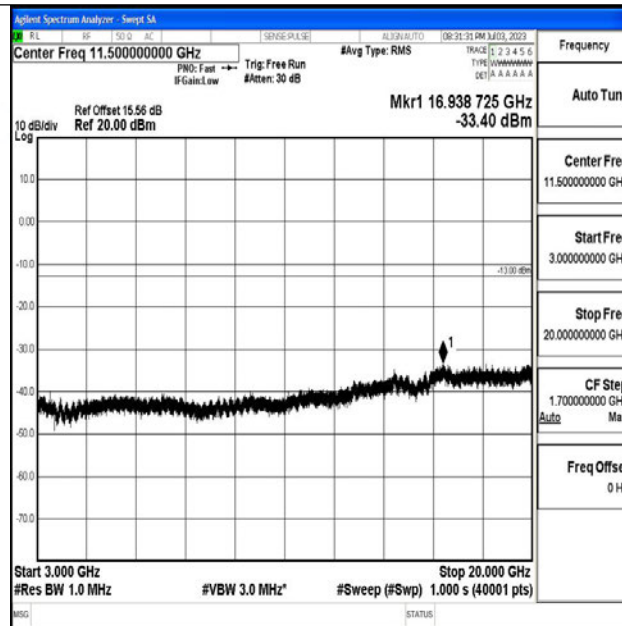
Band4_10MHz_16QAM_20175_1RB#0_3000~20000_3000~20000
