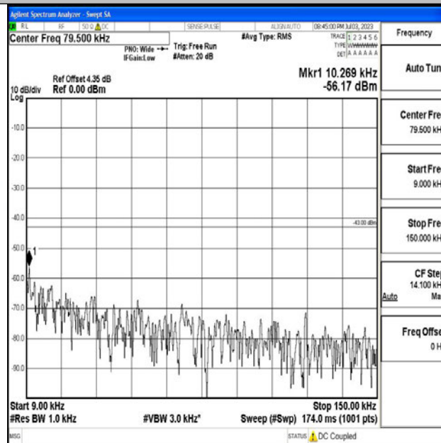
Band4_20MHz_QPSK_20300_1RB#0_0.009~0.15_0.009~0.15
