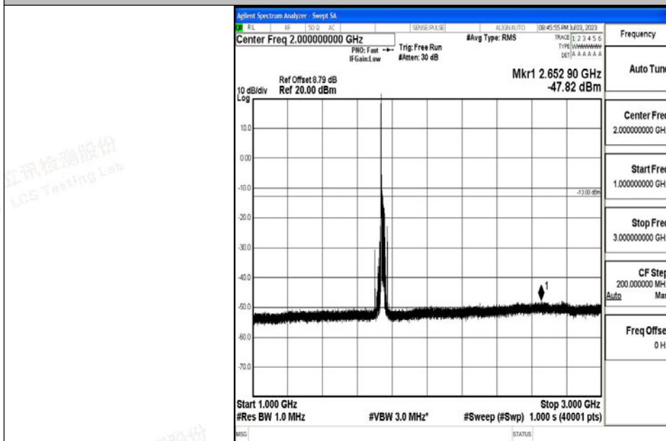
Band4_20MHz_16QAM_20300_1RB#0_1000~3000_1000~3000
