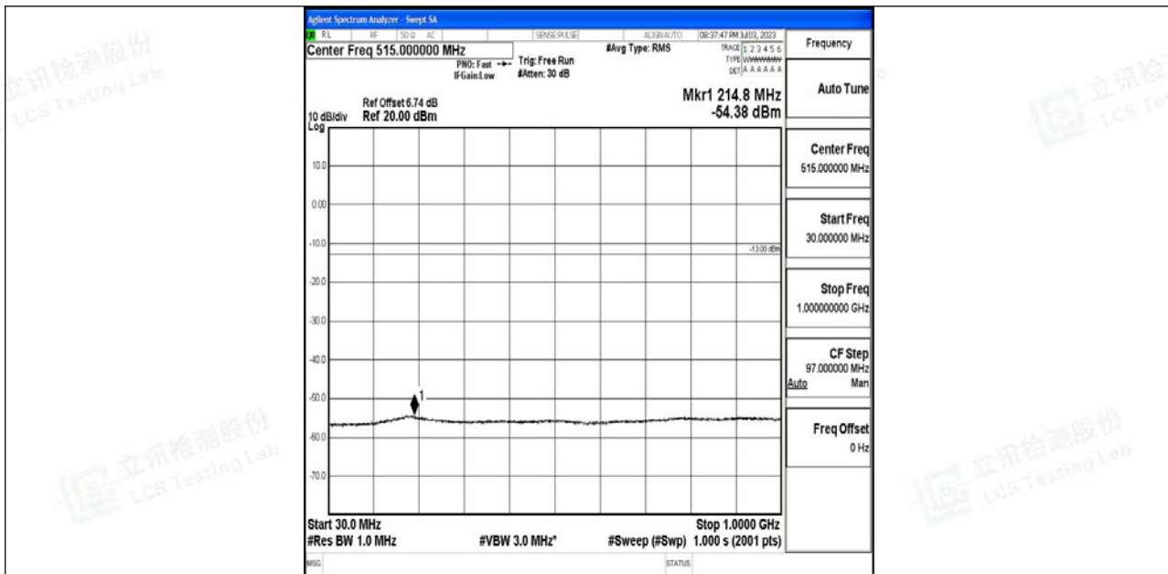
Band4_15MHz_16QAM_20175_1RB#0_30~1000_30~1000
