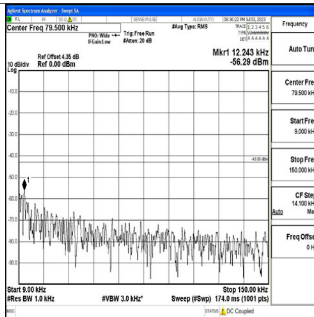
Band4_15MHz_16QAM_20025_1RB#0_0.009~0.15_0.009~0.15
