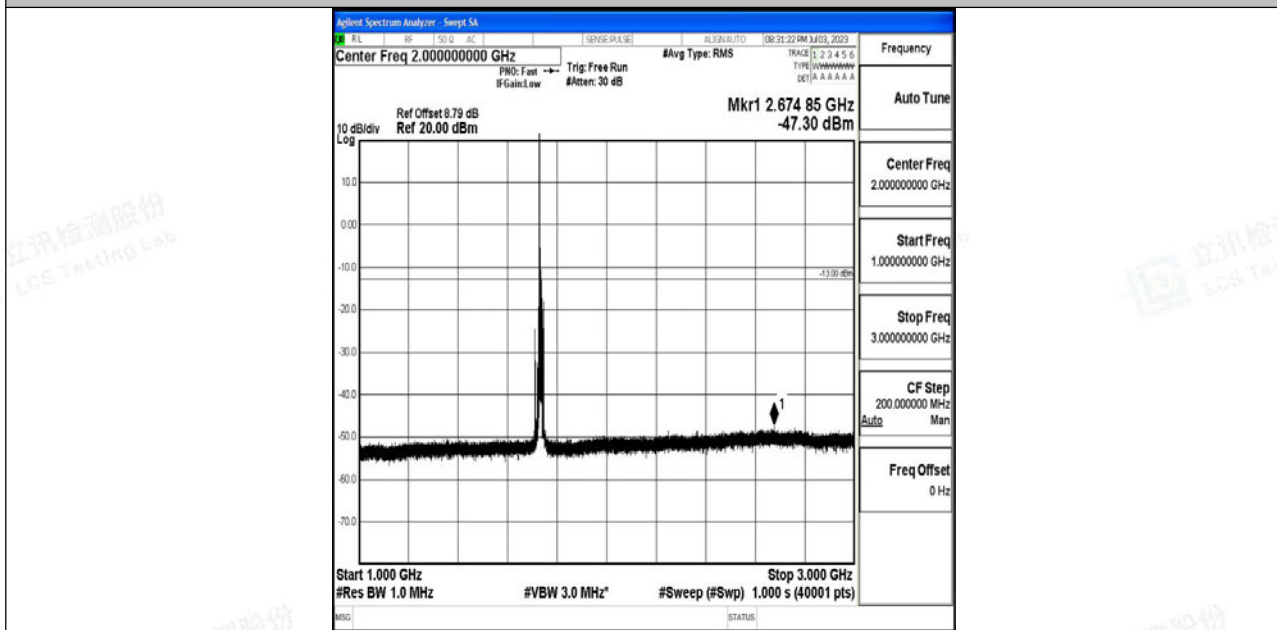
Band4_10MHz_16QAM_20175_1RB#0_1000~3000_1000~3000
