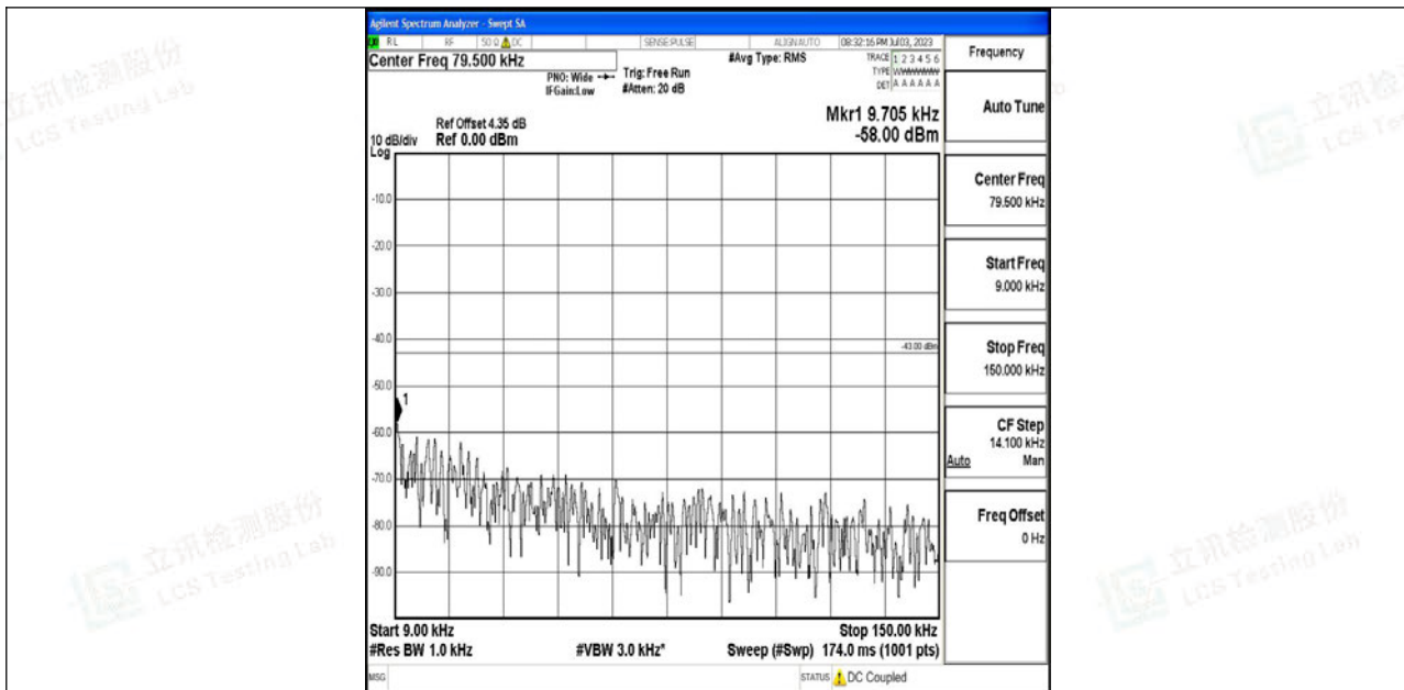
Band4_10MHz_16QAM_20350_1RB#0_0.009~0.15_0.009~0.15
