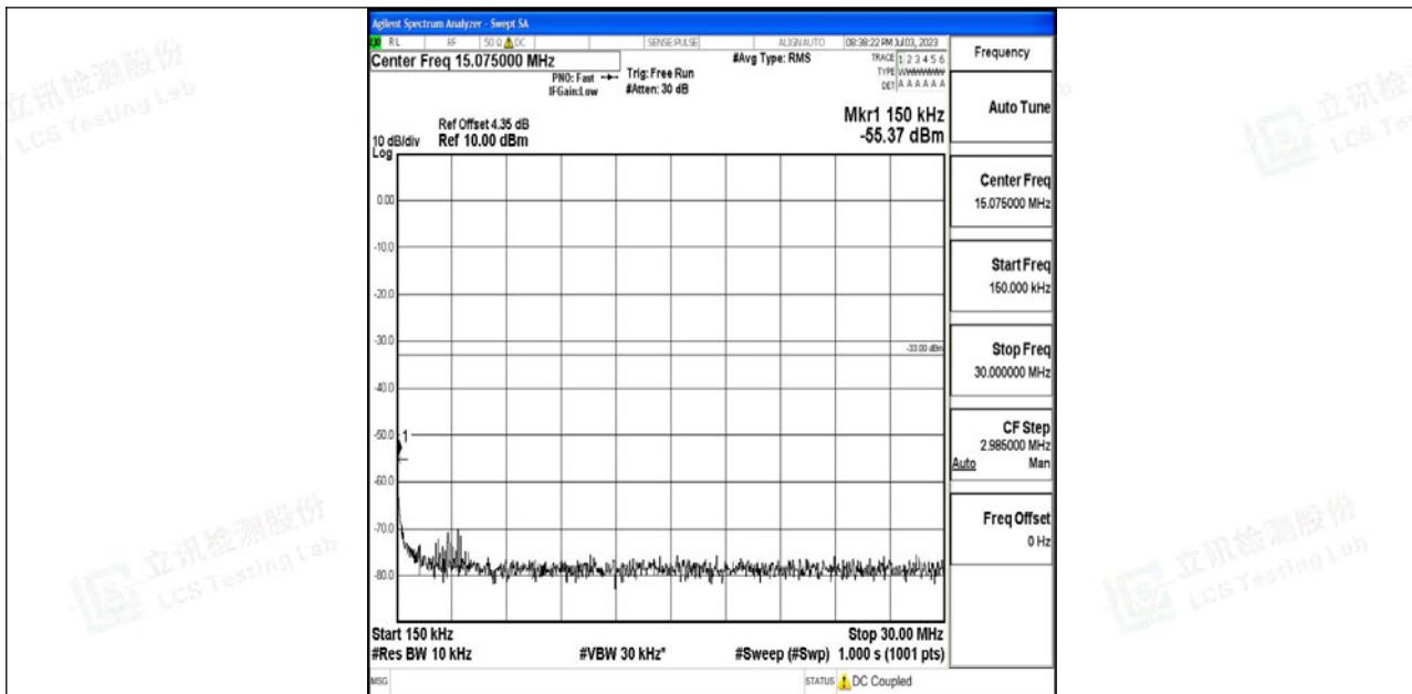
Band4_15MHz_QPSK_20325_1RB#0_0.15~30_0.15~30
