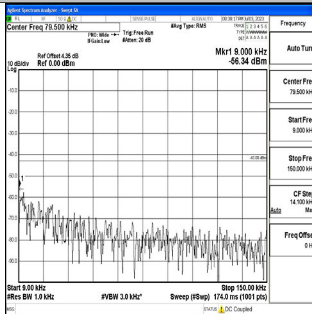
Band4_15MHz_QPSK_20325_1RB#0_0.009~0.15_0.009~0.15
