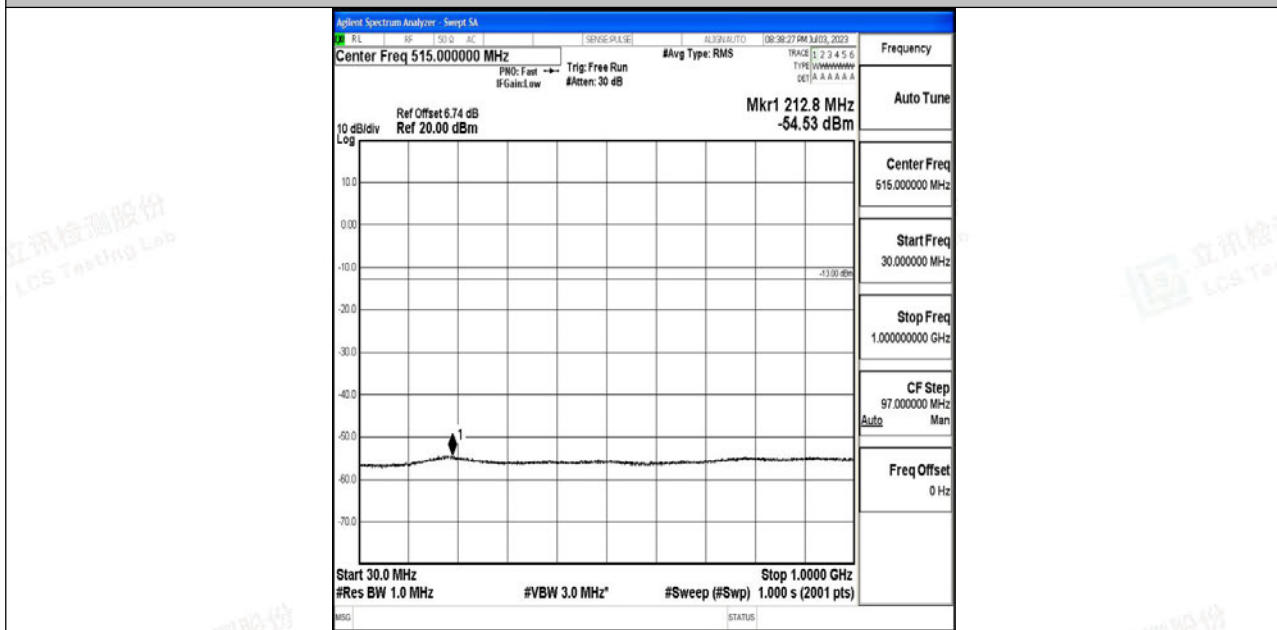
Band4_15MHz_QPSK_20325_1RB#0_30~1000_30~1000
