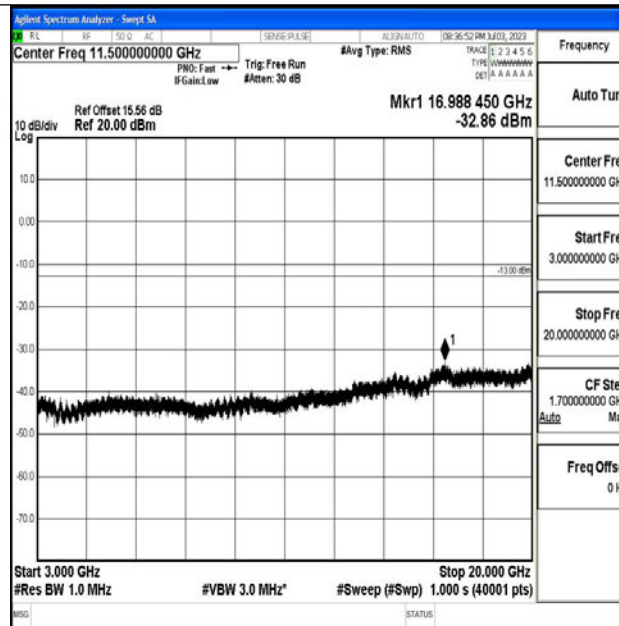
Band4_15MHz_16QAM_20025_1RB#0_3000~20000_3000~20000
