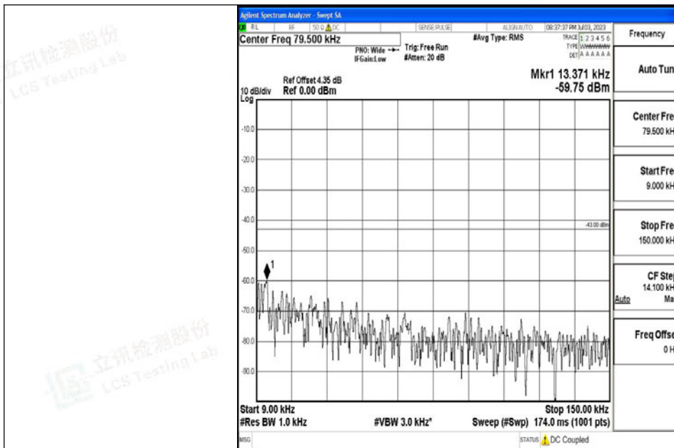
Band4_15MHz_16QAM_20175_1RB#0_0.009~0.15_0.009~0.15
