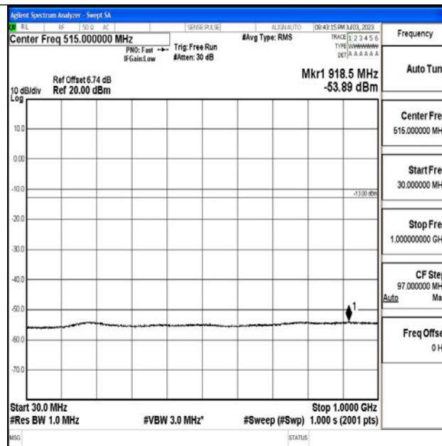
Band4_20MHz_16QAM_20050_1RB#0_30~1000_30~1000
