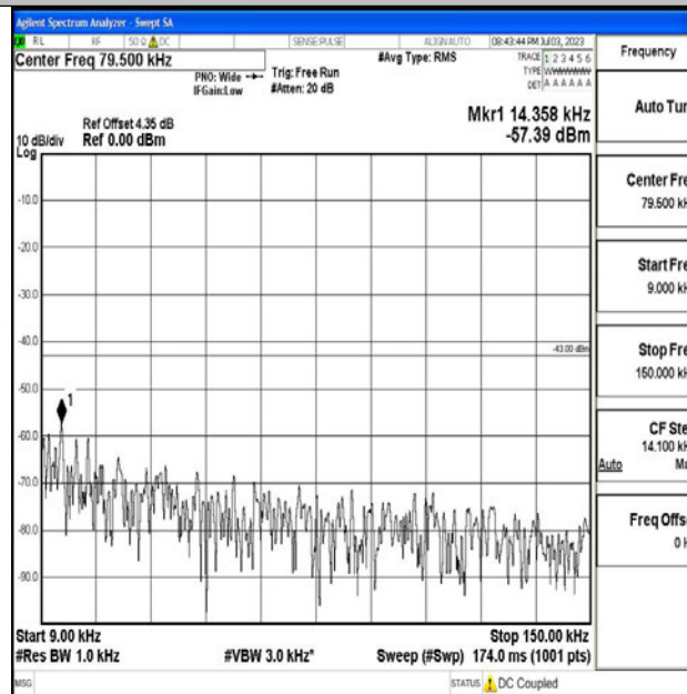
Band4_20MHz_QPSK_20175_1RB#0_0.009~0.15_0.009~0.15
