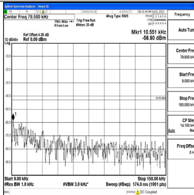
Band4_10MHz_QPSK_20350_1RB#0_0.009~0.15_0.009~0.15
