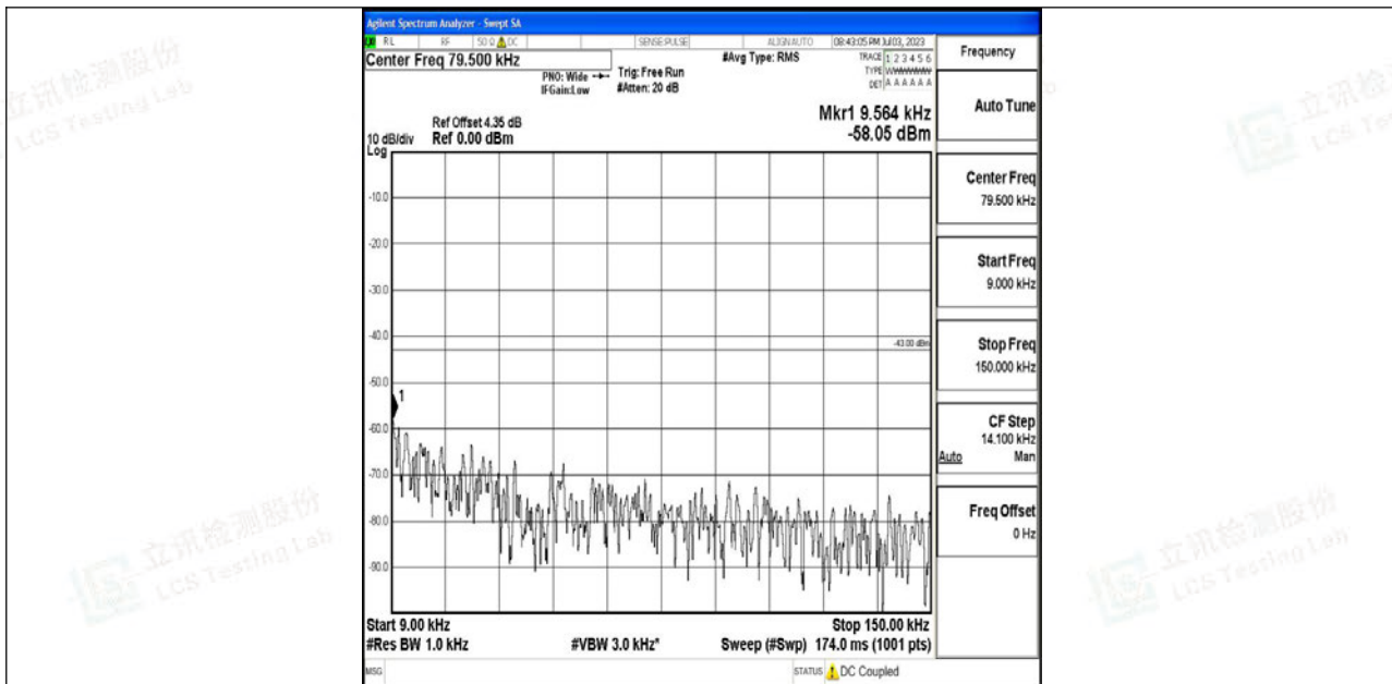
Band4_20MHz_16QAM_20050_1RB#0_0.009~0.15_0.009~0.15
