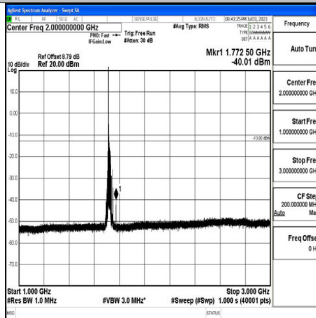
Band4_20MHz_16QAM_20050_1RB#0_1000~3000_1000~3000
