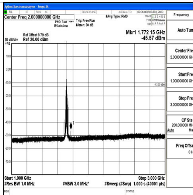
Band4_15MHz_QPSK_20025_1RB#0_1000~3000_1000~3000
