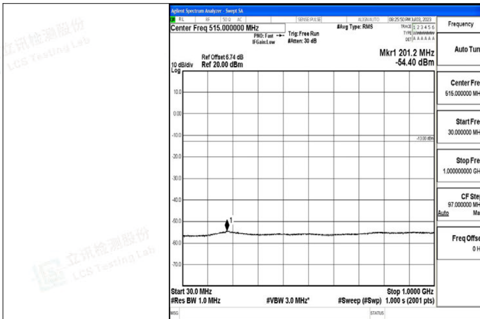
Band4_5MHz_16QAM_20375_1RB#0_30~1000_30~1000
