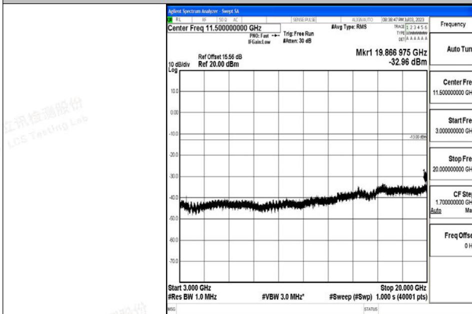
Band4_15MHz_QPSK_20325_1RB#0_3000~20000_3000~20000
