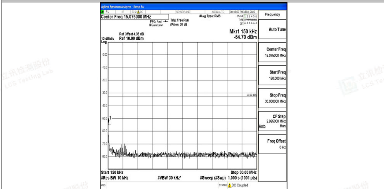
Band4_20MHz_16QAM_20050_1RB#0_0.15~30_0.15~30
