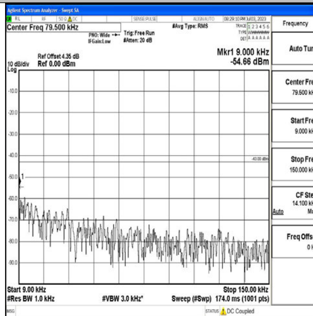
Band4_10MHz_QPSK_20000_1RB#0_0.009~0.15_0.009~0.15
