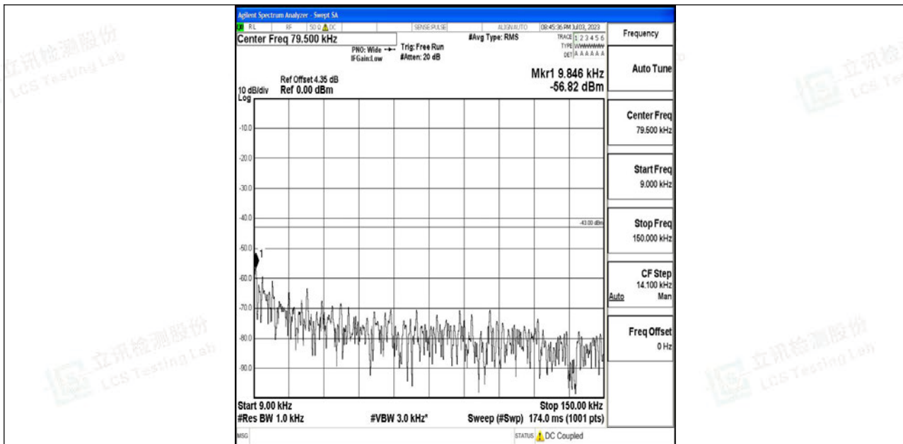
Band4_20MHz_16QAM_20300_1RB#0_0.009~0.15_0.009~0.15
