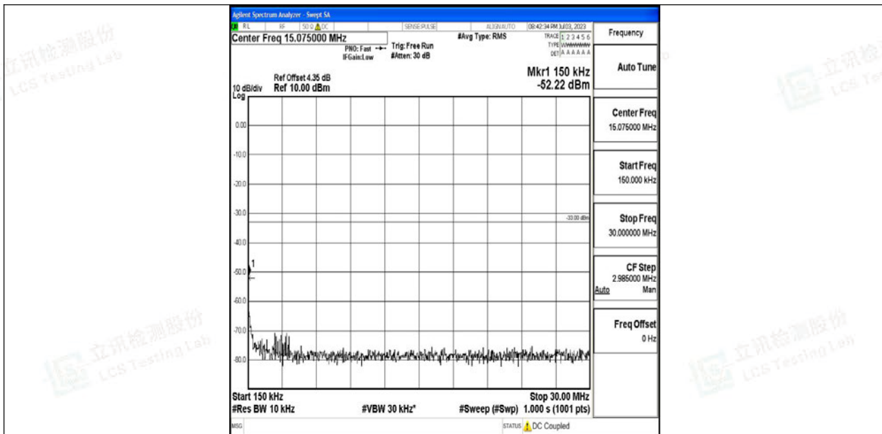
Band4_20MHz_QPSK_20050_1RB#0_0.15~30_0.15~30
