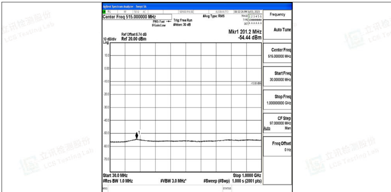
Band4_10MHz_16QAM_20350_1RB#0_30~1000_30~1000
