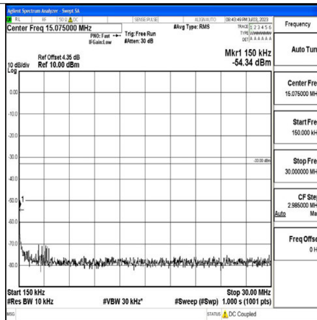
Band4_20MHz_QPSK_20175_1RB#0_0.15~30_0.15~30
