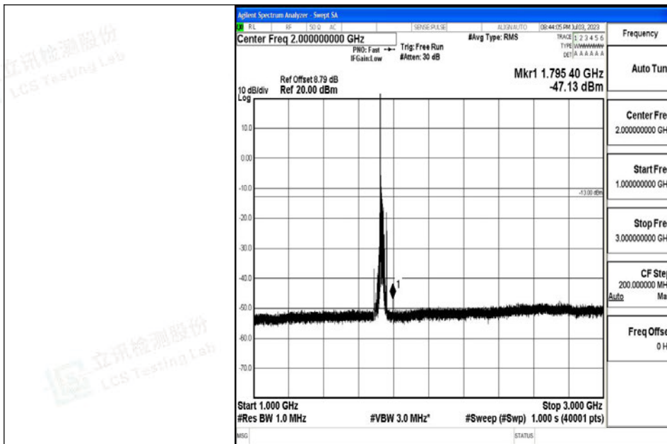
Band4_20MHz_QPSK_20175_1RB#0_1000~3000_1000~3000
