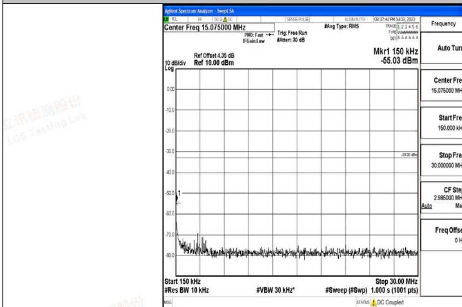
Band4_15MHz_16QAM_20175_1RB#0_0.15~30_0.15~30
