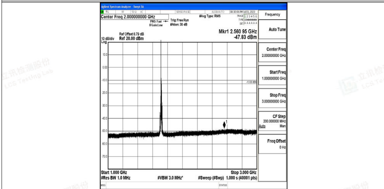
Band4_10MHz_16QAM_20000_1RB#0_1000~3000_1000~3000
