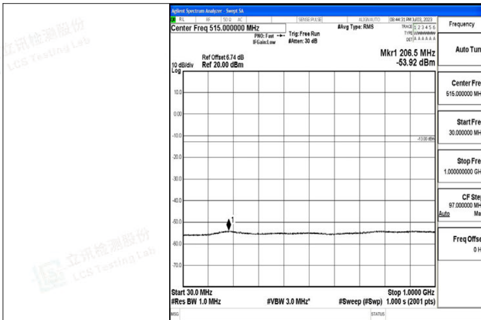
Band4_20MHz_16QAM_20175_1RB#0_30~1000_30~1000
