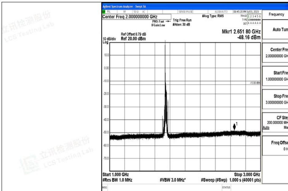
Band4_20MHz_QPSK_20300_1RB#0_1000~3000_1000~3000
