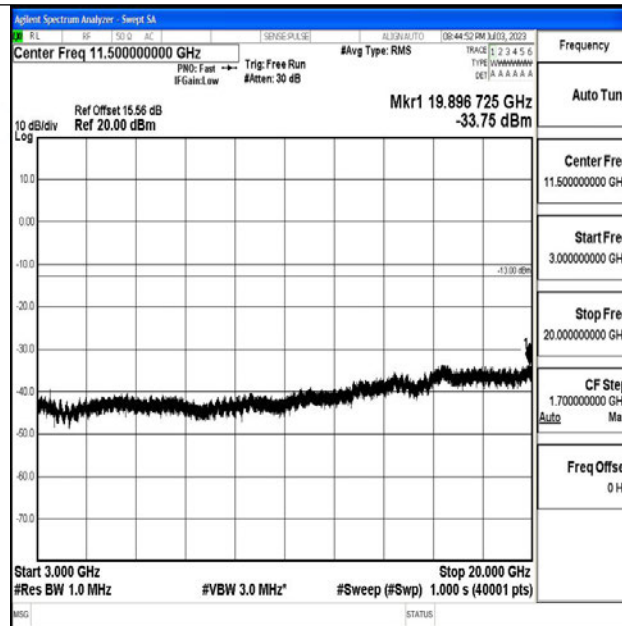
Band4_20MHz_16QAM_20175_1RB#0_3000~20000_3000~20000
