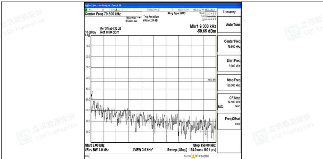
Band4_10MHz_16QAM_20175_1RB#0_0.009~0.15_0.009~0.15
