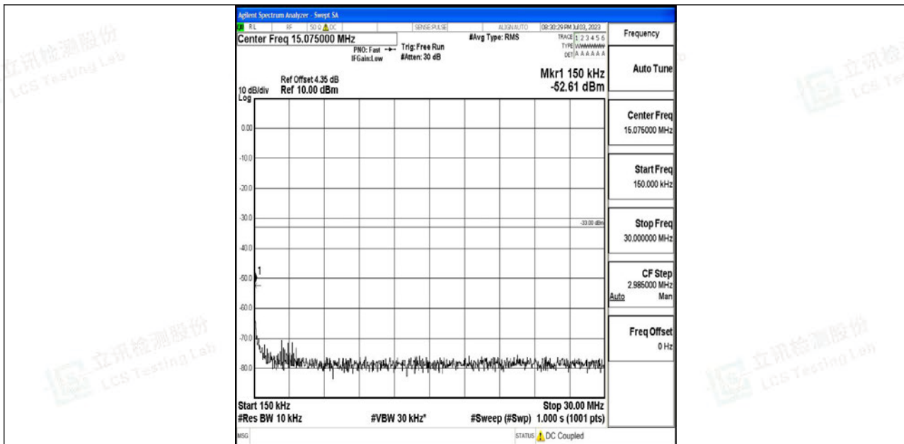
Band4_10MHz_QPSK_20175_1RB#0_0.15~30_0.15~30
