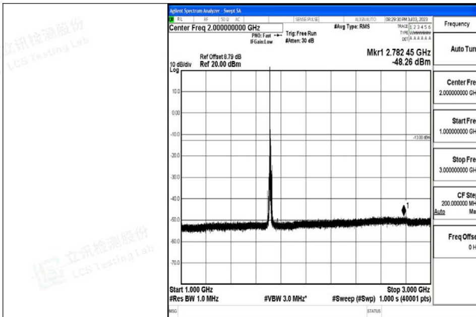
Band4_10MHz_QPSK_20000_1RB#0_1000~3000_1000~3000
