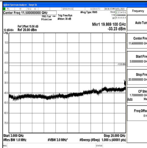
Band4_15MHz_QPSK_20025_1RB#0_3000~20000_3000~20000
