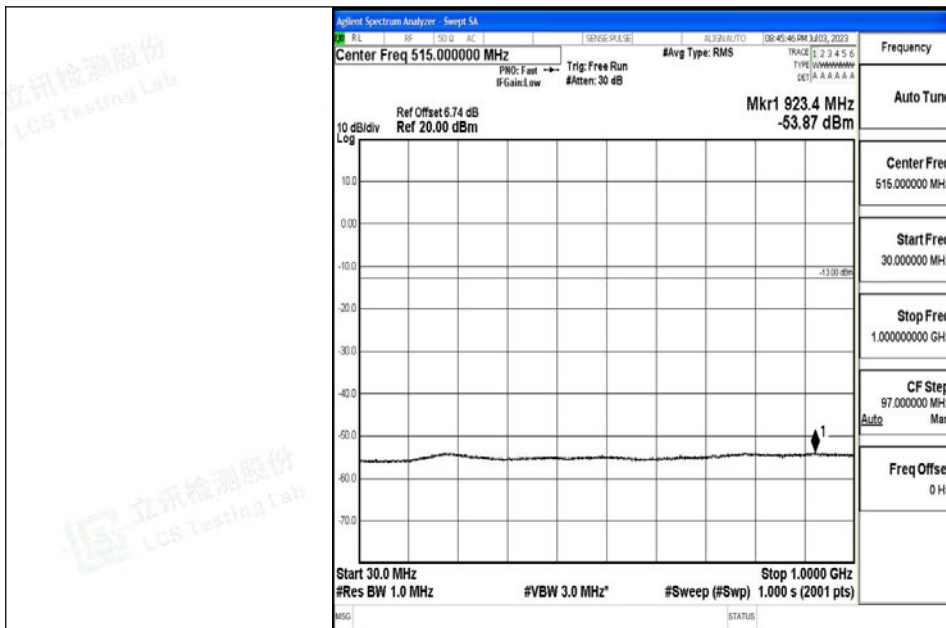
Band4_20MHz_16QAM_20300_1RB#0_30~1000_30~1000
