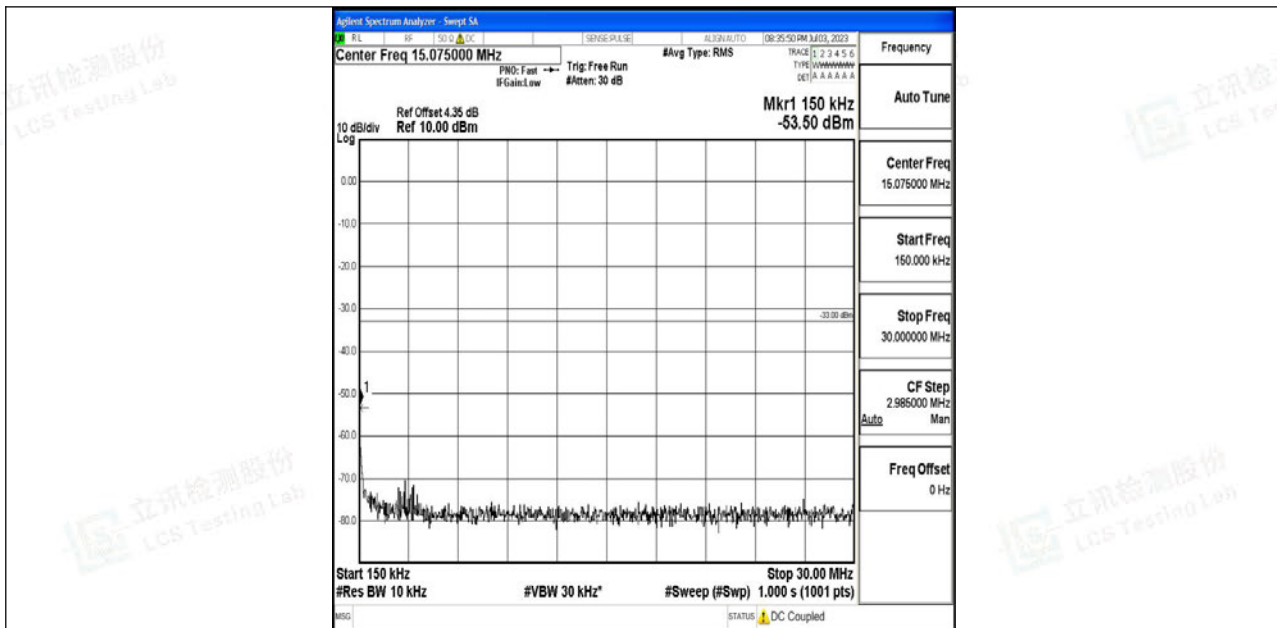
Band4_15MHz_QPSK_20025_1RB#0_0.15~30_0.15~30
