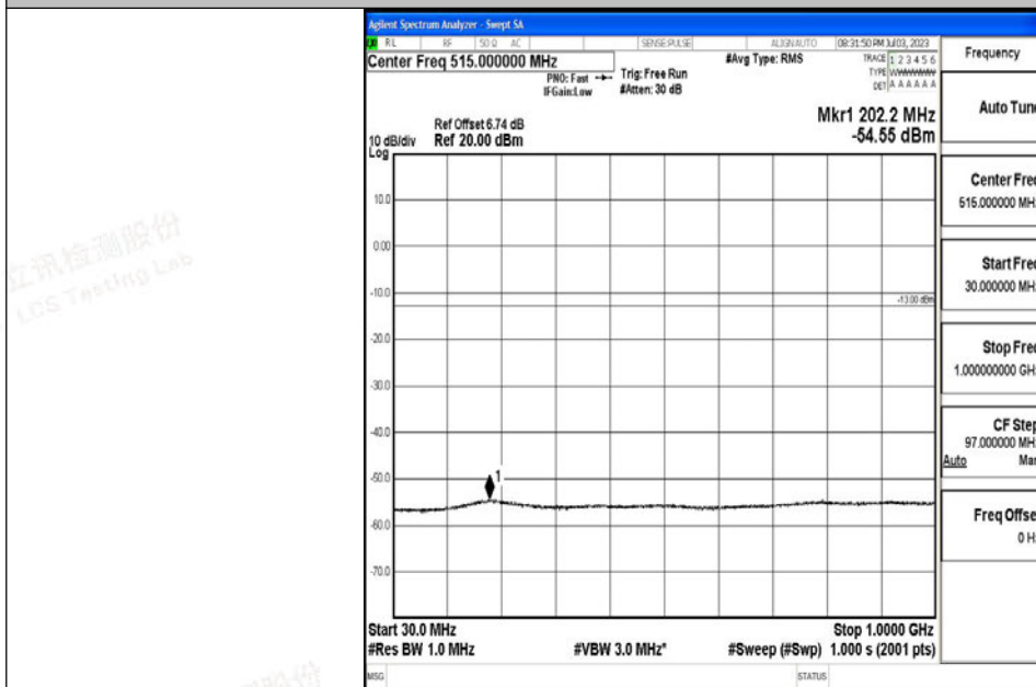
Band4_10MHz_QPSK_20350_1RB#0_30~1000_30~1000
