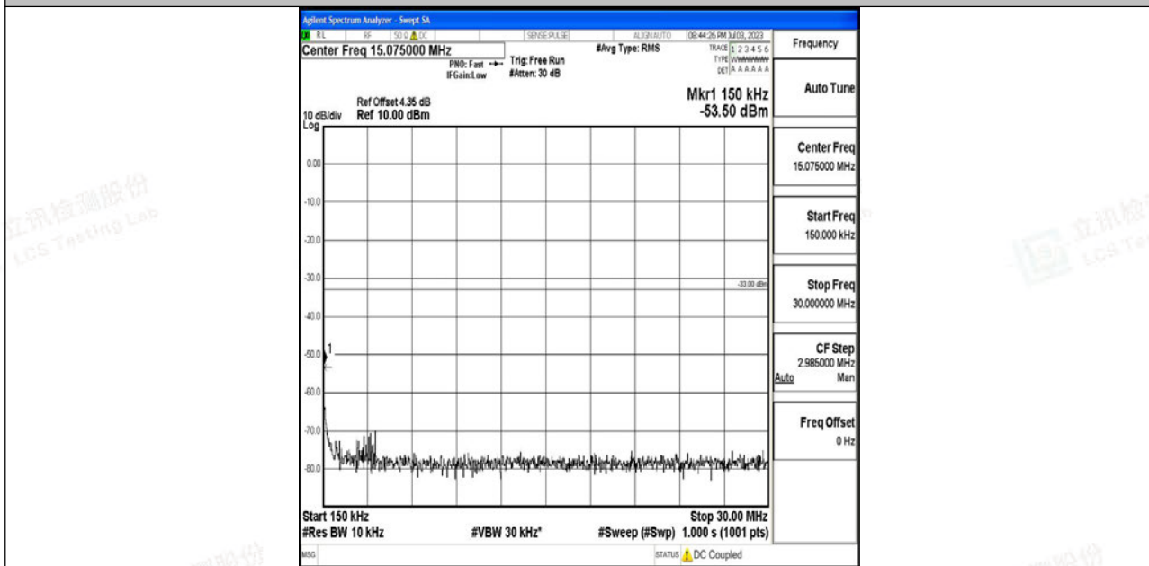
Band4_20MHz_16QAM_20175_1RB#0_0.15~30_0.15~30
