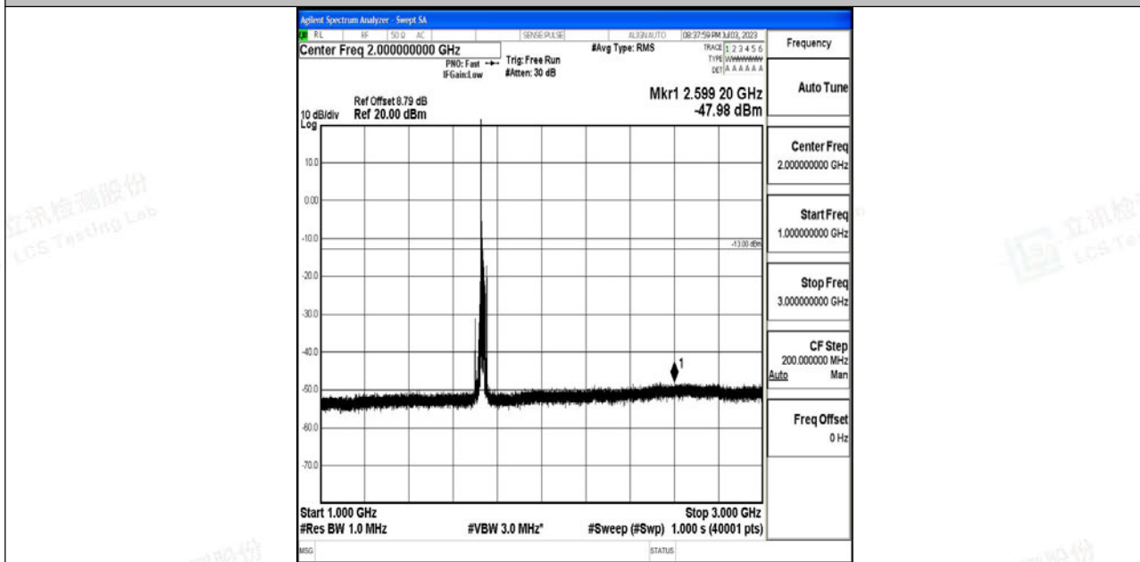
Band4_15MHz_16QAM_20175_1RB#0_1000~3000_1000~3000
