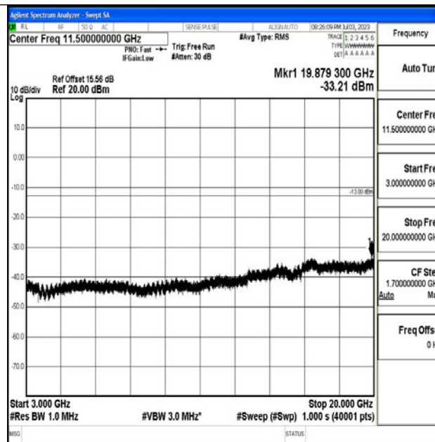
Band4_5MHz_16QAM_20375_1RB#0_3000~20000_3000~20000
