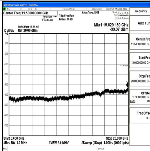
Band4_15MHz_QPSK_20175_1RB#0_3000~20000_3000~20000
