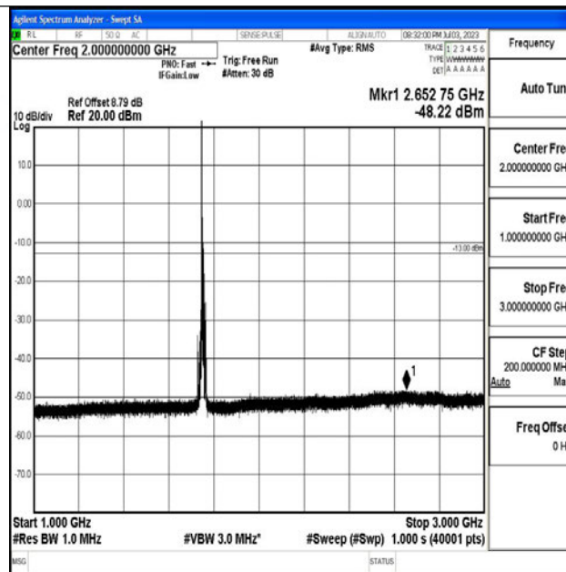
Band4_10MHz_QPSK_20350_1RB#0_1000~3000_1000~3000
