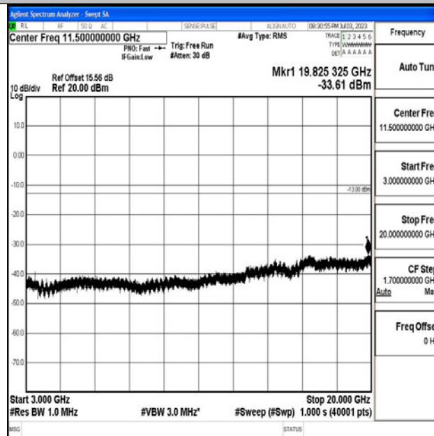
Band4_10MHz_QPSK_20175_1RB#0_3000~20000_3000~20000
