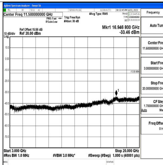
Band4_10MHz_16QAM_20350_1RB#0_3000~20000_3000~20000
