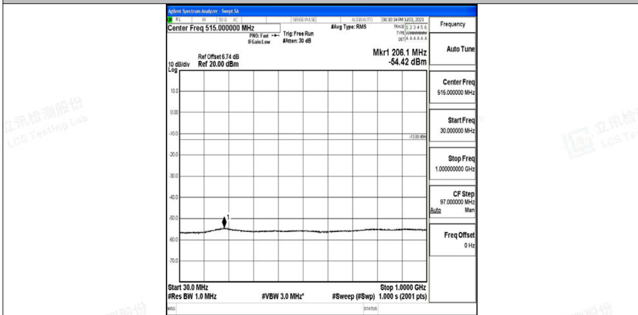
Band4_10MHz_QPSK_20175_1RB#0_30~1000_30~1000
