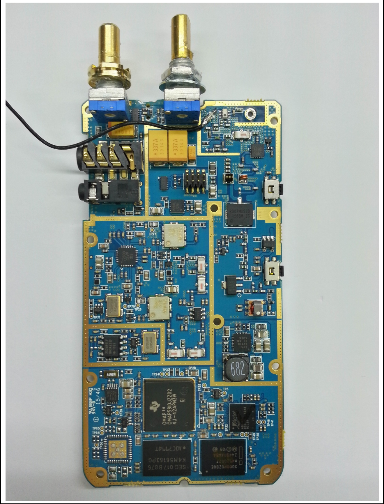
MainBoard-Rear
