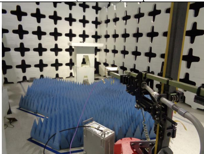
DRWG Horn (18-26GHz) Setup Overview
