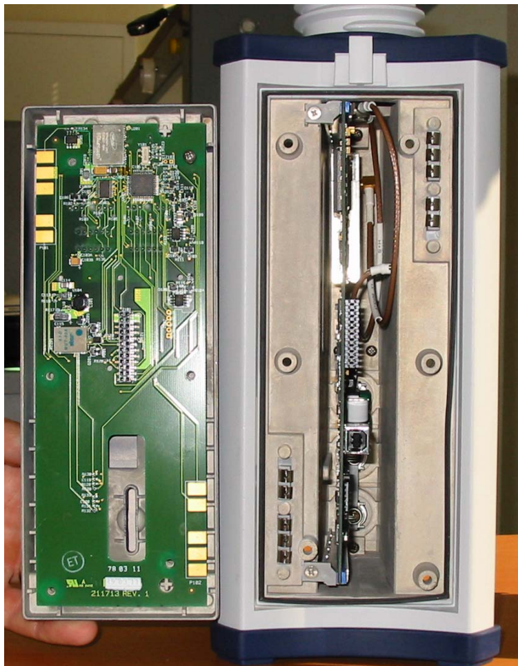
Close up view showing the BlueTooth transceiver's antenna behind a plastic bezel in the front panel (above) and the location of the front panel board in the system (below)
