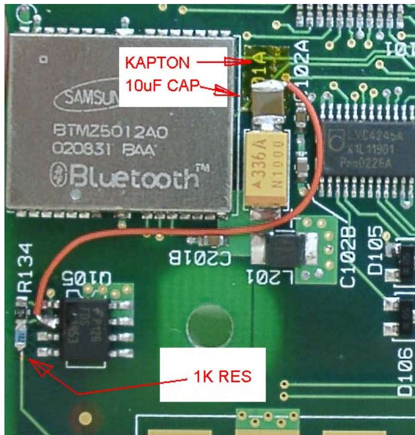
Close-up of BlueTooth chip
