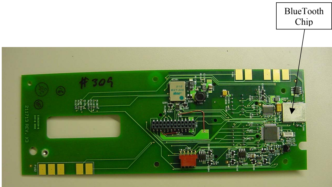
Circuit Board (Front Panel Circuit Board with BlueTooth Transceiver) – Component Side
