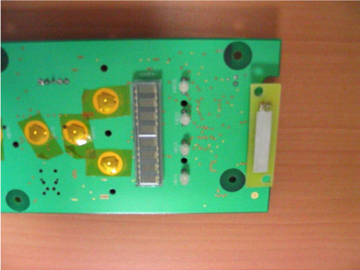
Circuit Board (Front Panel Circuit Board with BlueTooth Transceiver) Rear Side – detail showing antenna connected
