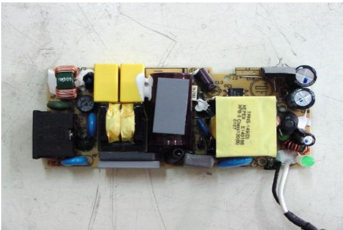
30. Component View of Adaptor's PCB
