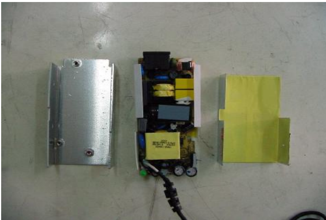
29. Internal View of Adaptor
