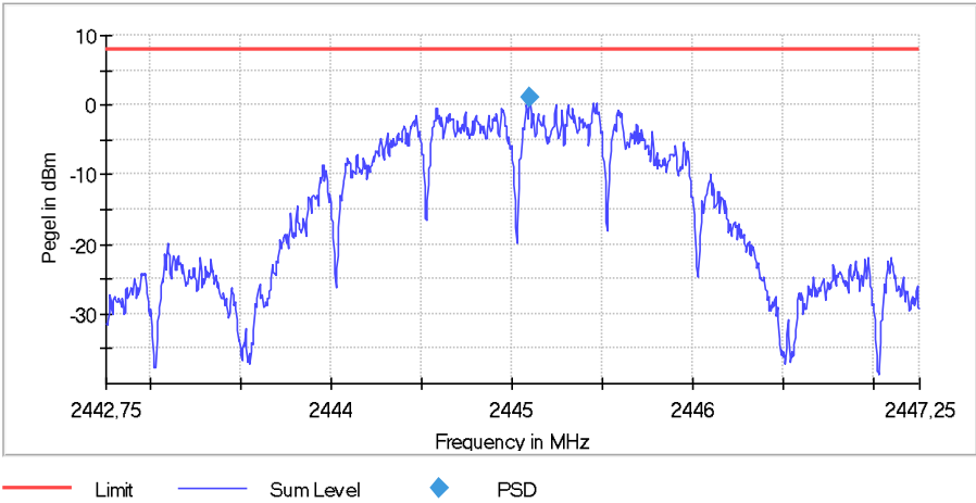
PSD, 2445 MHz, ZigBee
