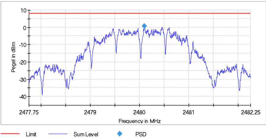
PSD, 2480 MHz, ZigBee
