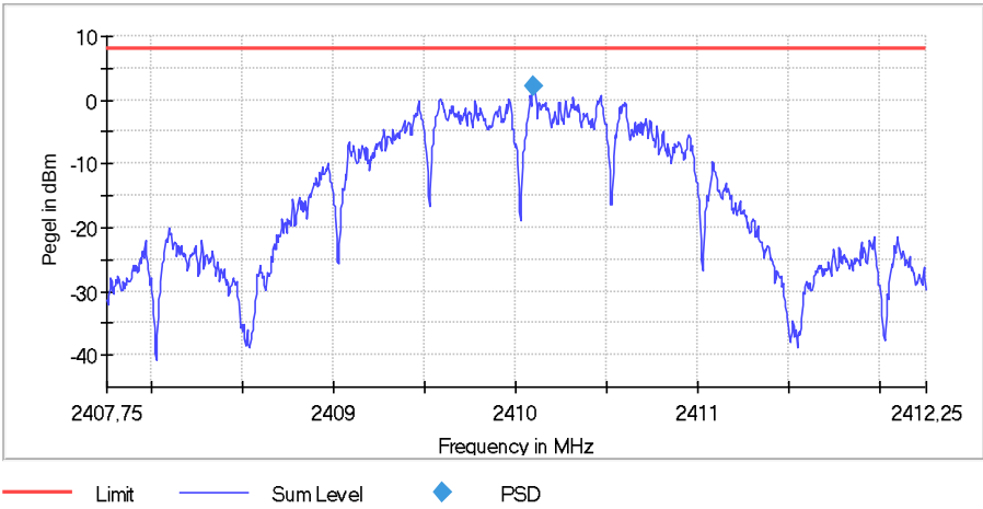
PSD, 2410 MHz, ZigBee
