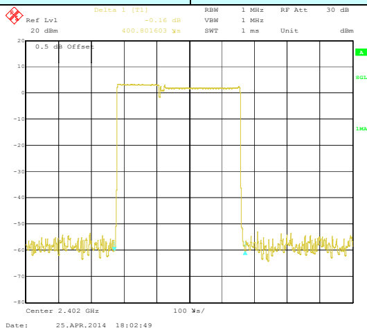
2-DH1
