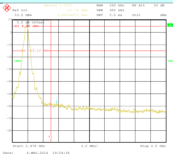
No-hopping mode
