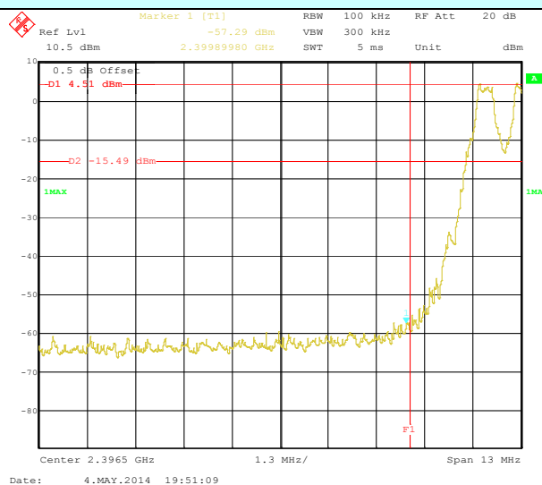
Hopping mode
