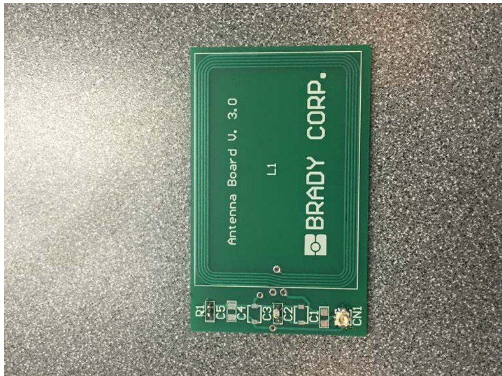
Antenna – ANT2000 PCB – Side 1
