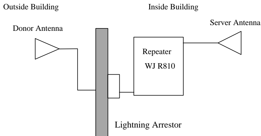
Figure 1-3. WJ R810 Typical Usage
