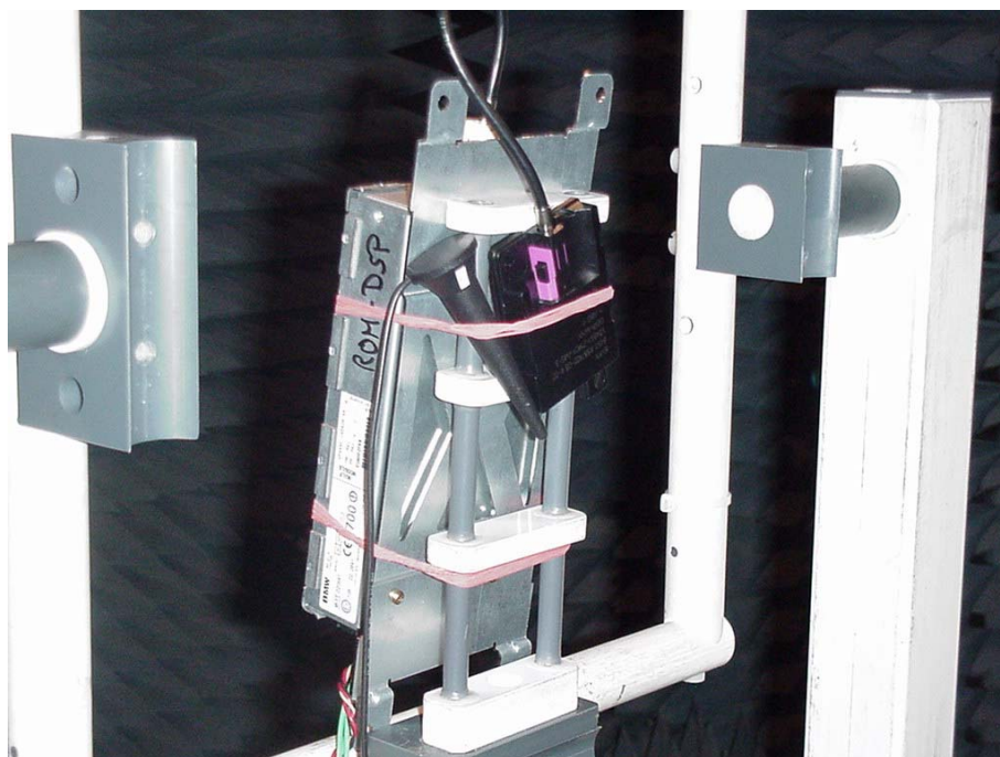
Picture 2 : EUT with external antenna and signalling antenna to the test system
