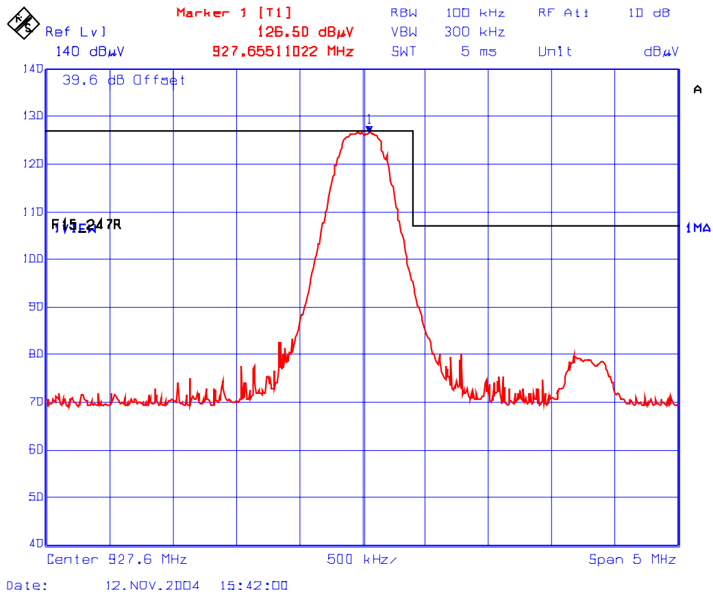
Plot 38: Band-Edge RF Radiated Emissions @ 3 meters Upper End of Frequency Band Test Configuration 1: EUT with 1/4 Wave Antenna (1.5 dBi Gain) Rx Antenna Orientation: Vertical
