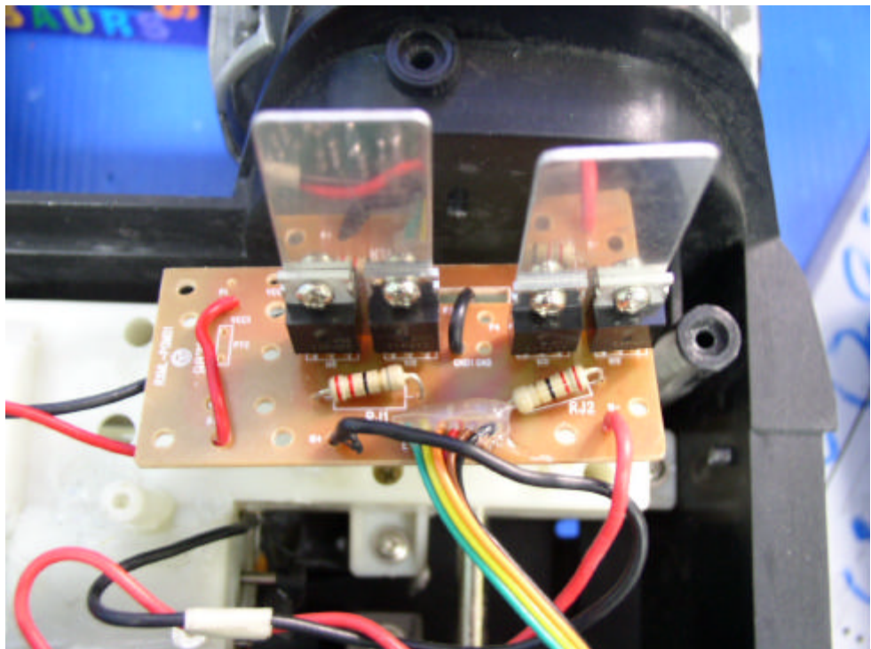
Iphoto8 (Control PCB for front wheel)
