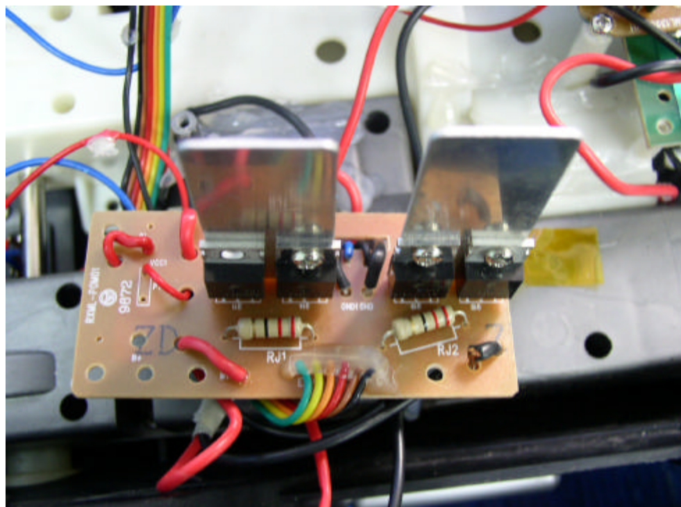
Iphoto2 (Control PCB for rear wheel)
