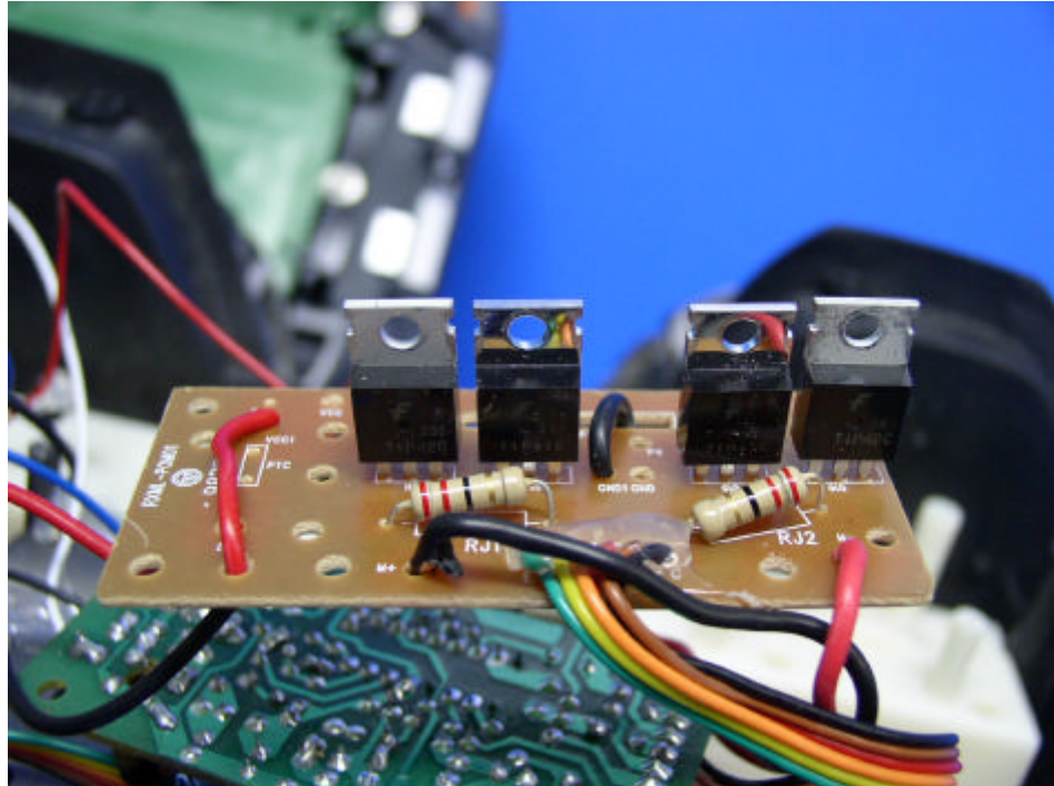
Iphoto9 (Control PCB for front wheel)
