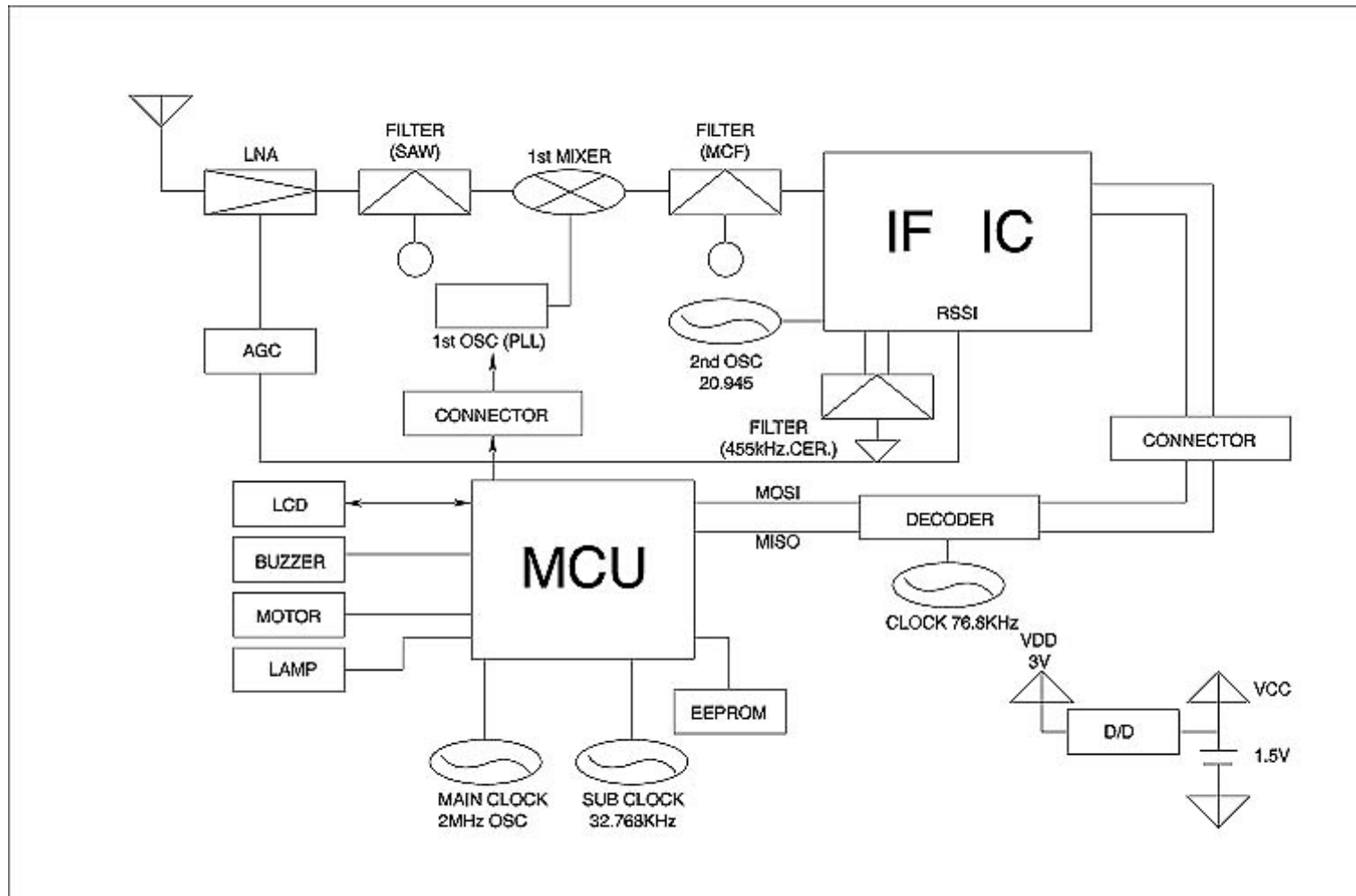
*DFP-920 LOGIC/RF PART BLOCK DIAGRAM.
