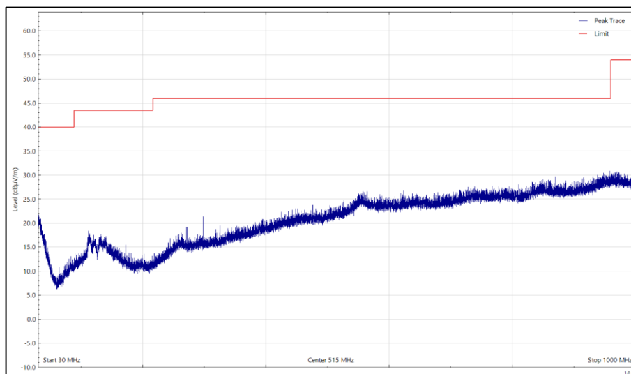
Figure 18 - NFC Transmit - Y Plane, 13.56MHz, 30 MHz to 1 GHz, Horizontal (Peak)
