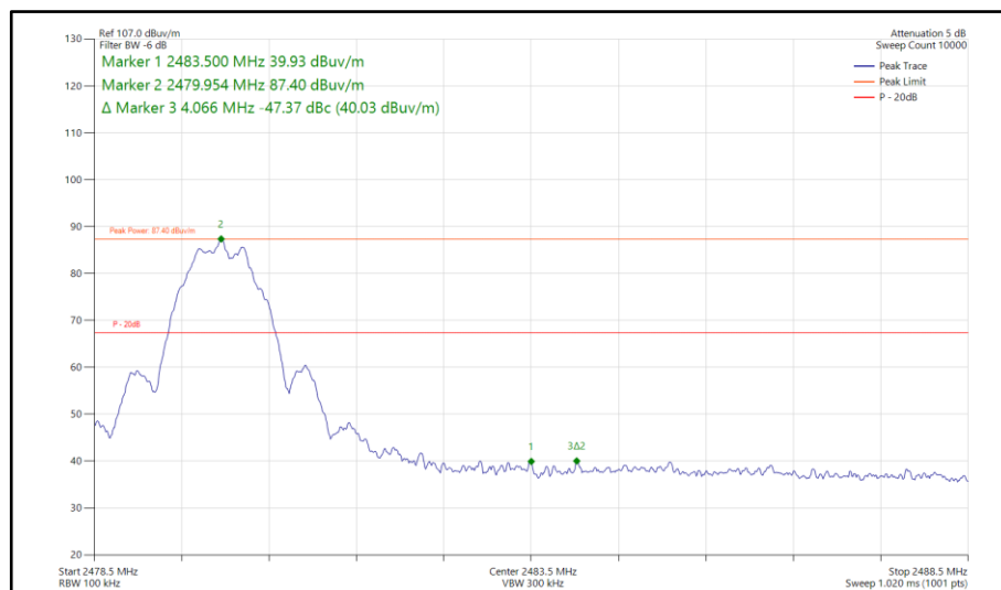
Figure 22 - CH39_UBC_LE1M_Core0_iPA, 2480 MHz, Band Edge Frequency 2483.5 MHz
