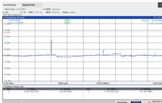
Conducted Emissions 2550-10000 MHz, 2402 MHz, 2Mb
