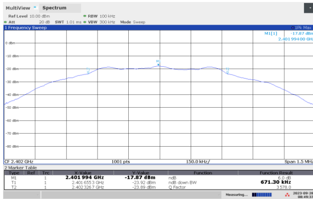
DTS BW, 2402 MHz, 1M
