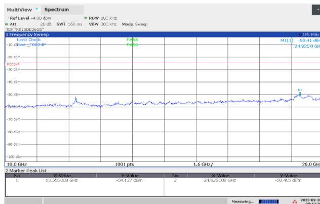
Conducted Emissions 10-26 GHz, 2480 MHz, 2Mb
