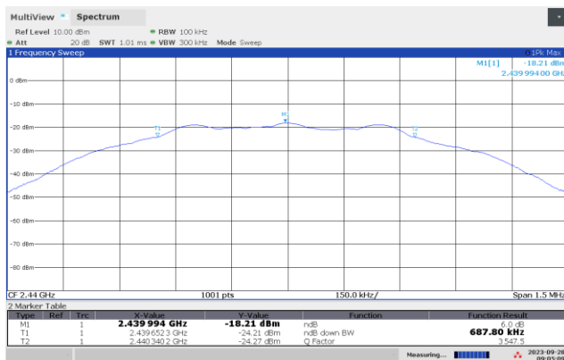
DTS BW, 2440 MHz, 1M
