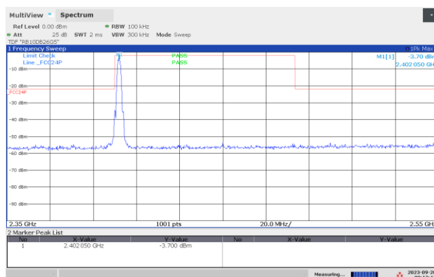
Conducted Emissions 2350-2550 MHz, 2402 MHz, 2Mb
