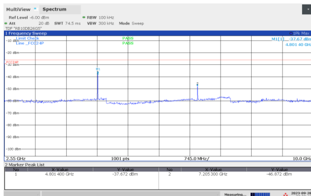
Conducted Emissions 2550-10000 MHz, 2402 MHz, 1Mb
