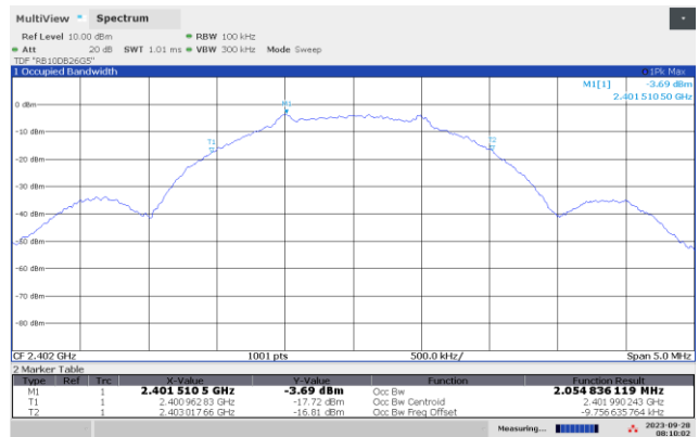
2402 MHz, 99% Occupied BW, 2Mb
