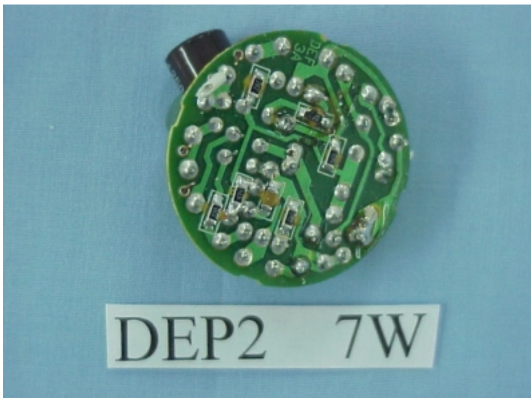
FIGURE 10 ELECTRONIC ENERGY SAVING LAMP (M/N: DEP2/7W) MAIN BOARD (SOLDERED SIDE)
