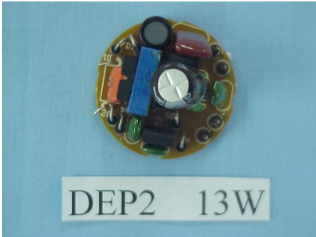
FIGURE 13 ELECTRONIC ENERGY SAVING LAMP (M/N: DEP2/13W) MAIN BOARD (COMPONENT SIDE)
