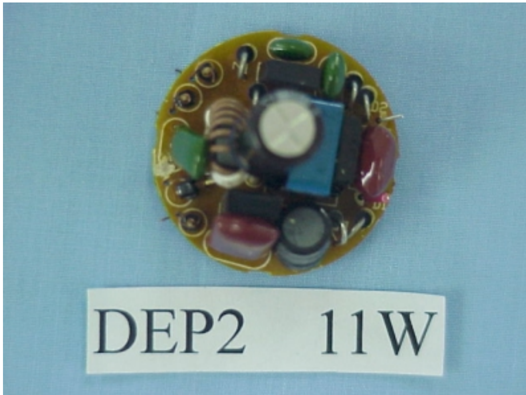
FIGURE 4 ELECTRONIC ENERGY SAVING LAMP (M/N: DEP2/11W) MAIN BOARD (COMPONENT SIDE)
