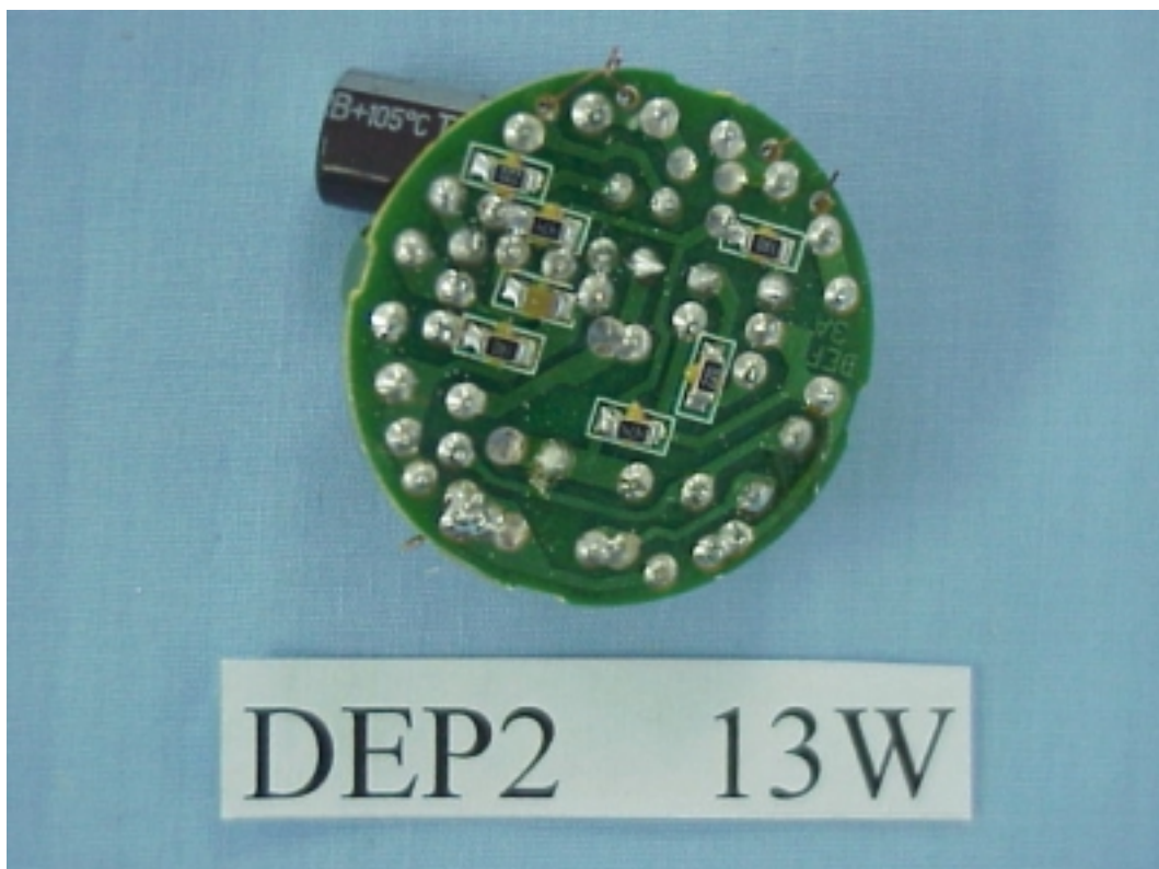
FIGURE 14 ELECTRONIC ENERGY SAVING LAMP (M/N: DEP2/13W) MAIN BOARD (SOLDERED SIDE)
