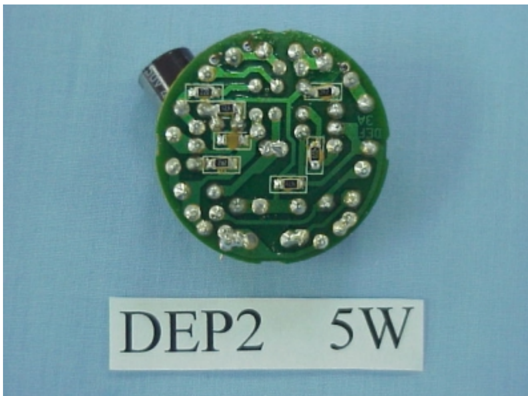
FIGURE 3 ELECTRONIC ENERGY SAVING LAMP (M/N: DEP2/5W) MAIN BOARD (SOLDERED SIDE)
