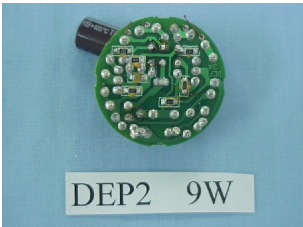
FIGURE 12 ELECTRONIC ENERGY SAVING LAMP (M/N: DEP2/9W) MAIN BOARD (SOLDERED SIDE)
