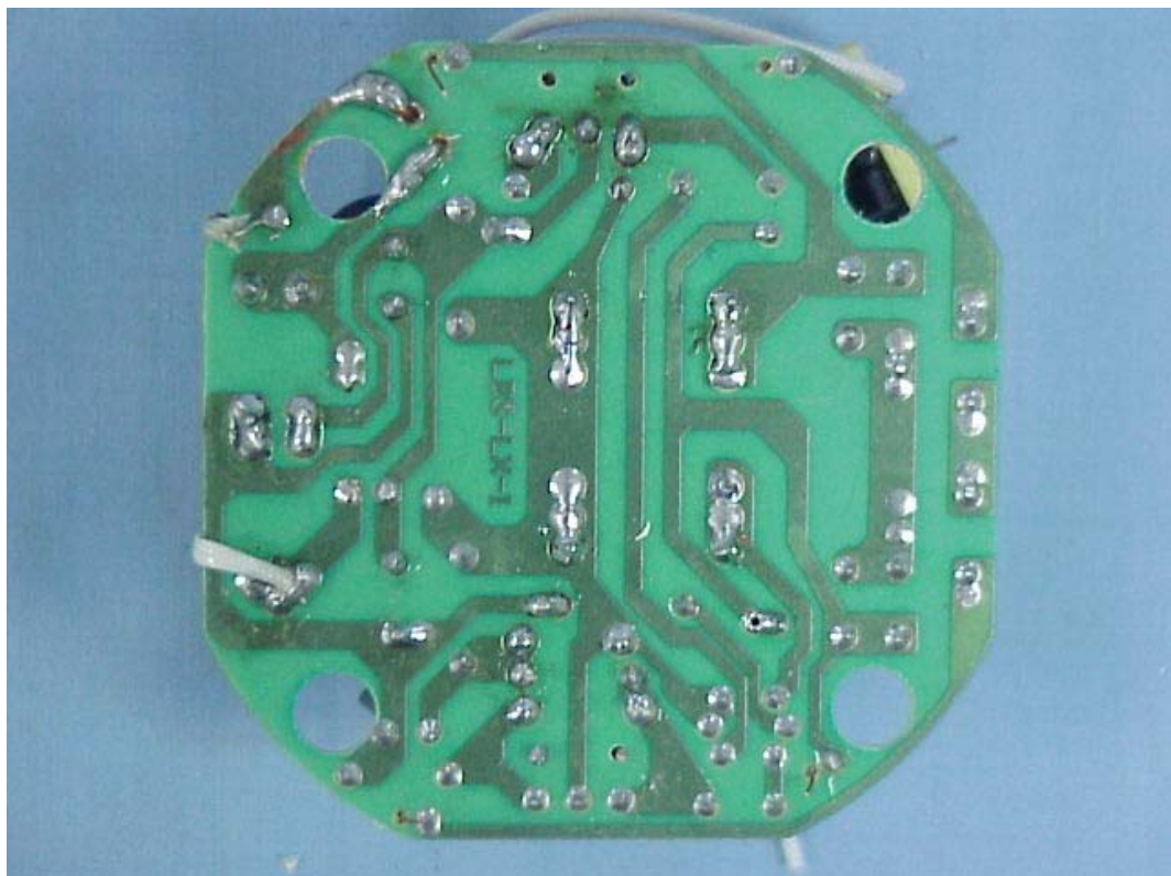
FIGURE 15 ELECTRONICS ENERGY SAVING LAMP (M/N: DEC 3E39 65W) MAIN BOARD (SOLDERED SIDE)
