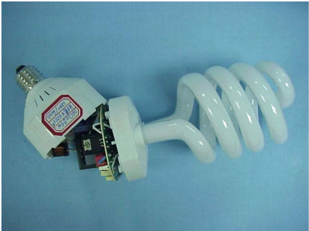
FIGURE 7 ELECTRONIC ENERGY SAVING LAMP (M/N: DEC 3E26 85W) COVER REMOVED
