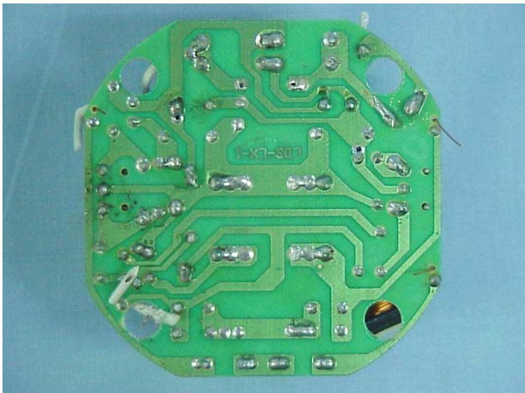
FIGURE 9 ELECTRONICS ENERGY SAVING LAMP (M/N: DEC 3E26 85W) MAIN BOARD (SOLDERED SIDE)
