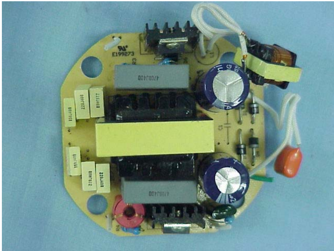
FIGURE 11 ELECTRONIC ENERGY SAVING LAMP (M/N: DEC 3E39 45W) MAIN BOARD (COMPONENT SIDE)
