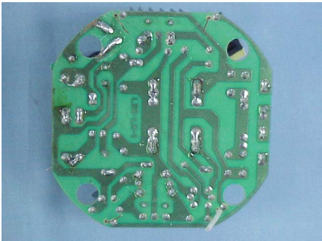
FIGURE 18 ELECTRONICS ENERGY SAVING LAMP (M/N: DEC 3E39 85W) MAIN BOARD (SOLDERED SIDE)
