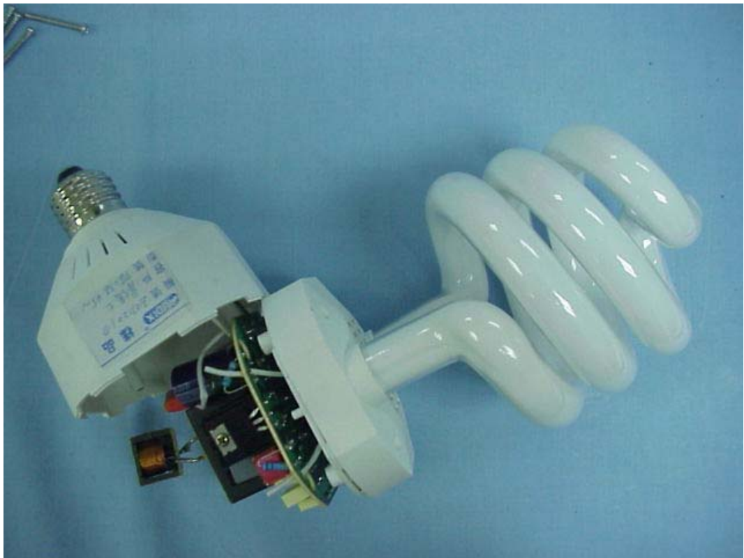
FIGURE 1 ELECTRONIC ENERGY SAVING LAMP (M/N: DEC 3E26 45W) COVER REMOVED
