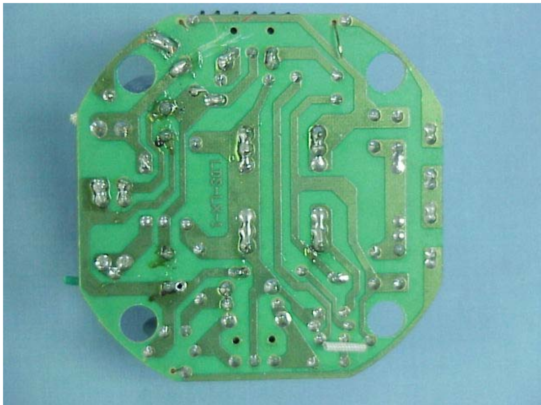
FIGURE 12 ELECTRONICS ENERGY SAVING LAMP (M/N: DEC 3E39 45W) MAIN BOARD (SOLDERED SIDE)
