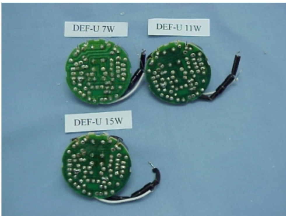
Figure 6 Electronic Energy Saving Lamp (M/N: DEF-U SERIES) MAIN BOARD (COMPONENT SIDE)
