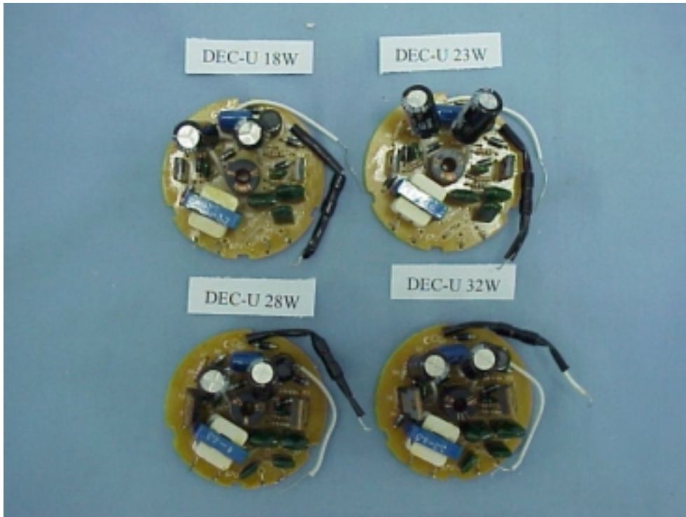
Figure 3 Electronic Energy Saving Lamp (M/N: DEC-U SERIES) MAIN BOARD (COMPONENT SIDE)
