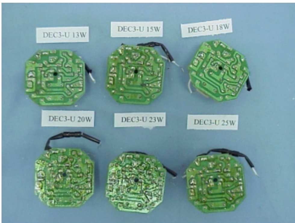
Figure 2 Electronic Energy Saving Lamp (M/N: DEC3-U SERIES) MAIN BOARD (SOLDERED SIDE)
