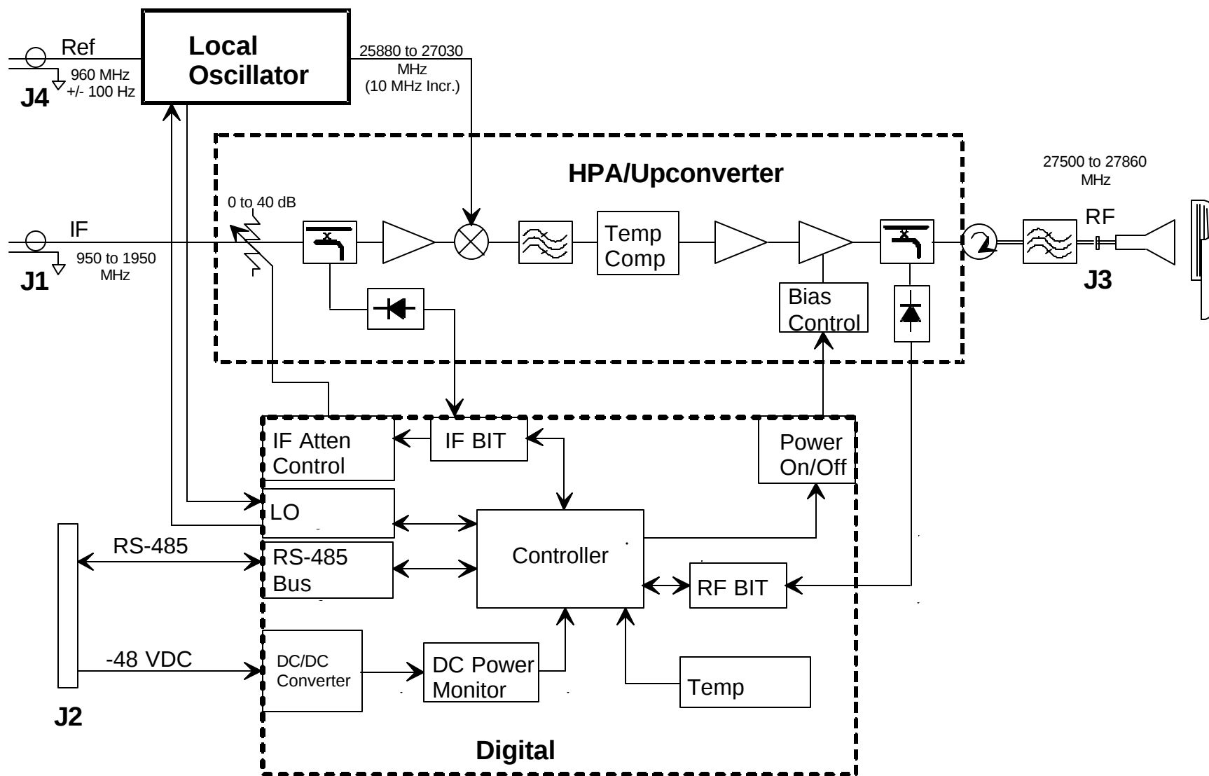
Figure 4-1 Node Transmitter Block Diagram
