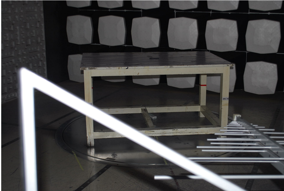
Radiated Emission
