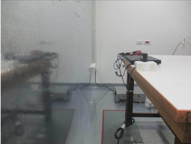
Part_15_247_WLAN_2.4G_Conduction_Setup
