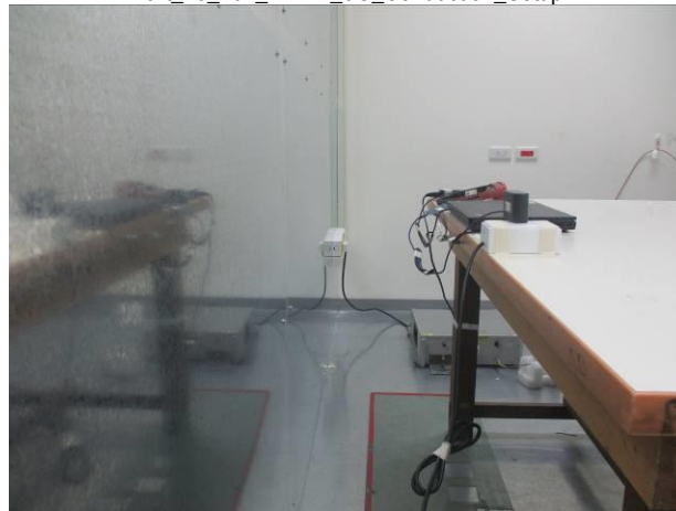
Part_15_407_WLAN_5G_Normal_DFS_Slave_Setup
