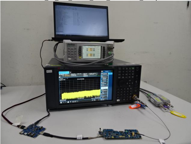
Part_15_247_WLAN_2.4G_Conducted_Setup
