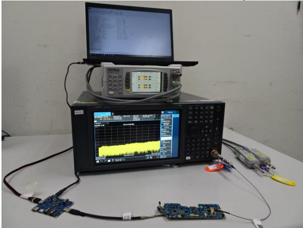
Part_15_407_WLAN_6E_Normal_Setup
