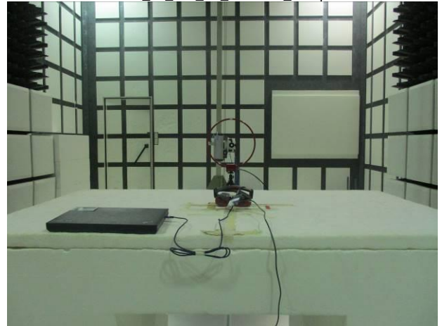
Part_15_247_LE_Radiated_Setup
