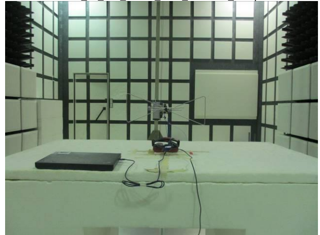
Part_15_247_WLAN_2.4G_Radiated_Setup
