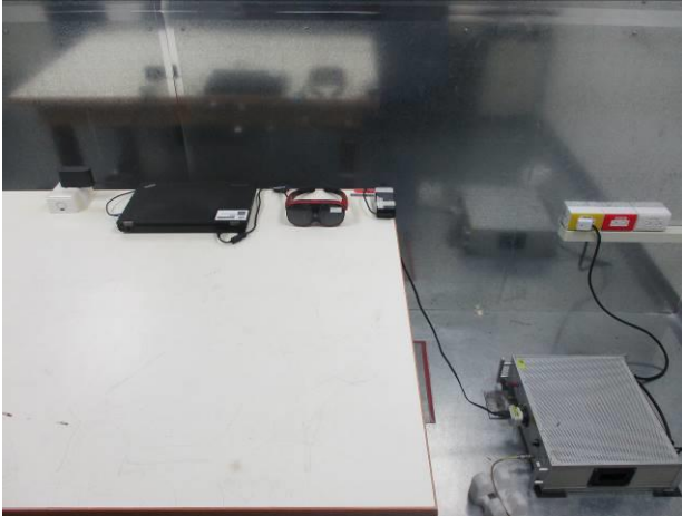
Part_15_247_WLAN_2.4G_Conduction_Setup
