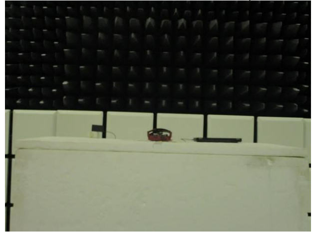
Part_15_247_WLAN_2.4G_Radiated_Setup
