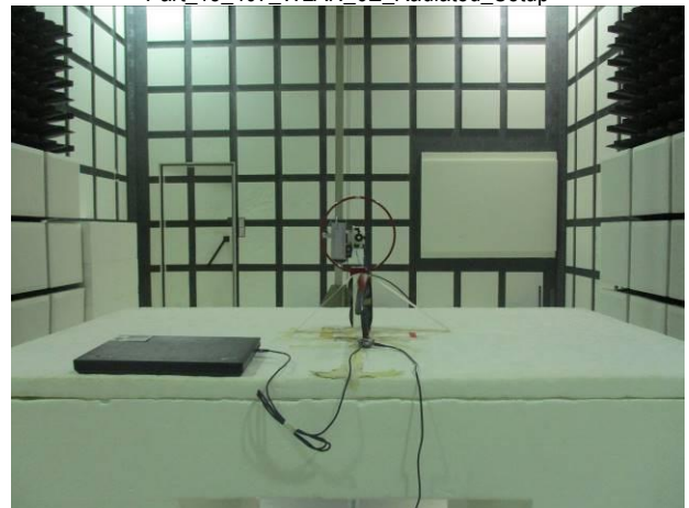
Part_15_407_WLAN_6E_Radiated_Setup
