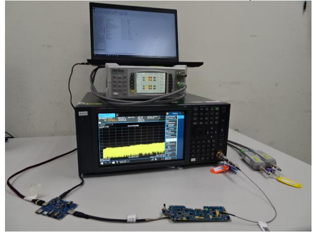
Part_15_249_SRD_2.4G_Radiated_Setup
