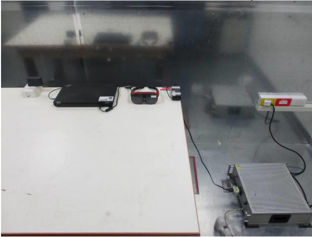
Part_15_407_WLAN_6E_Conduction_Setup
