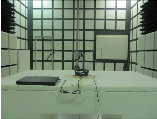
Part_15_249_SRD_2.4G_Radiated_Setup
