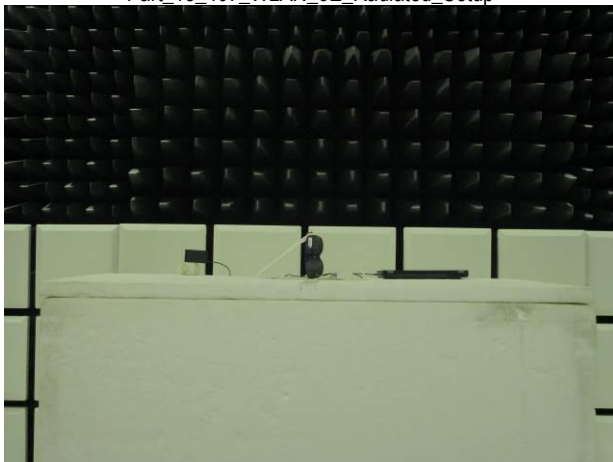
Part_15_407_WLAN_6E_Radiated_Setup
