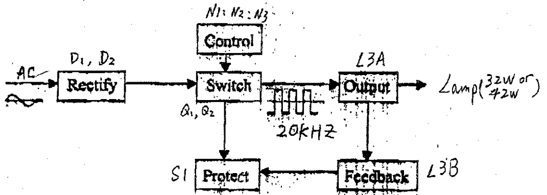
A32W-1, A42W-1 Electronic Ballast Block Diagram
