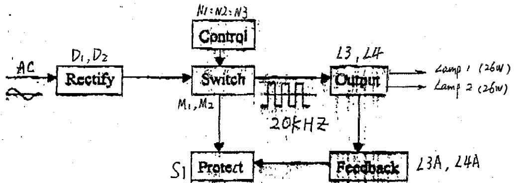
A26W-2 Electronic Ballast Block Diagram
