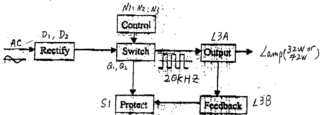
A32W-1, A42W-1 Electronic Ballast Block Diagram
