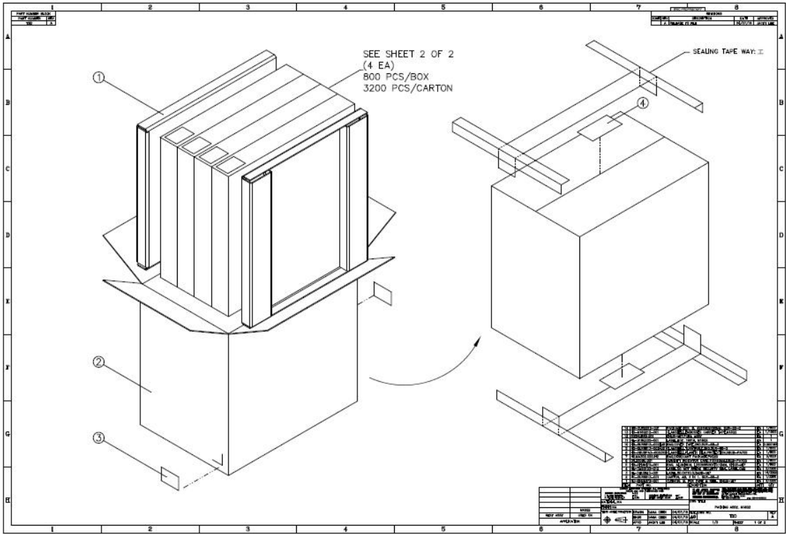
Figure 27. Packing—carton
