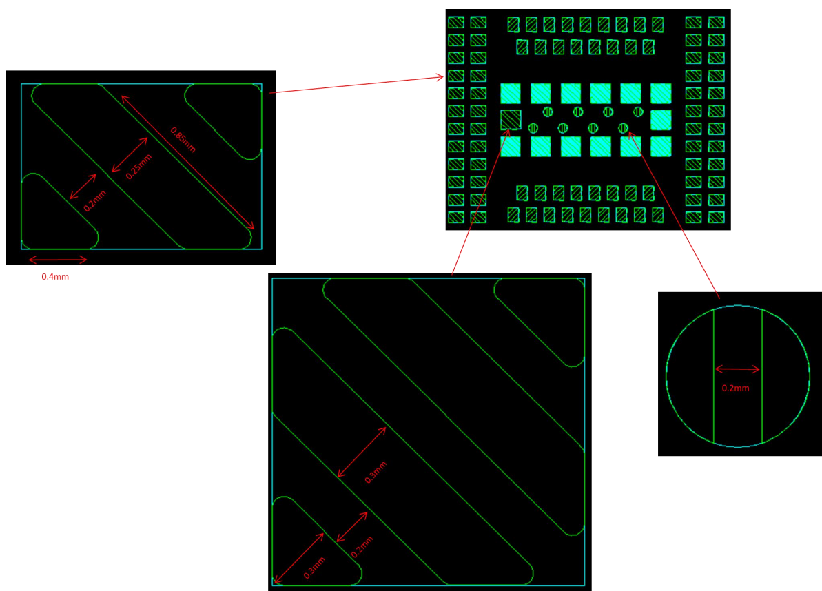
Figure 24. Stencil-foil drawing
