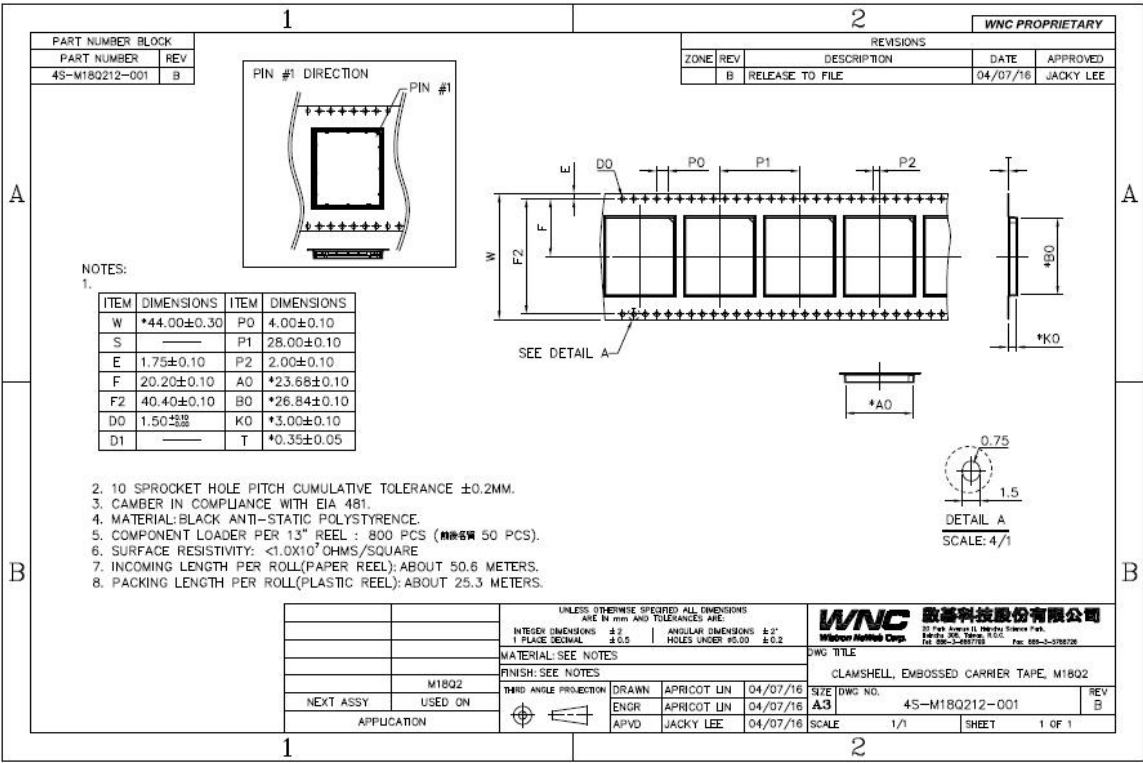
Figure 25. Packing--tape
