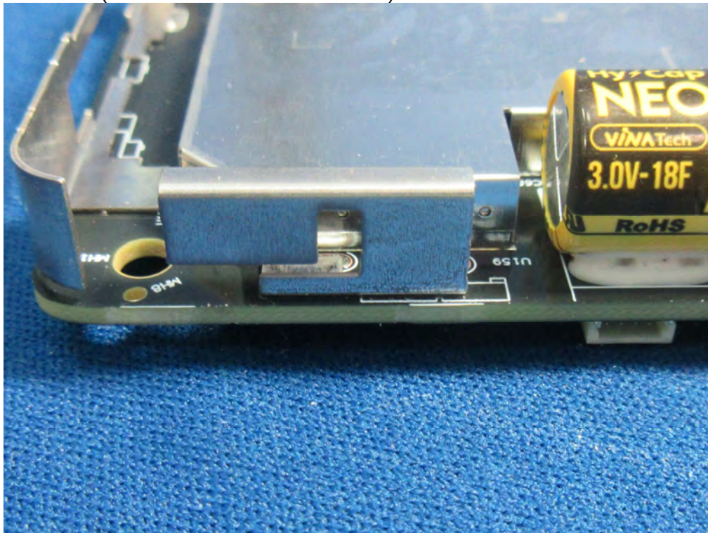
(8) EUT Photo (WWAN Antenna 2, Model No.: LTE_Div)
