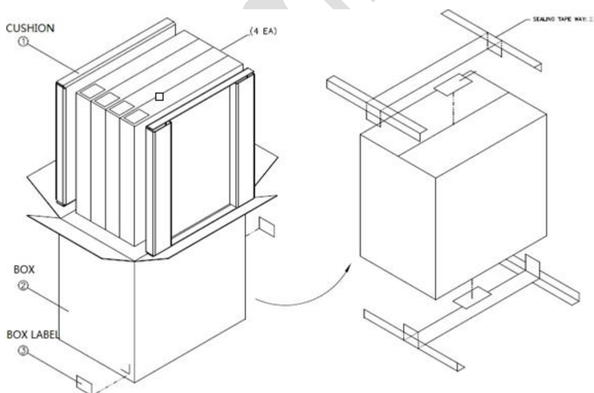
Figure 7-2. Packaging--tape
