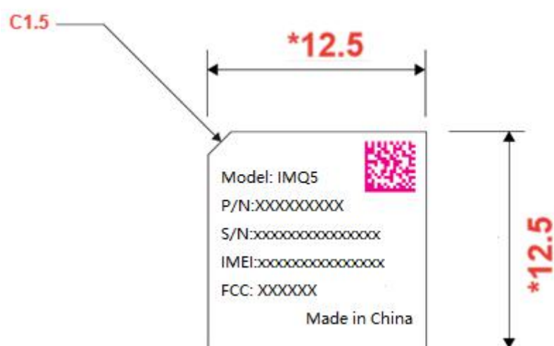
Figure 7-1. Label drawing
