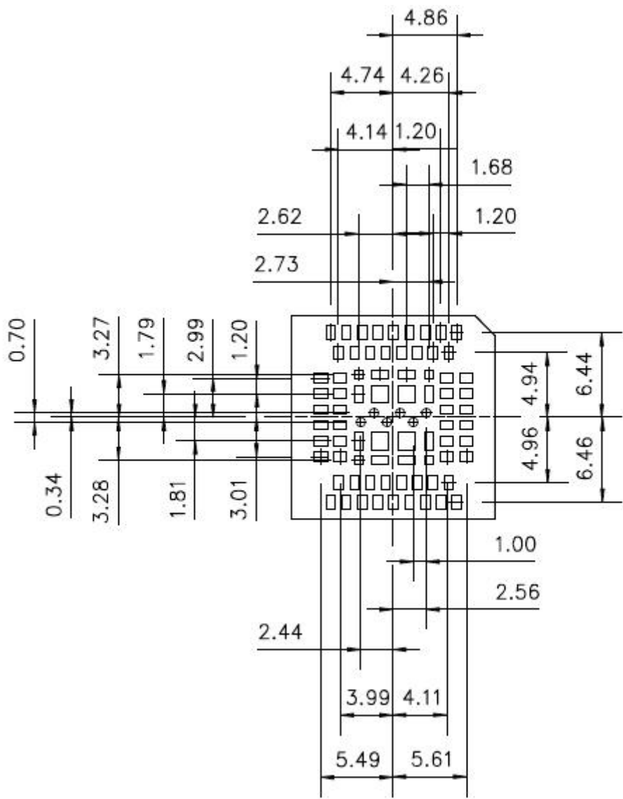
Figure 5-2. Pad dimensions (bottom view)
