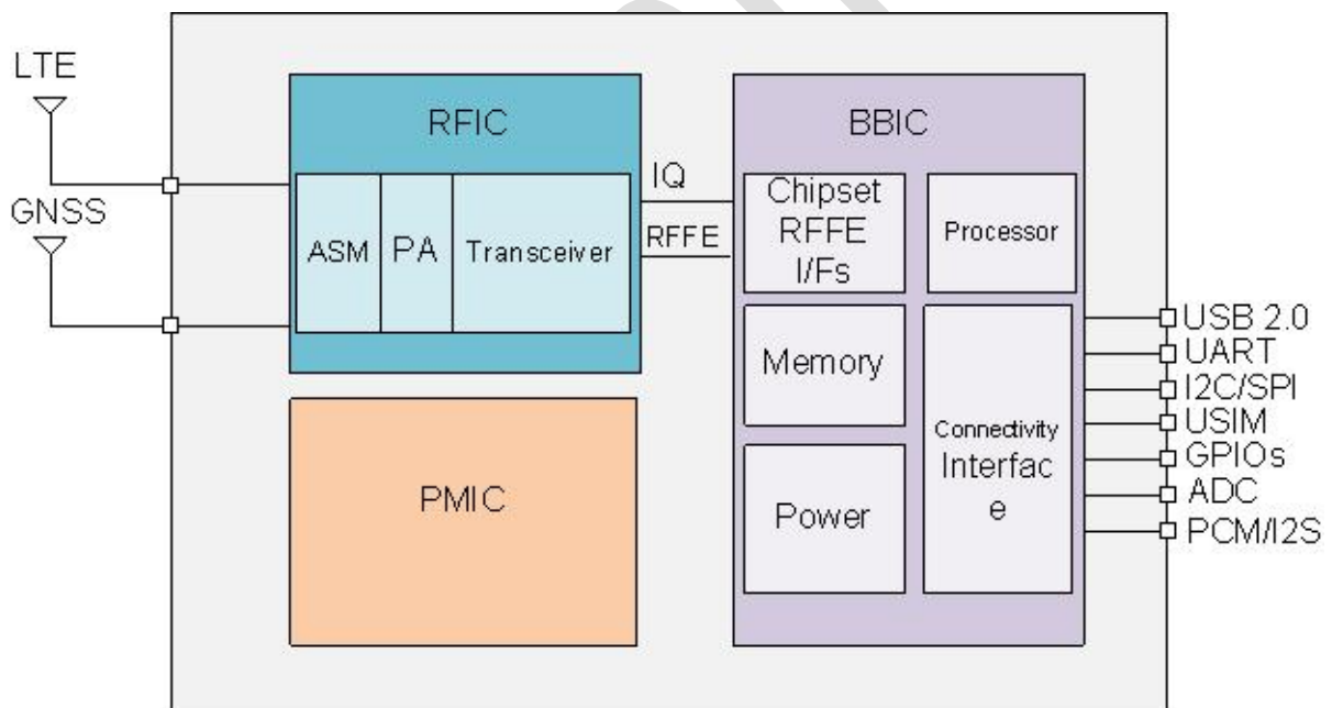
Figure 1-1. LGA function block diagram
