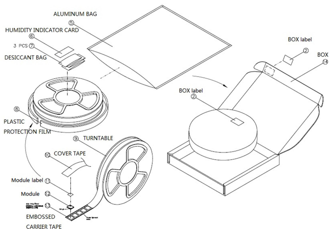
Figure 7-2. Packaging--tape
