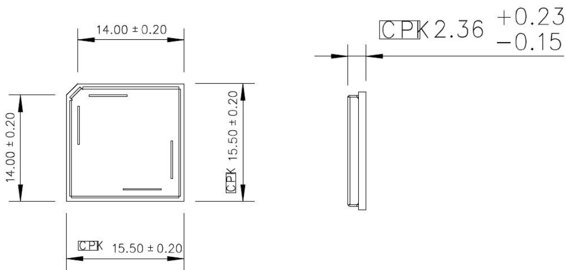
Figure 5-1. PCBA dimensions
