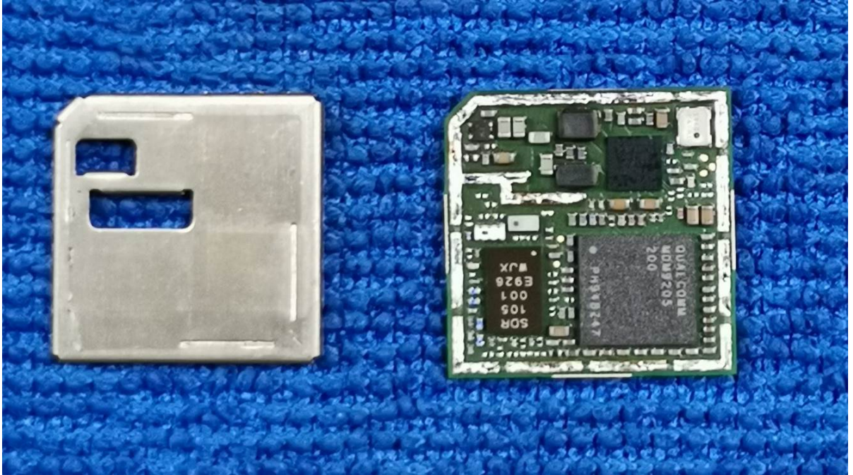
(1) EUT Photo
