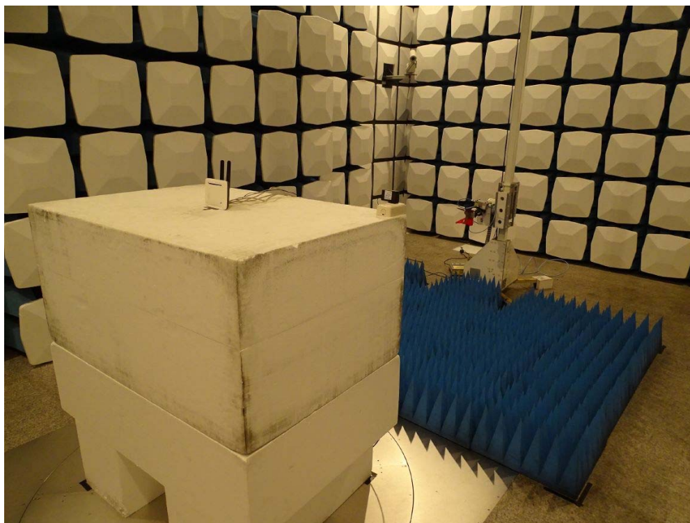
Back View of Radiated Test (Horn) (M/N:MU12AR120100-A1)
