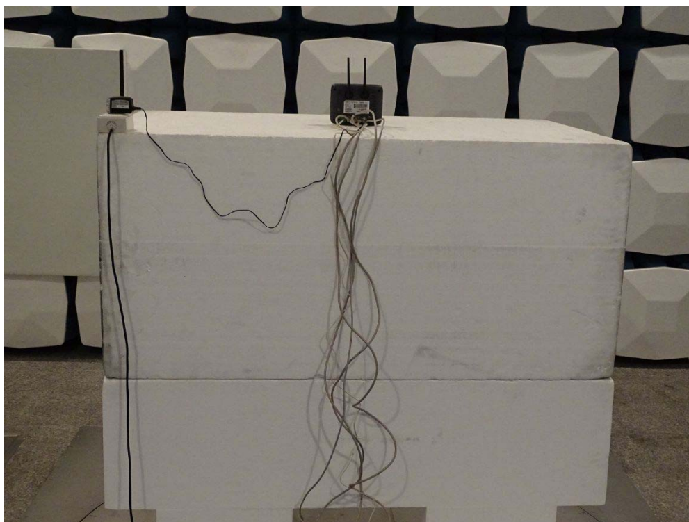
Back View of Radiated Test (Horn) (M/N:WA-12M12FU)
