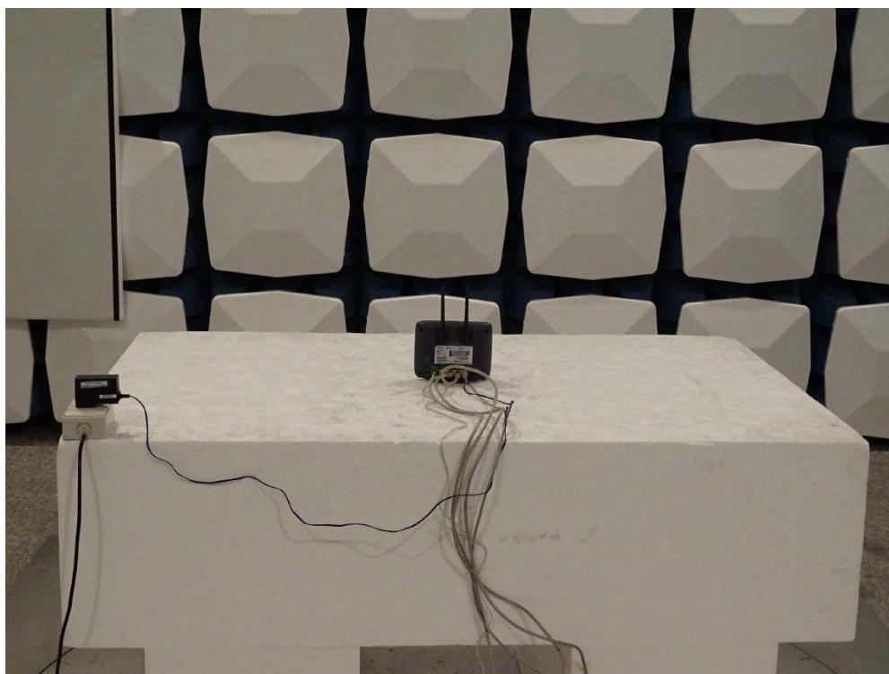
Back View of Radiated Test (M/N:MU12AR120100-A1)
