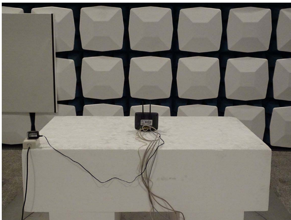
Back View of Radiated Test (M/N:WA-12M12FU)
