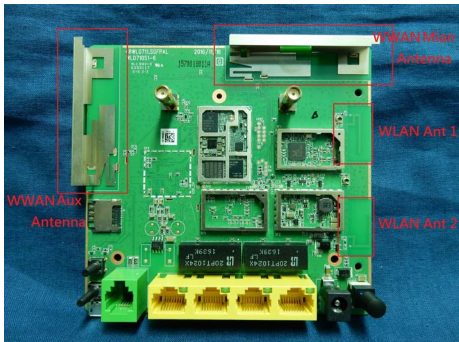
(11) EUT Photo
