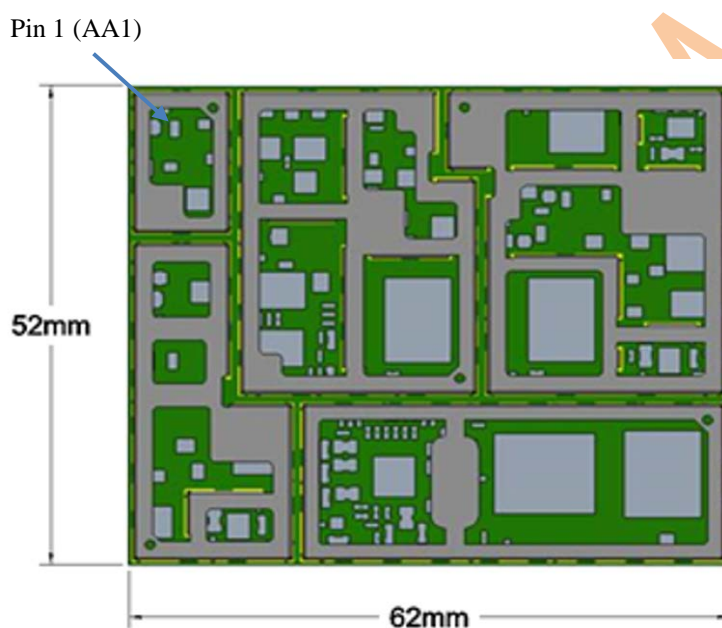
Figure 1. Top view of SA515M
