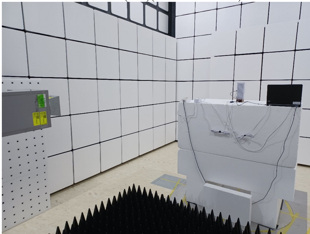
Radiated Test (Horn) (Simultaneous Transmit)
