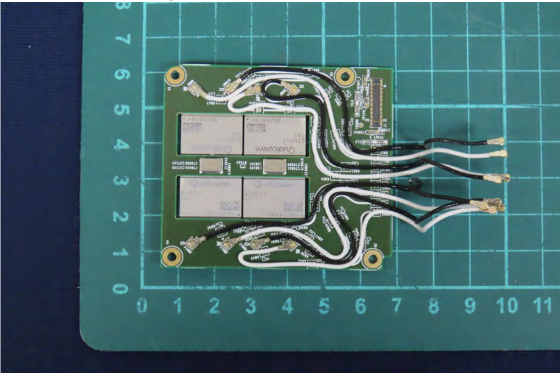
(8) EUT Photo_5G FR2 Chip
